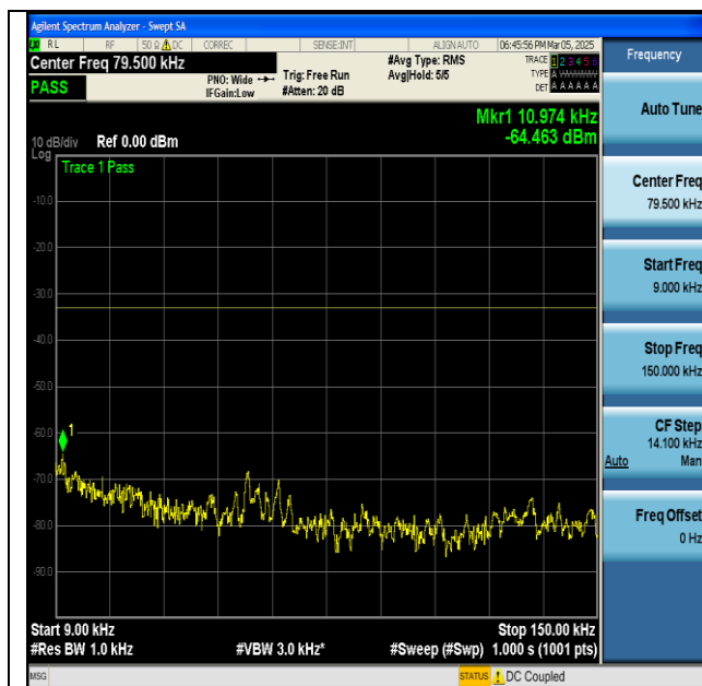
NTNV-n71-PC3-15-20-H-DFT-BPSK-Edge_1RB_Left- 0.009-0.15-PASS
