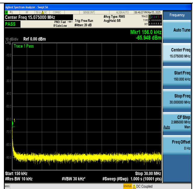
NTNV-n71-PC3-15-20-H-DFT-BPSK-Edge_1RB_Left-0.15- 30-PASS
