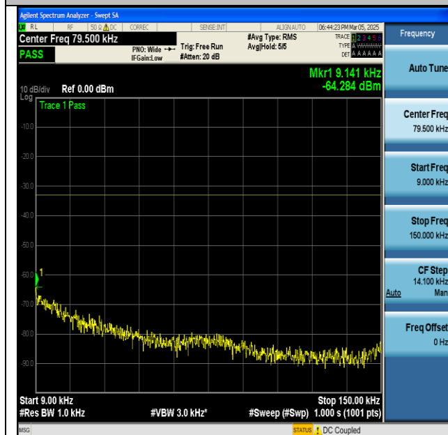
NTNV-n71-PC3-15-20-M-CP-QPSK-Edge_1RB_Left- 0.009-0.15-PASS
