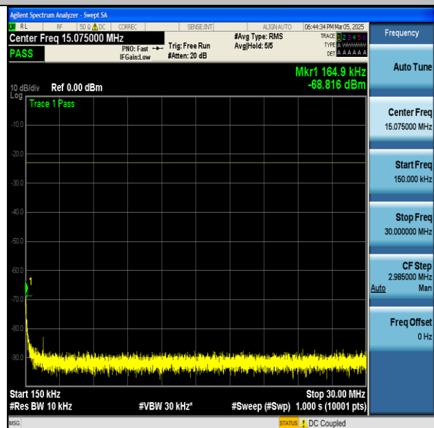
NTNV-n71-PC3-15-20-M-CP-QPSK-Edge_1RB_Left-0.15- 30-PASS
