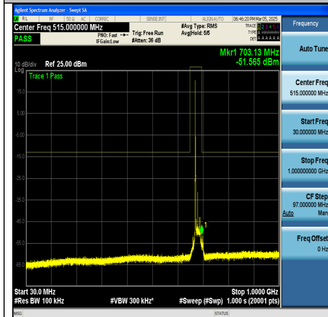
NTNV-n71-PC3-15-20-H-DFT-BPSK-Edge_1RB_Left-30- 1000-PASS
