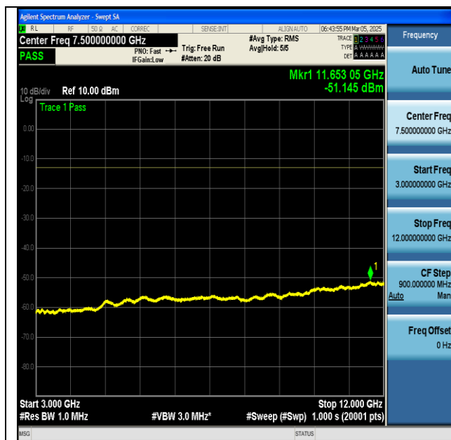
NTNV-n71-PC3-15-20-M-DFT-BPSK-Edge_1RB_Left- 3000-12000-PASS
