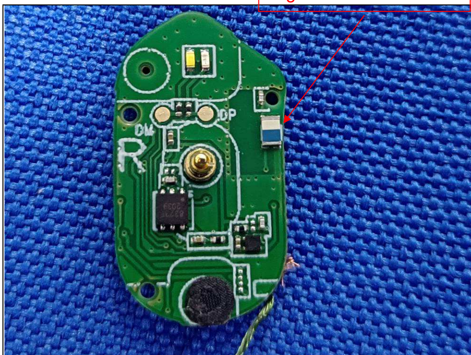
Right Earbud BT ANT.
