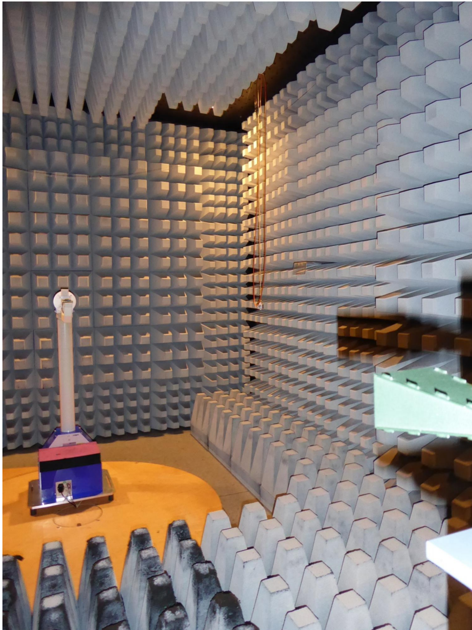
181323_SetRadC11.JPG: Test setup fully anechoic chamber; EVB-ANNA-B112C#143, 18 – 26.5 GHz
