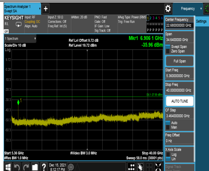
11A_Ant1_5180_5360~40000
