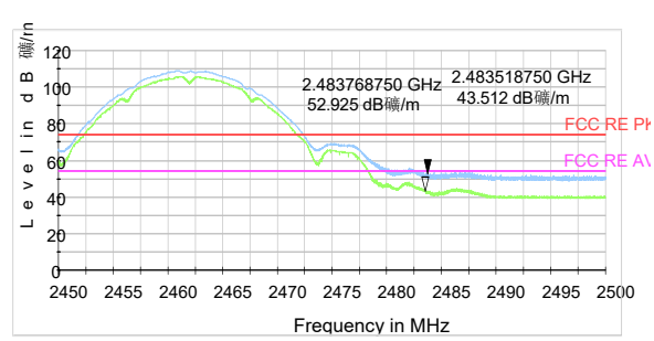
802.11b-Channel 11 Peak+ Average
