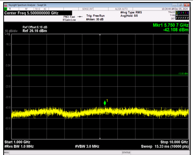
Band5-1.4MHz-64QAM-20407-1RB#0-Range2:1000~10000MHz
