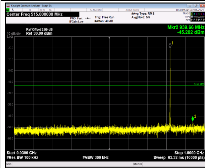
Band5-1.4MHz-16QAM-20407-1RB#0-Range1:30~10 00MHz
