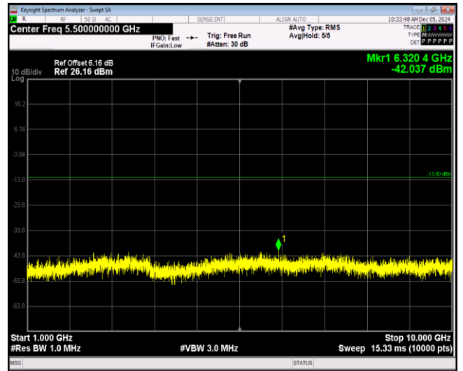
Band5-1.4MHz-16QAM-20643-1RB#0-Range2:1000~10000MHz
