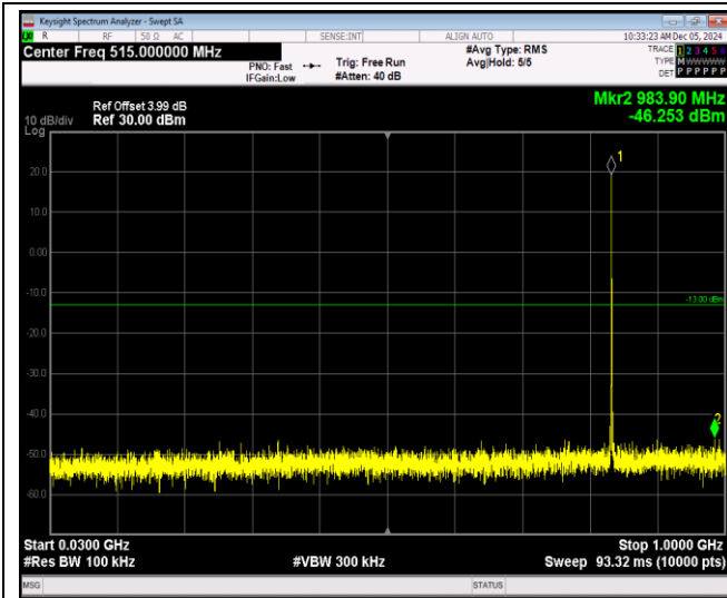
Band5-1.4MHz-QPSK-20643-1RB#0-Range1:30~100 0MHz
