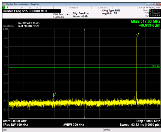
Band5-1.4MHz-64QAM-20407-1RB#0-Range1:30~1000MHz
