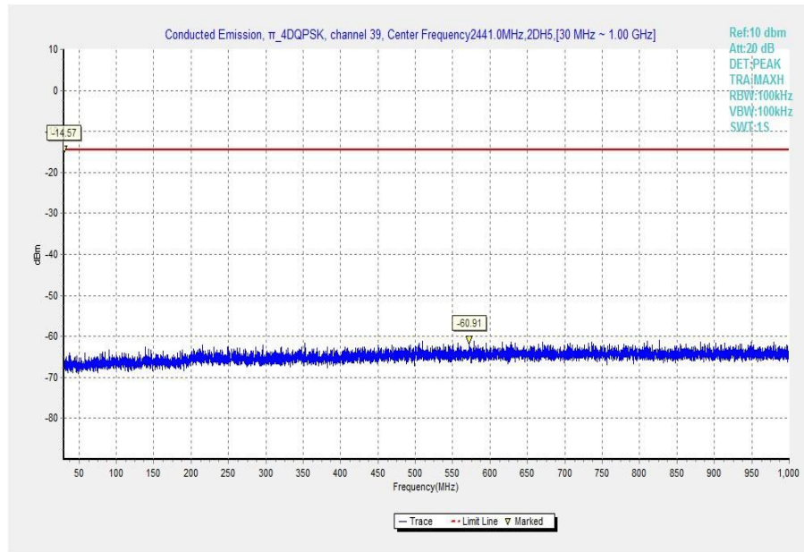
Fig. 39 Conducted Spurious Emission ( \pi /4 DQPSK, Ch39, 30 MHz-1 GHz)
