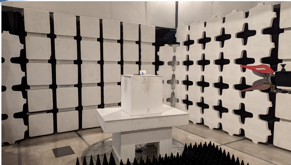
5GHz FXP831.07.0100C Tx Spurious Emissions 1-18GHz
