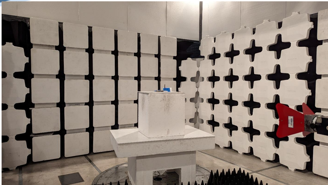
2.4GHz GW.48.A151 Tx Spurious Emissions 1-18GHz
