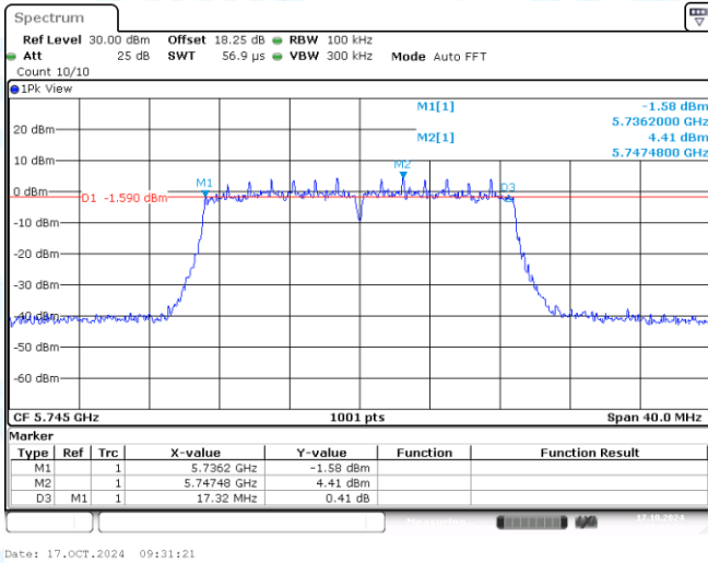
11N20MIMO-Ant1-5745-PASS
