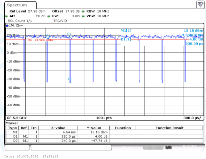
NTNV-11A-CDD-Ant2-5200
