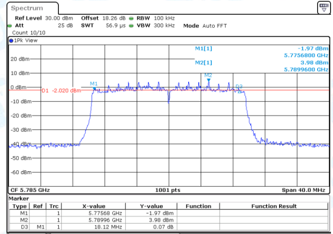
11AX20MIMO-Ant2-5785-PASS
