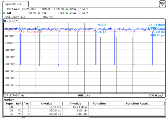
NTNV-11A-CDD-Ant2-5745
