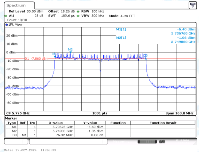
11AC80MIMO-Ant2-5775-PASS
