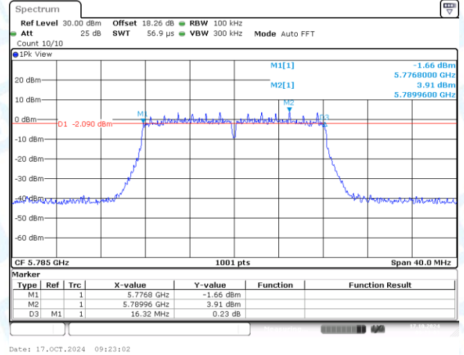
11A-CDD-Ant2-5785-PASS
