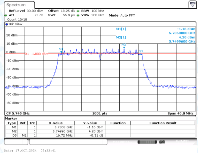
11N20MIMO-Ant2-5745-PASS
