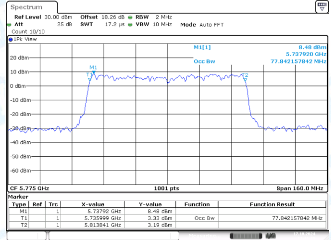
11AX80MIMO-Ant2-5775
