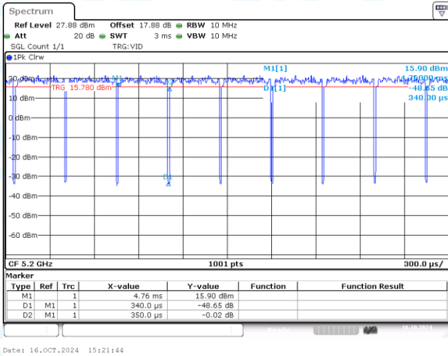
NTNV-11A-CDD-Ant1-5200
