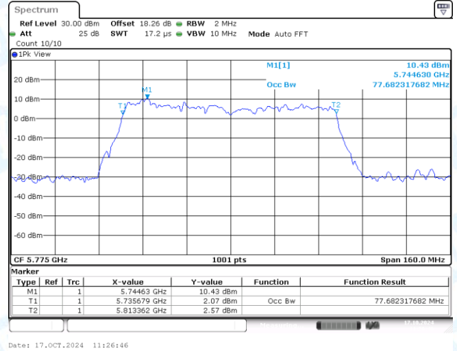
11AC80MIMO-Ant2-5775
