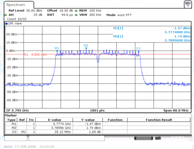
11AC40MIMO-Ant2-5795-PASS
