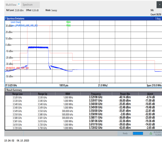
1-N48-PC3-30-30-L-3-DFT-PI2BPSK-Outer_Full -75@0-Ant2-1--PASS-see graph
