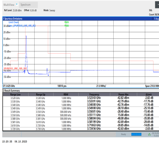
1-N48-PC3-30-30-L-1-DFT-PI2BPSK-Edge_1RB_Le ft_1@0-Ant2-1--PASS-see graph
