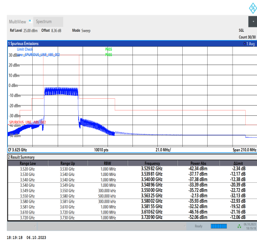
1-N48-PC3-30-30-L-6-CP-QPSK-Outer_Full-78 @0-Ant2-1--PASS-see graph
