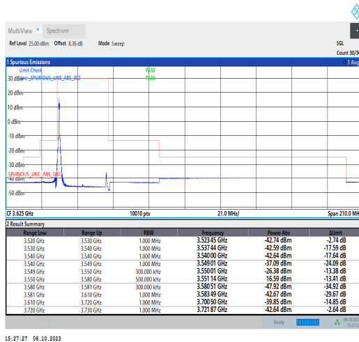
1-N48-PC3-30-30-L-4-CP-QPSK-Edge_1RB_Left-1 @0-Ant2-1--PASS-see graph
