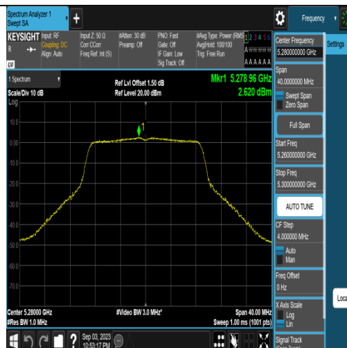
11N20SISO-Ant1-5280
