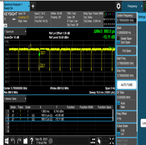
NTNV-11AC40SISO-Ant1-5795
