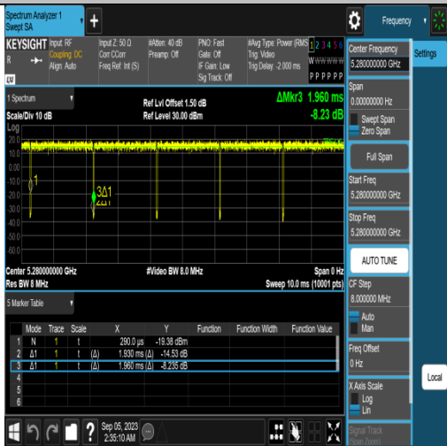
NTNV-11AC20SISO-Ant1-5280
