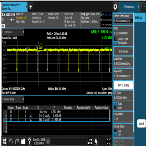
NTNV-11AC40SISO-Ant1-5510
