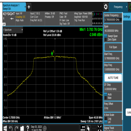
11N20SISO-Ant1-5785
