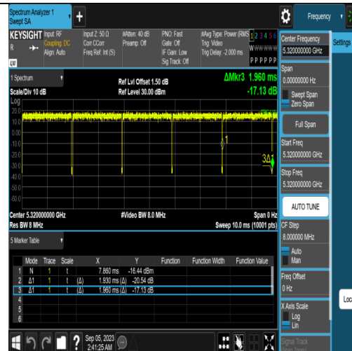
NTNV-11AC20SISO-Ant1-5320
