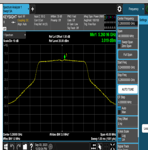
11N20SISO-Ant1-5260
