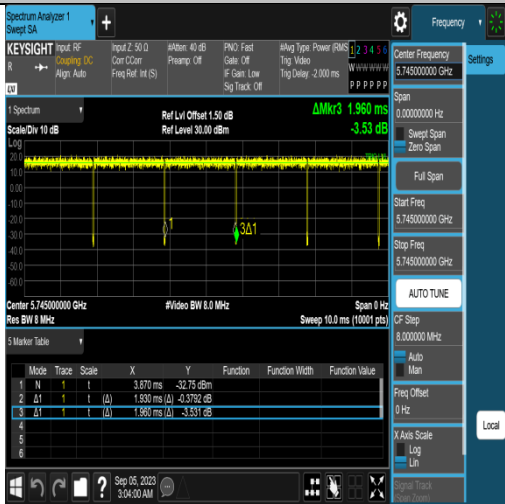
NTNV-11AC20SISO-Ant1-5745
