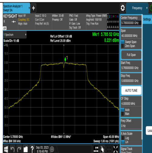
11A-Ant1-5785
