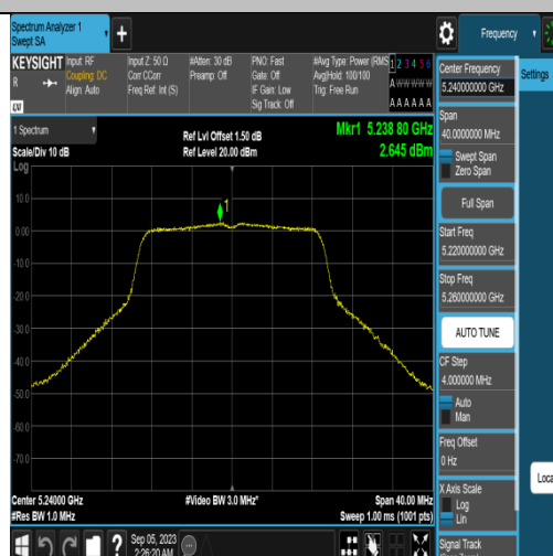
11AC20SISO-Ant1-5240
