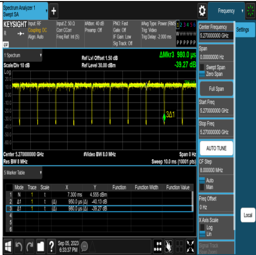
NTNV-11AC40SISO-Ant1-5270
