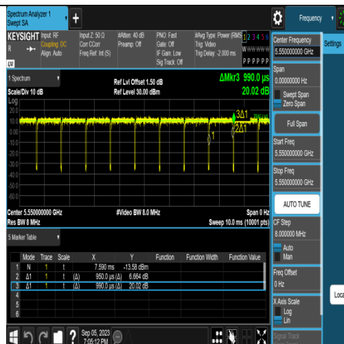
NTNV-11AC40SISO-Ant1-5550
