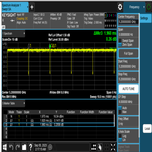
NTNV-11AC20SISO-Ant1-5200
