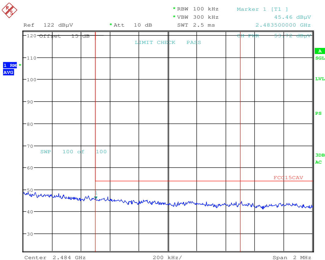
Plot 7-19. Radiated Restricted Upper Band Edge Measurement (Average)
