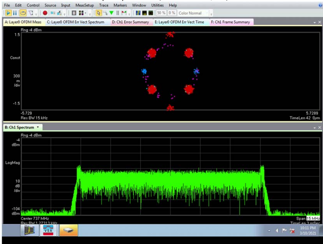
Channel Frequency 737 MHz, Modulation QPSK, 10 MHz BW
