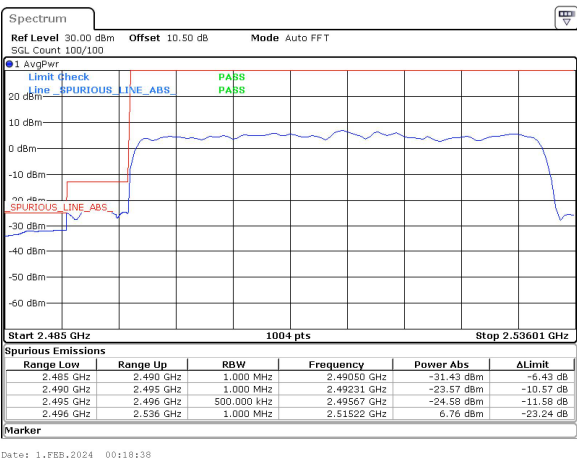
40MHz_30kHz_2516.01MHz_DFT-s-OFDM QPSK_RB100@0&-31.43 dBm
