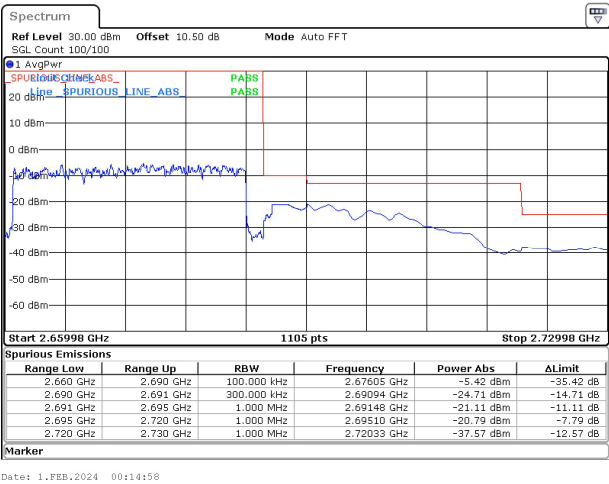
30MHz_30kHz_2674.98MHz_DFT-s-OFDM QPSK_RB75@0&-20.79 dBm
