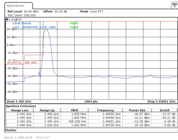
40MHz_30kHz_2516.01MHz_DFT-s-OFDM QPSK_RB1@0&-13.38 dBm
