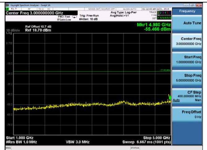
CUE-802.11n-20-5280M -chain3(1GHz-5GHz)
