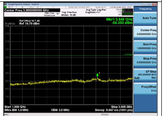
CUE-802.11a-5260M-chain3(1GHz-5GHz)
