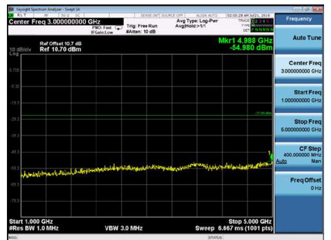
CUE-802.11n-20-5280M-chain4(1GHz-5GHz)
