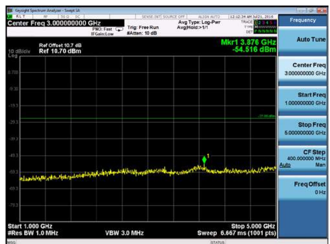
CUE-802.11a-5260M-chain2(1GHz-5GHz)
