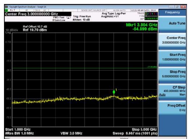
CUE-802.11n-20-5260M-chain2(1GHz-5GHz)
