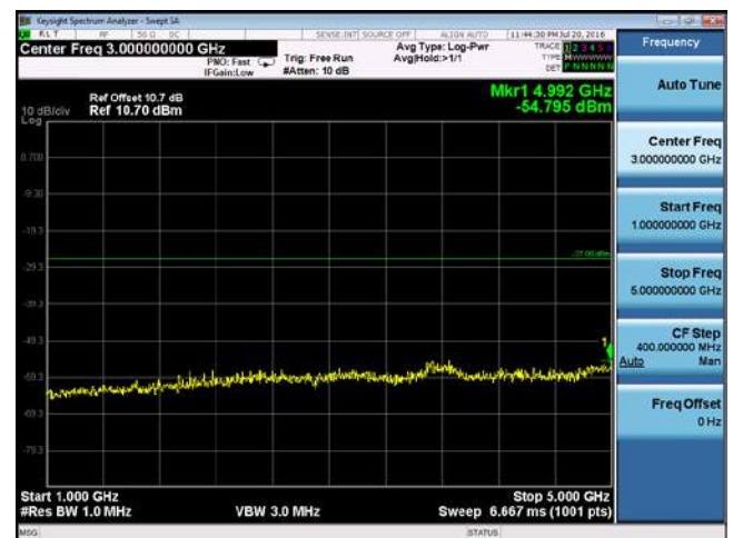
CUE-802.11n-20-5280M-chain1(1GHz-5GHz)
