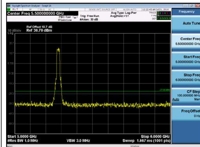
CUE-802.11n-20-5280M -chain2(5GHz-6GHz)
