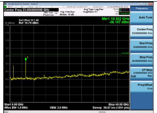
CUE-802.11n-20-5260M-chain1(6GHz-40GHz)
