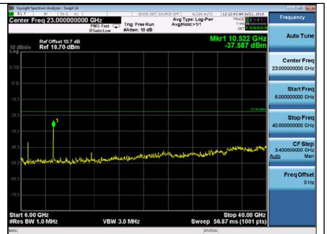
CUE-802.11a-5260M-chain2(6GHz-40GHz)
