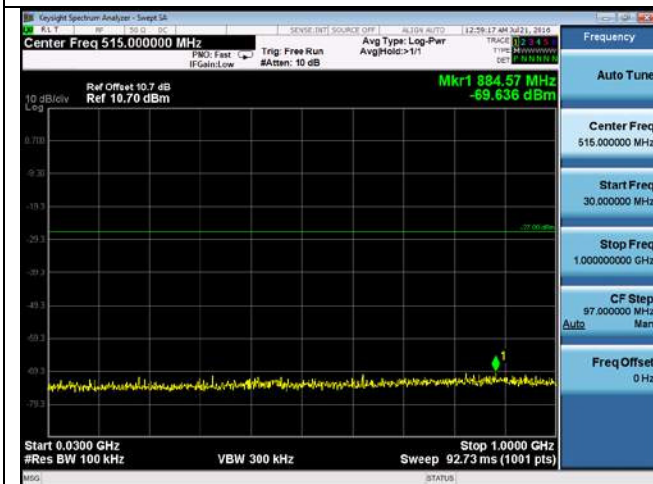
CUE-802.11a-5260M-chain3(30MHz-1GHz)
