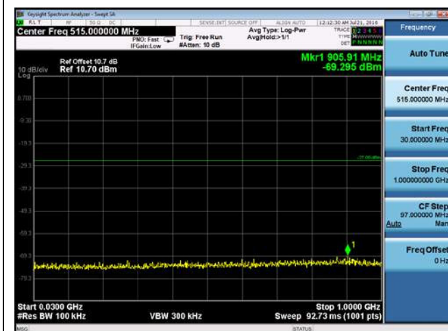
CUE-802.11a-5260M-chain2(30MHz-1GHz)
