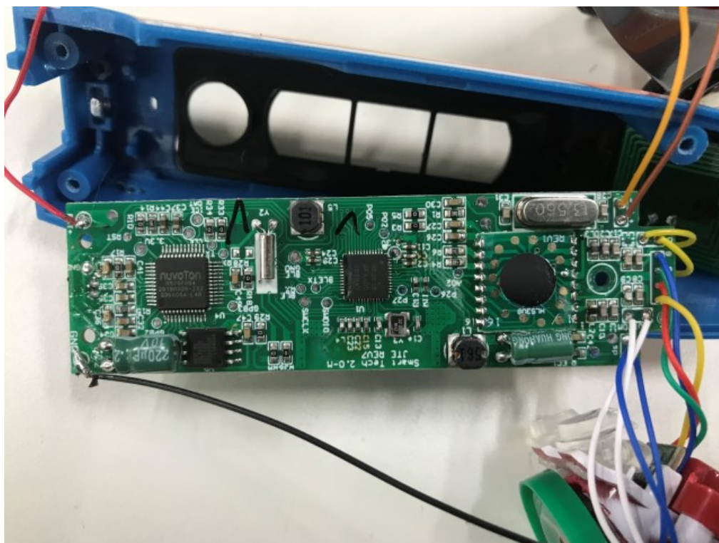
Internal View (Model: 3971)
