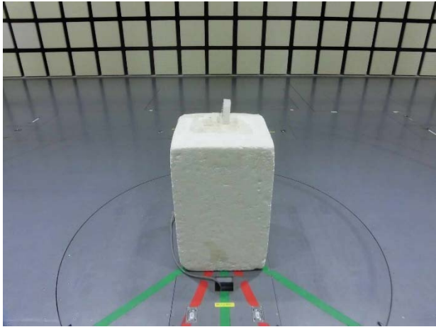
Below 1 GHz
