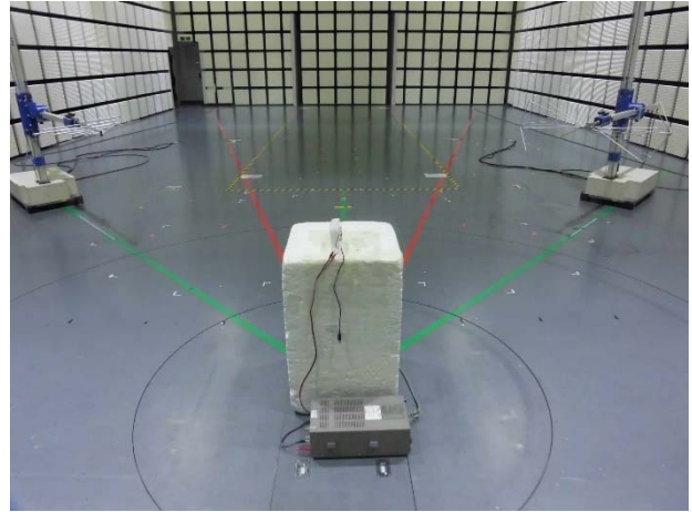
Below 1 GHz
