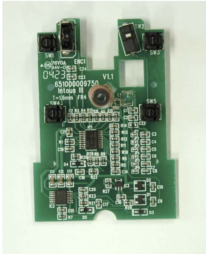
Photo11 Mouse (model: ZC-100)
