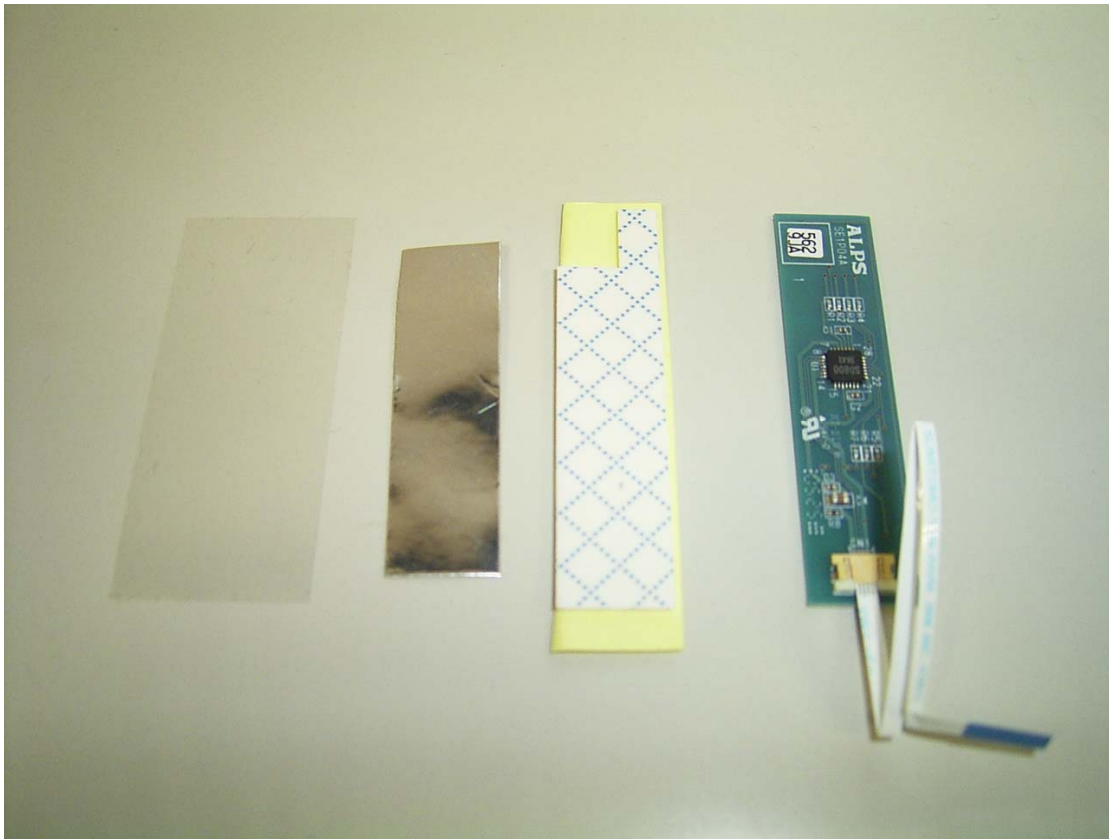
Photo 5 Touch pad view
