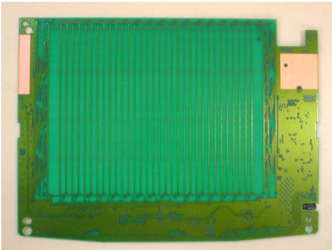
Photo 4 Reverse of Main board
