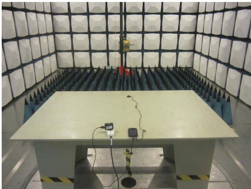
Radiated Emission Above 1GHz- Rear View (Operating & Charging)
