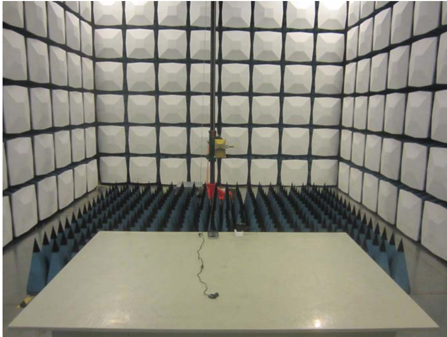
Radiated Emission Above 1GHz -Front View (Operating & Charging)
