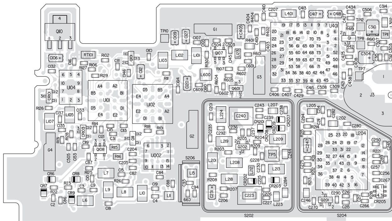
BOTTOM VIEW
