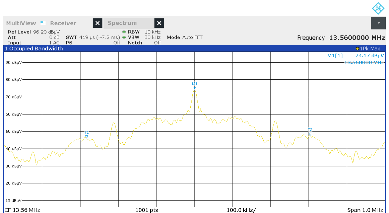
Figure 11: Chart of occupied bandwidth test, with tag
