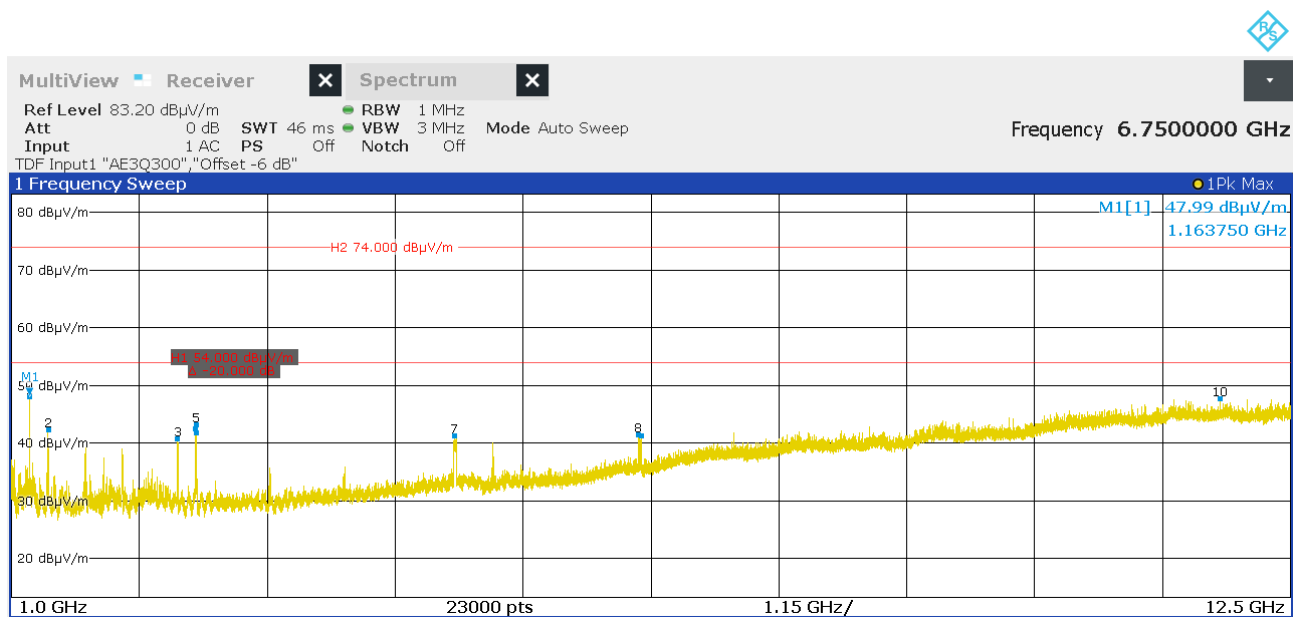
Figure 15: Chart of emissions test from 1 GHz to 12.5 GHz, EUT position Y, antenna polarization vertical, with tag
