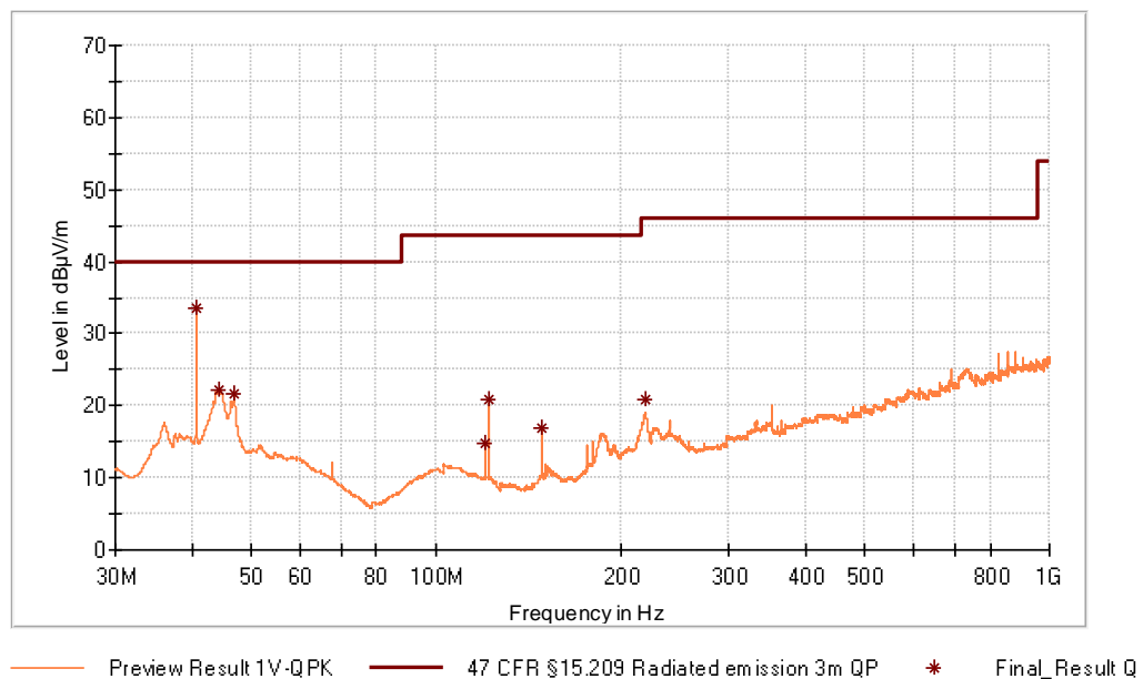
Figure 14: Chart of radiated emissions test from 30 MHz to 1 GHz, EUT position Z, antenna polarization vertical, without tag
