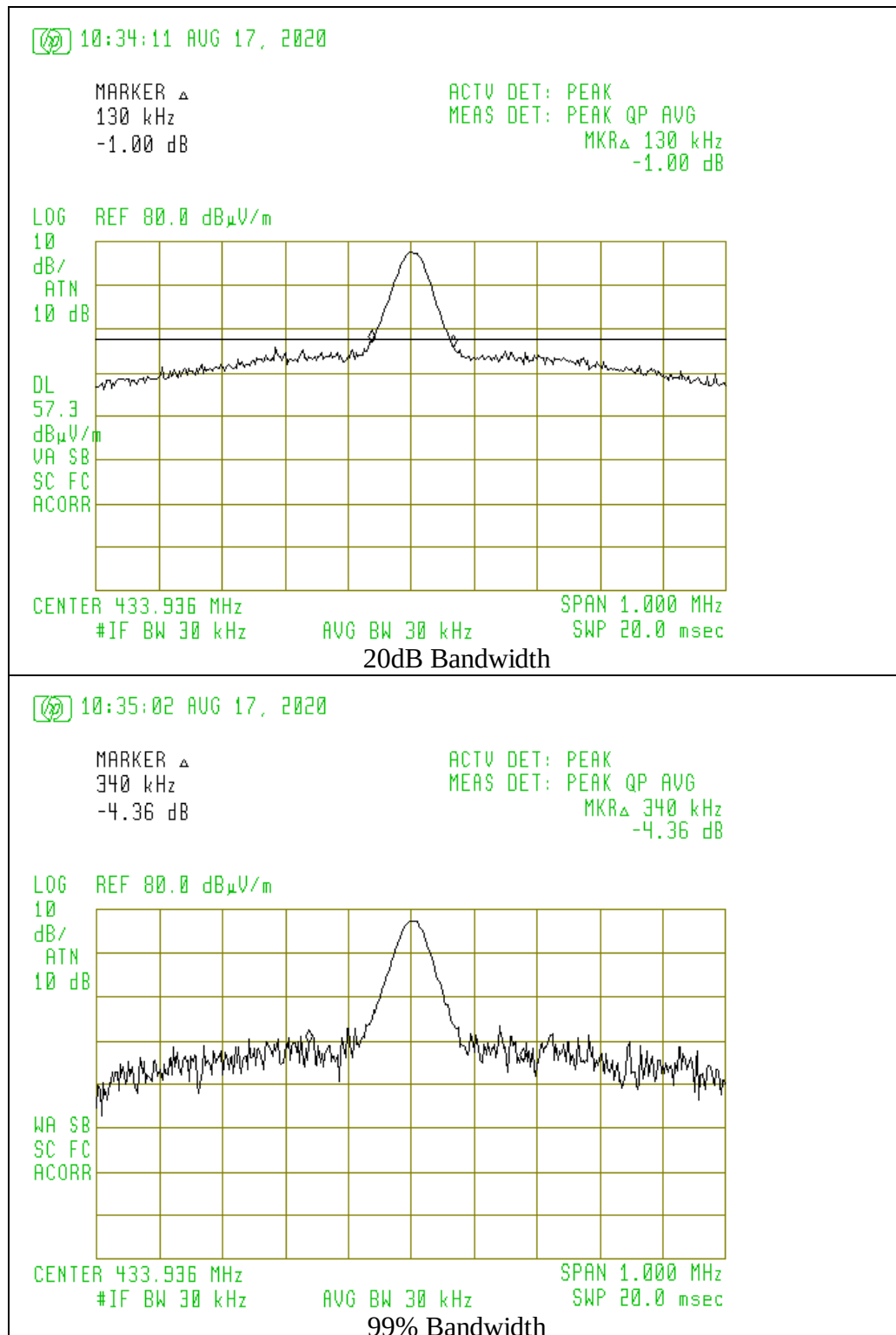
Figure 6.1 Occupied Bandwidth
