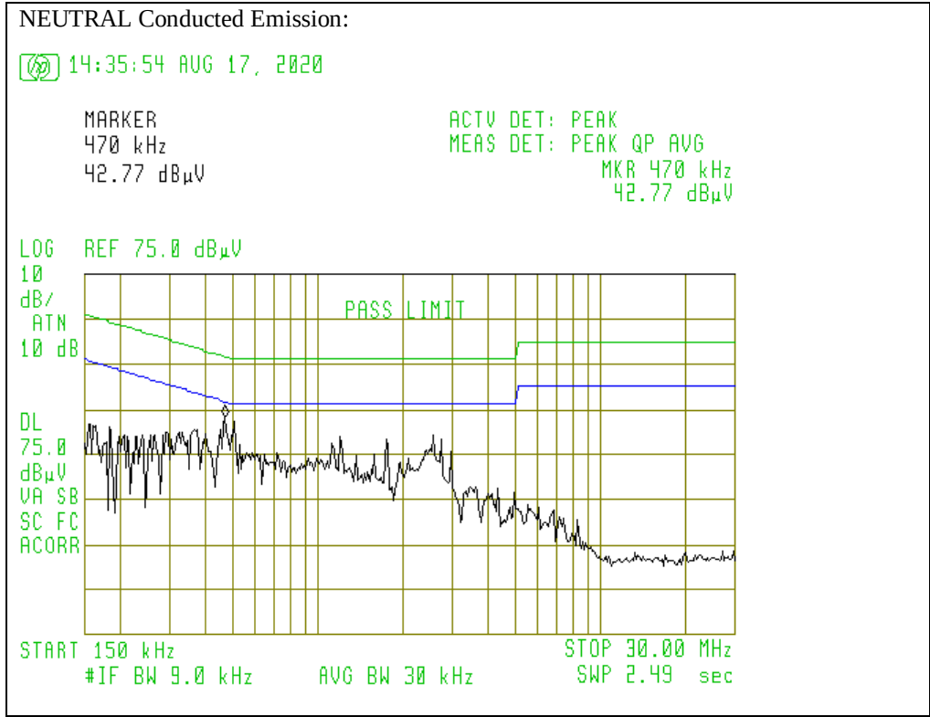
Figure 5.2 NEUTRAL Conducted Emission
