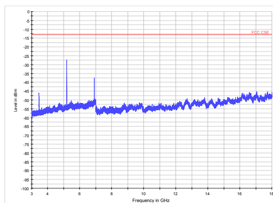
LTE Band 4 5MHz CH-High 3GHz~18GHz
