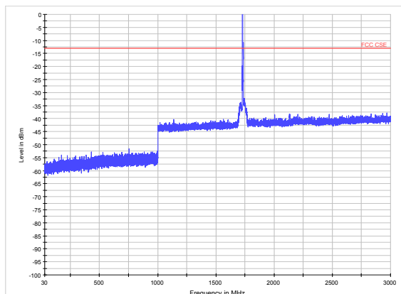
LTE Band 4 5MHz CH-High 30MHz~3GHz
