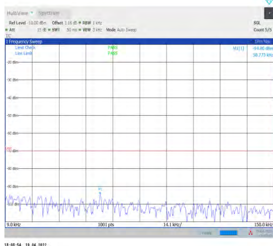
1-N30--15-10-M-1-DFT-PI2BPSK-Inner_1RB_Left-1 @1-0.009-0.15-Ant1--94.80--70-PASS
