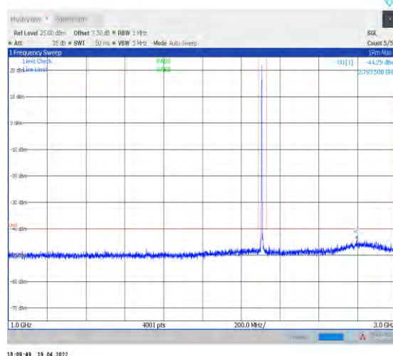
1-N30--15-10-H-1-DFT-PI2BPSK-Inner_1RB_Left-1 @1-1000-3000-Ant1--44.29--40-PASS
