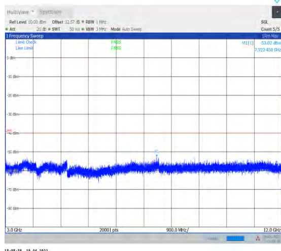
1-N30--30-15-L-1-DFT-PI2BPSK-Inner_1RB_Left-1 @1-3000-12000-Ant1--53.02--40-PASS
