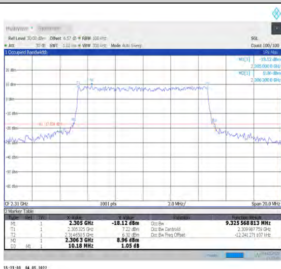
1-N30--15-10-H-6-CP-QPSK-Outer_Full-52@0-Ant1- 9.326-10.180-≤10-PASS
