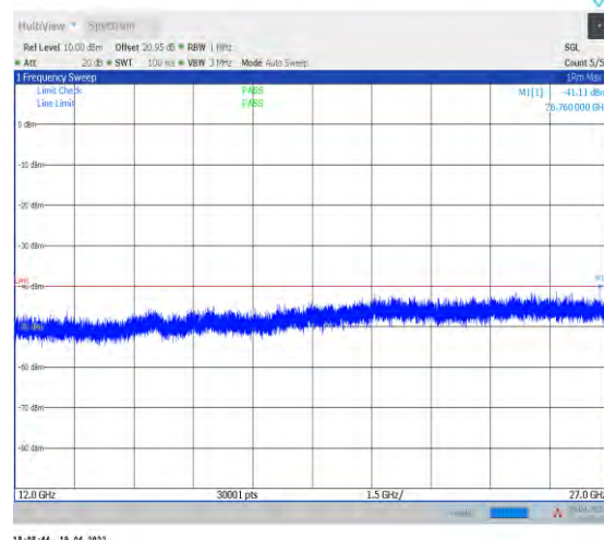
1-N30--15-10-L-1-DFT-PI2BPSK-Inner_1RB_Left-1@ 1-12000-27000-Ant1--41.11--40-PASS
