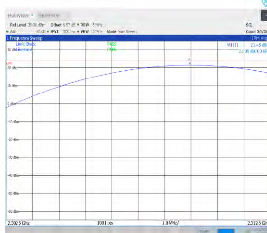
1-N30-PC3-15-5-L-2-DFT-PI2BPSK-Inner_1RB_Right -1@23-2302.5-2312.5-Ant1-21.45-23.98-PASS
