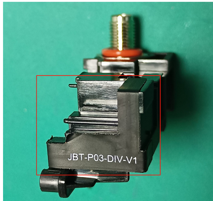
BT/Wi-Fi ANT
