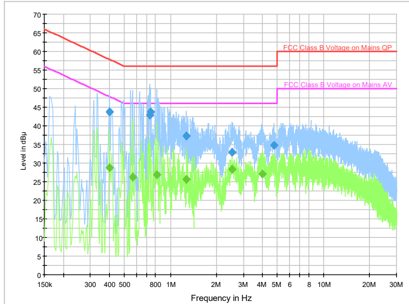
Fig. 26 AC Powerline Conducted Emission-Ide
