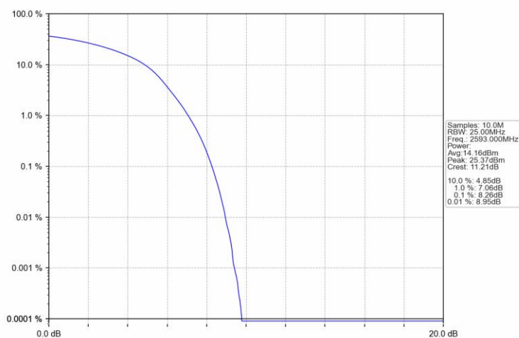
Band41_15MHz_16QAM_MCH_2593MHz_RB_75_0_NTNV
