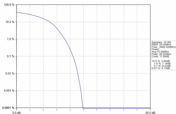
Band41_15MHz_16QAM_HCH_2682.5MHz_RB_75_0_NTNV
