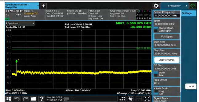
Band66-20MHz-QPSK-132572-1RB#99-3000~20000-PASS
