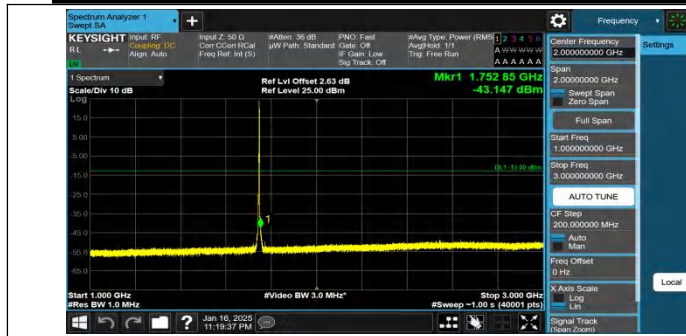
Band66-3MHz-QPSK-132322-1RB#14-1000~3000-PASS
