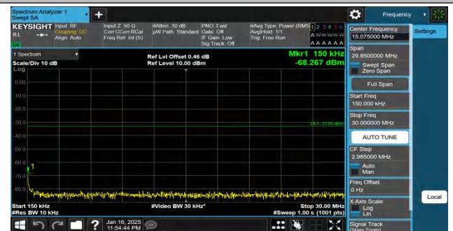
Band66-20MHz-QPSK-132072-1RB#0-0.15~30-PASS
