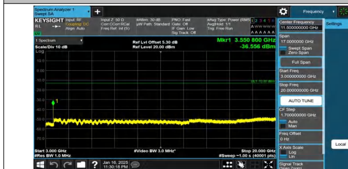
Band66-5MHz-QPSK-132647-1RB#0-3000~20000-PASS
