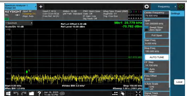
Band66-15MHz-QPSK-132322-1RB#74-0.009~0.15-PASS
