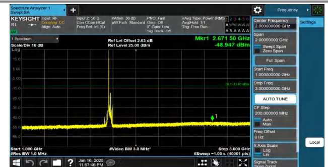
Band66-20MHz-QPSK-132572-1RB#0-1000~3000-PASS
