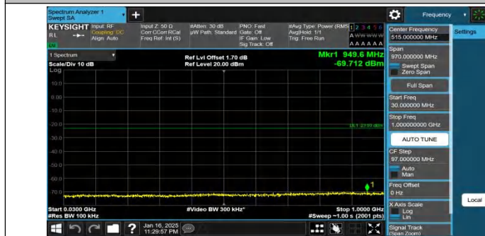
Band66-5MHz-QPSK-132647-1RB#0-30~1000-PASS
