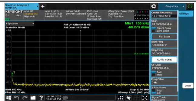
Band66-15MHz-QPSK-132322-1RB#0-0.15~30-PASS
