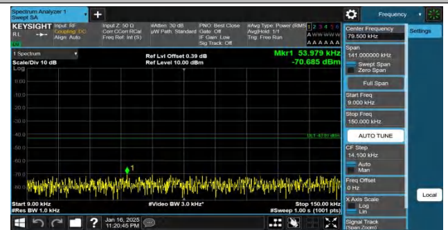
Band66-3MHz-QPSK-132657-1RB#14-0.009~0.15-PASS
