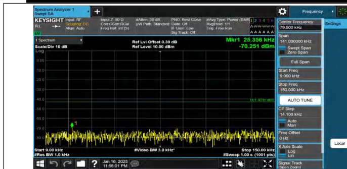
Band66-20MHz-QPSK-132322-1RB#0-0.009~0.15-PASS
