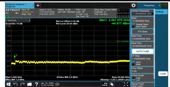
Band66-20MHz-QPSK-132322-1RB#99-3000~20000-PASS
