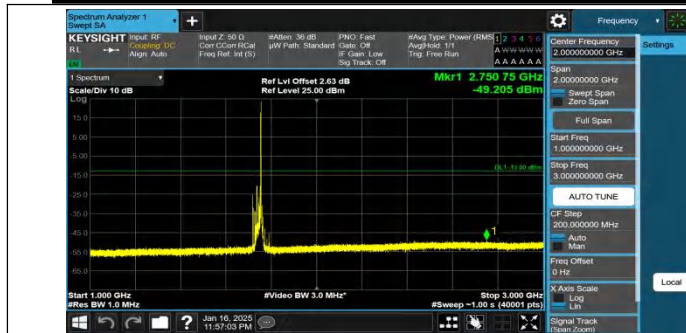
Band66-20MHz-QPSK-132322-1RB#99-1000~3000-PASS
