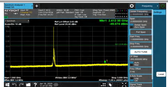
Band66-15MHz-QPSK-132322-1RB#0-1000~3000-PASS
