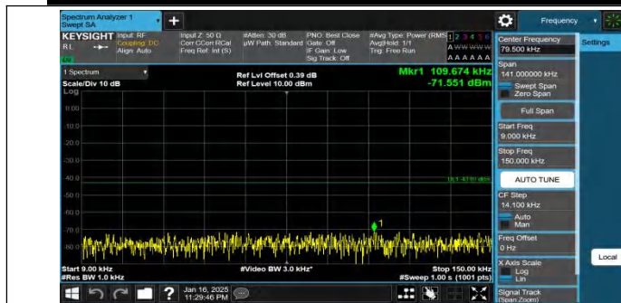
Band66-5MHz-QPSK-132647-1RB#0-0.009~0.15-PASS
