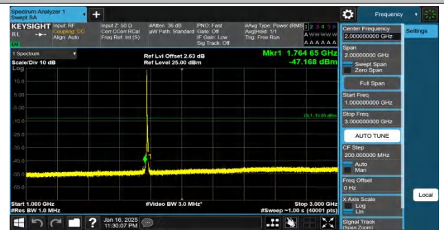
Band66-5MHz-QPSK-132647-1RB#0-1000~3000-PASS
