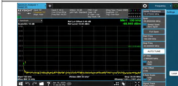
Band66-5MHz-QPSK-132647-1RB#24-0.15~30-PASS
