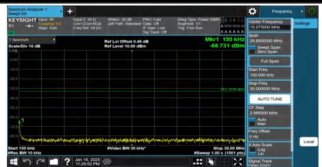
Band66-5MHz-QPSK-132647-1RB#0-0.15~30-PASS
