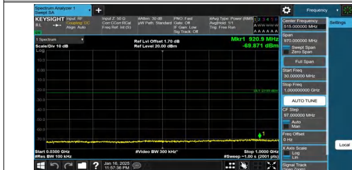
Band66-20MHz-QPSK-132572-1RB#0-30~1000-PASS
