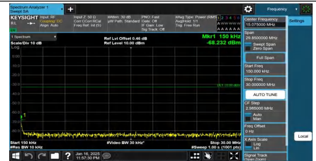
Band66-20MHz-QPSK-132572-1RB#0-0.15~30-PASS
