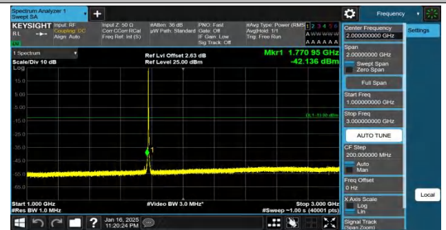
Band66-3MHz-QPSK-132657-1RB#0-1000~3000-PASS
