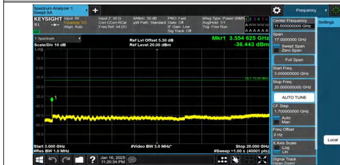
Band66-3MHz-QPSK-132657-1RB#0-3000~20000-PASS
