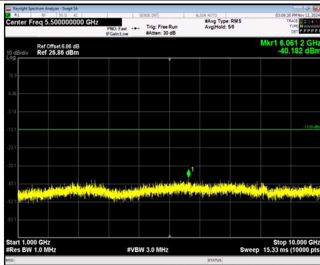
Band17-5MHz-64QAM-23755-1RB#0-Range2:1000~10000MHz
