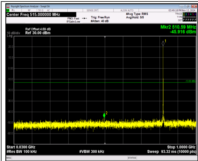
Band26-1.4MHz-16QAM-26915-1RB#0-Range1:30~1000MHz
