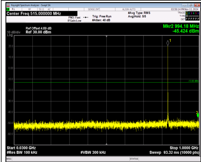
Band26-1.4MHz-16QAM-27033-1RB#0-Range1:30~1000MHz
