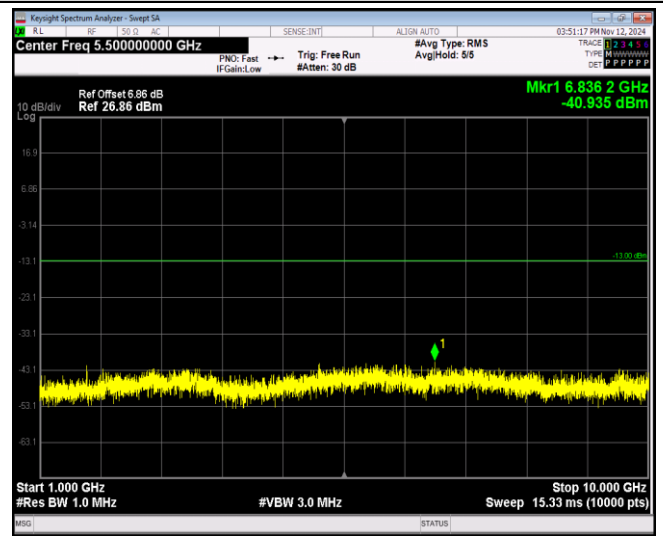
Band26-1.4MHz-16QAM-27033-1RB#0-Range2:1000~10000MHz
