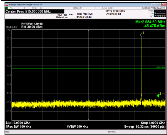
Band26-1.4MHz-16QAM-27033-1RB#0-Range1:30~1000MHz
