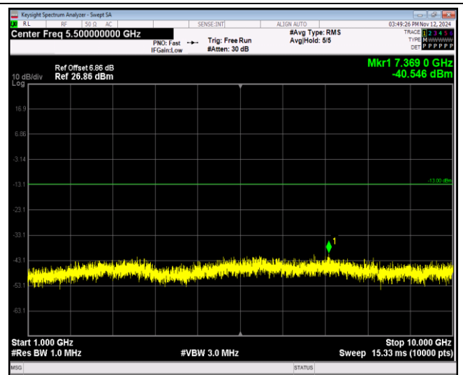
Band26-1.4MHz-16QAM-26915-1RB#0-Range2:1000~10000MHz
