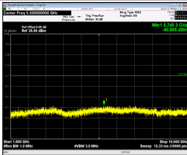
Band17-10MHz-QPSK-23800-1RB#0-Range2:1000~10000MHz
