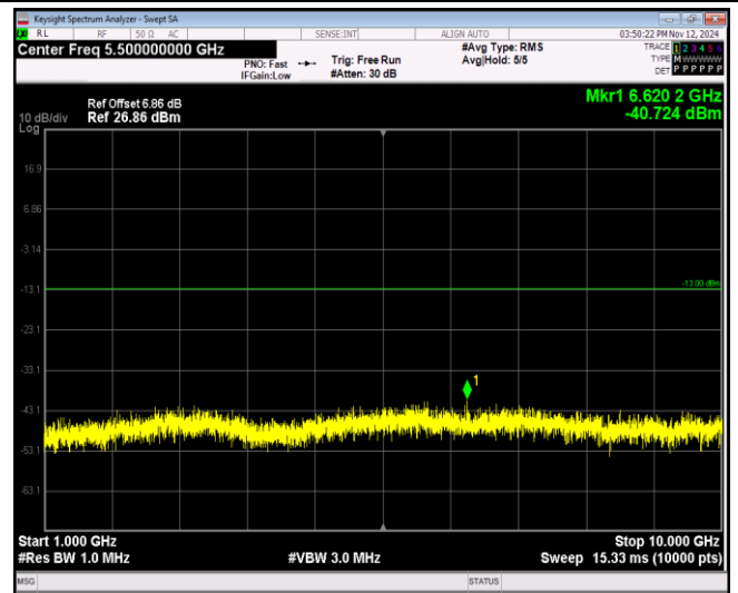
Band26-1.4MHz-16QAM-27033-1RB#0-Range2:1000~10000MHz
