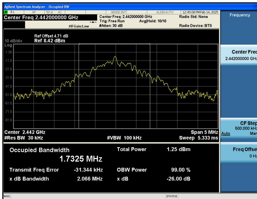
99%_Occupied_Bandwidth_NVNT_ANT1_2.4G_2442_00
