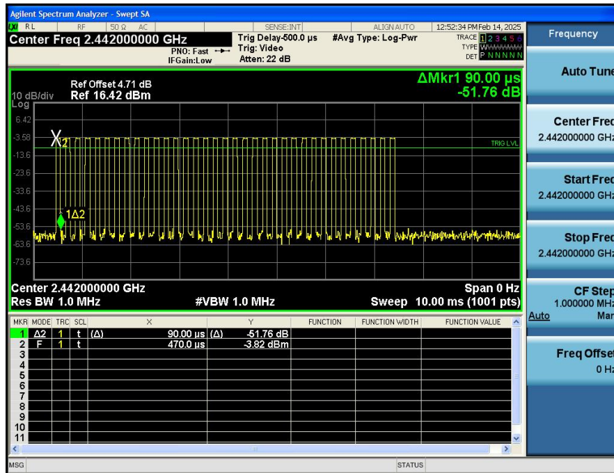
Dwell_Time_(Hopping)_NVNT_ANT1_2.4G_2442_00_Accumulated
