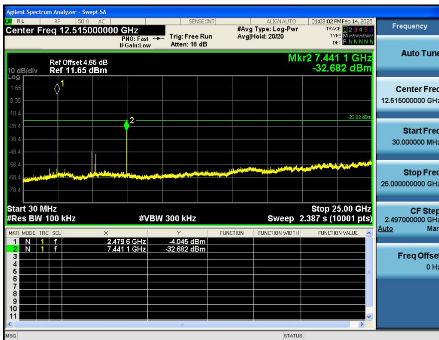
2_Spurious_Emissions_NVNT_ANT1_2.4G_2480_00
