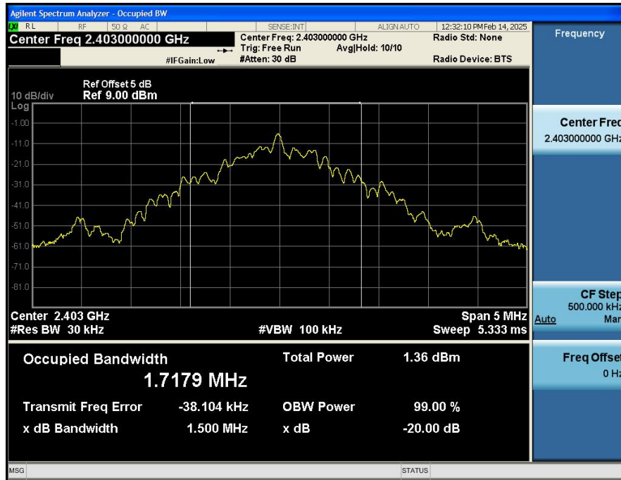
-20dB_Bandwidth_NVNT_ANT1_2.4G_2403_00
