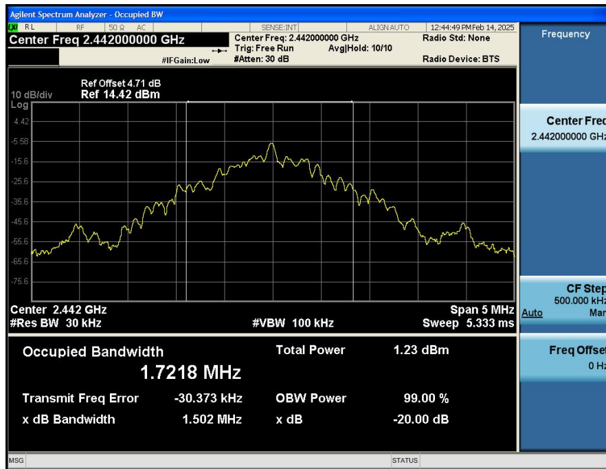
-20dB_Bandwidth_NVNT_ANT1_2.4G_2442_00
