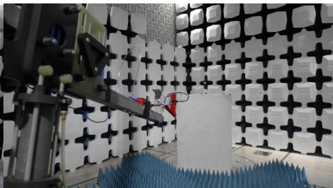
Figure 2: QLXD2 Transmitter Test Setup
