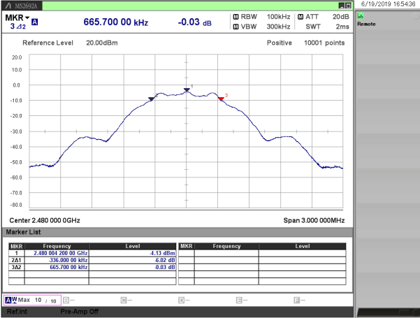
[1 Mbps / 2480 MHz]
