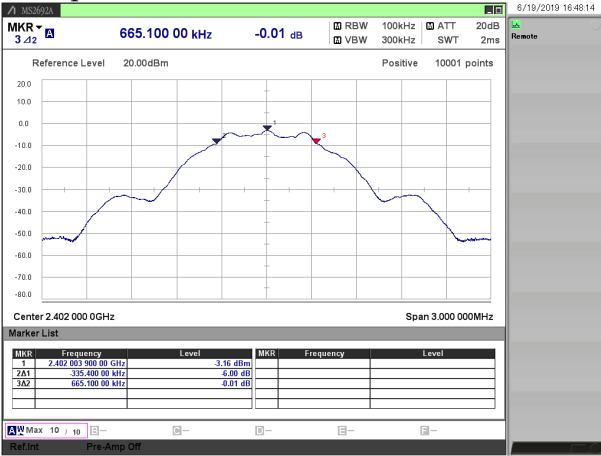
[1 Mbps / 2402 MHz]
