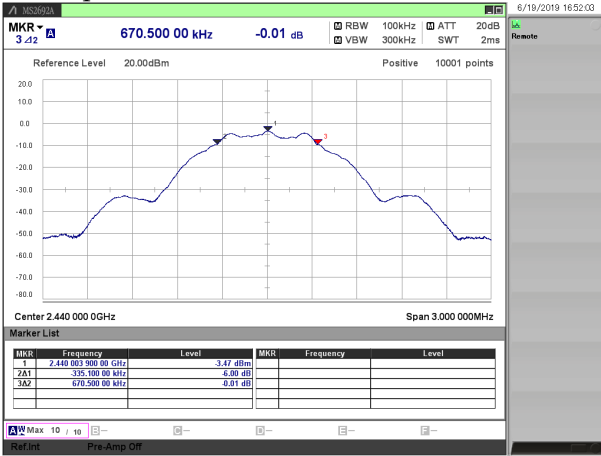
[1 Mbps / 2440 MHz]
