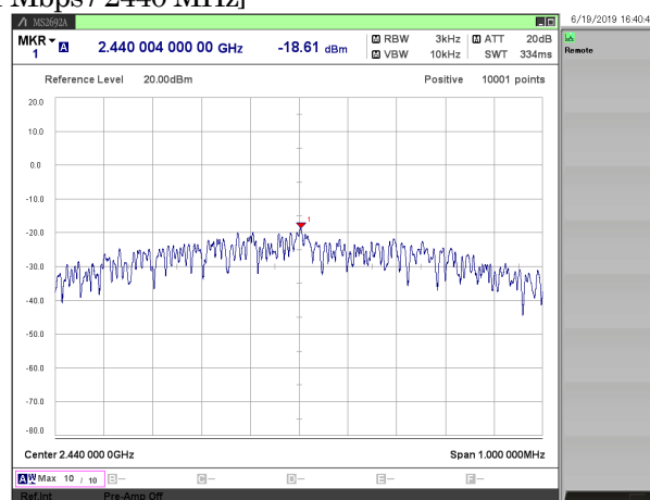
[1 Mbps / 2440 MHz]
