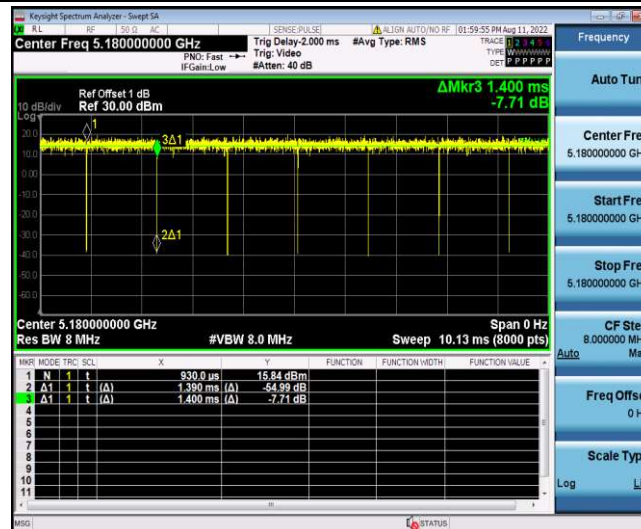
11A_Ant2_5180
