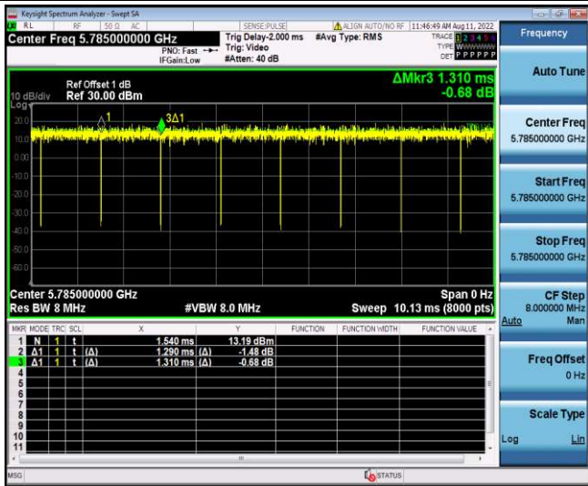
11N20SISO_Ant1_5785
