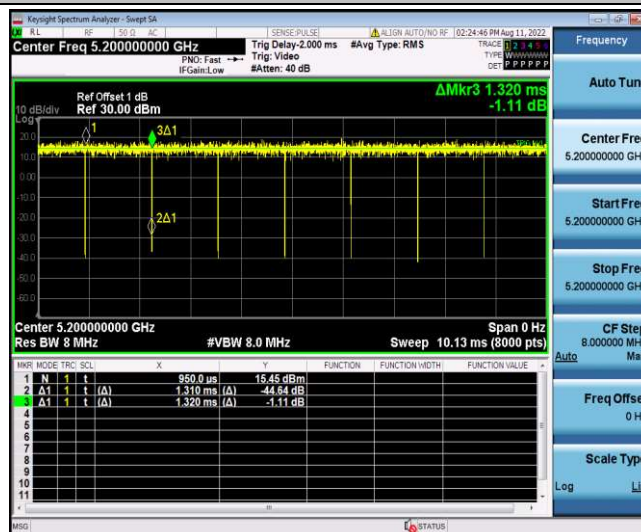
11AC20SISO_Ant2_5200
