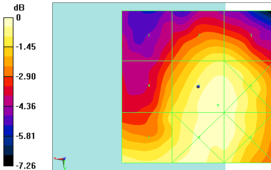
Fig B.3 HAC RF E-Field LTE Band41 Power Class 2 QPSK CH40620
