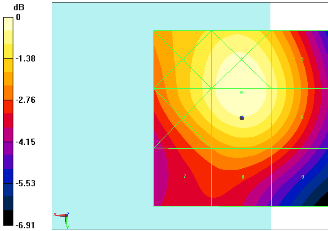
Fig B.4 HAC RF E-Field WiFi2.4G 11g
