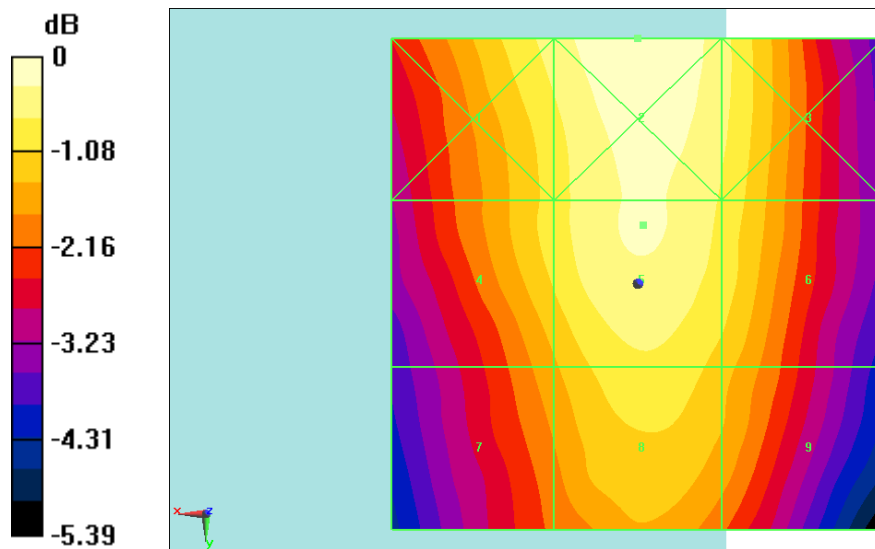
Fig B.1 HAC RF E-Field GSM 850 Middle
