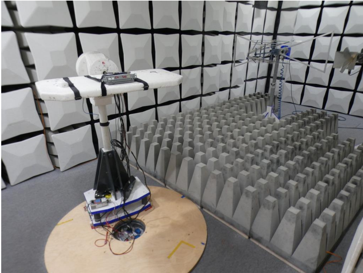
Photo 3: Test setup for radiated measurements (stand alone setup, 1 GHz – 24 GHz; FCC 15c247)
