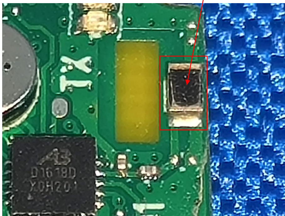
Chip Antenna
