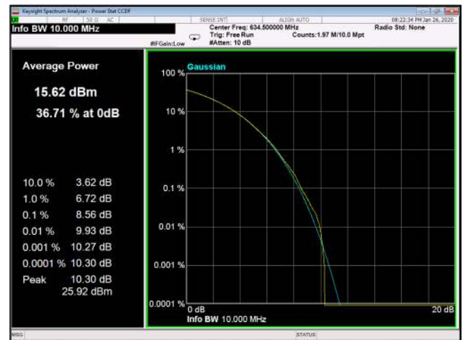
Figure 234: 16QAM 10MHz B.W; 634.5MHz, 15kHz
