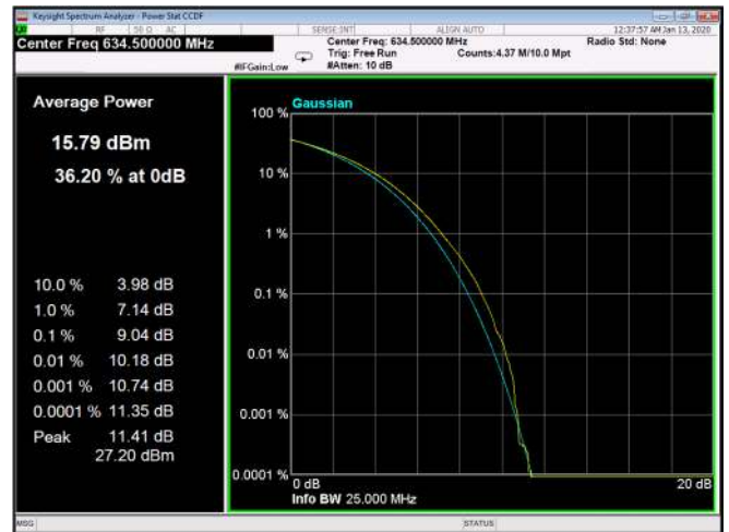
Figure 287: 64QAM 20MHz B.W; 634.5MHz, 15kHz
