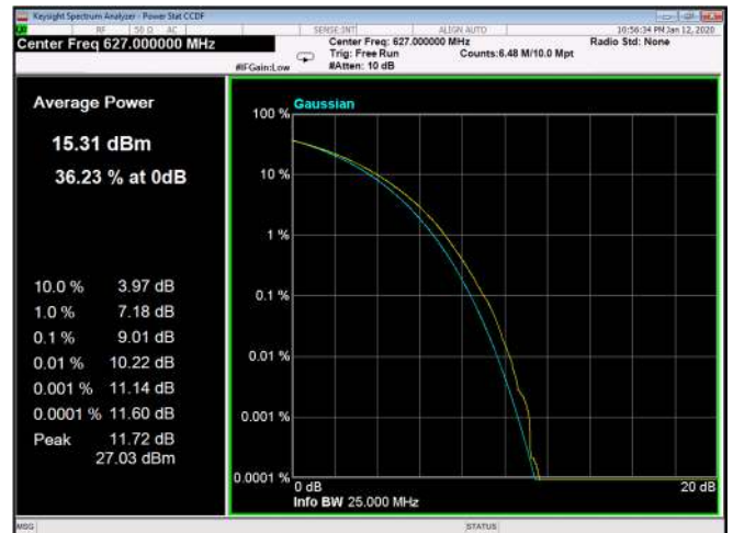
Figure 317: 256QAM 20MHz B.W; 627.0MHz, 15kHz
