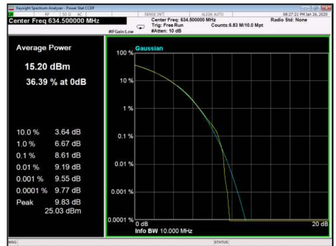
Figure 240: 16QAM 10MHz B.W; 634.5MHz, 60kHz
