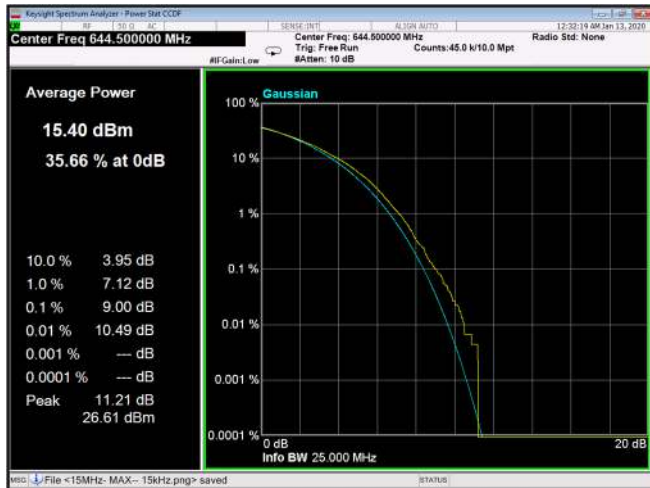
Figure 282: 64QAM 15MHz B.W; 644.5MHz, 30kHz
