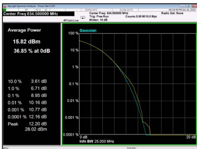
Figure 243: 16QAM 15MHz B.W; 634.5MHz, 15kHz
