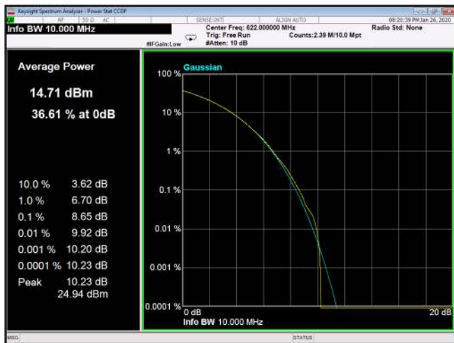
Figure 233: 16QAM 10MHz B.W; 622.0MHz, 15kHz
