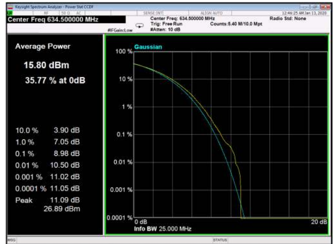
Figure 289: 64QAM 20MHz B.W; 634.5MHz, 60kHz
