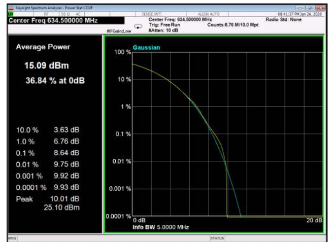
Figure 228: 16QAM 5MHz B.W; 634.5MHz, 15kHz
