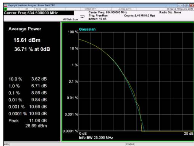
Figure 252: 16QAM 20MHz B.W; 634.5MHz, 15kHz
