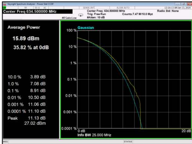
Figure 270: 64QAM 10MHz B.W; 634.5MHz, 30kHz
