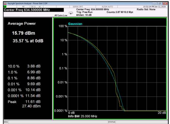
Figure 313: 256QAM 15MHz B.W; 634.5MHz, 30kHz
