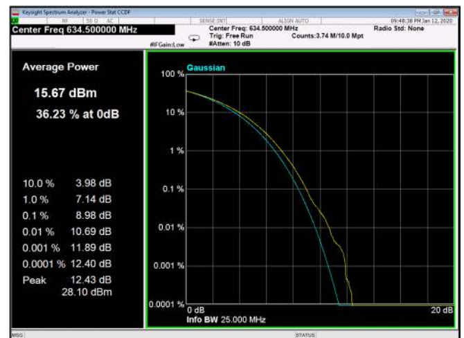
Figure 351: QPSK 20MHz B.W; 634.5MHz, 15kHz
