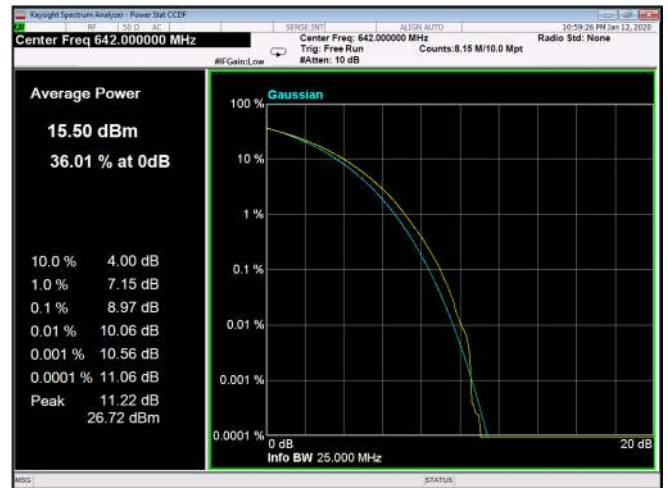
Figure 323: 256QAM 20MHz B.W; 642.0MHz, 15kHz
