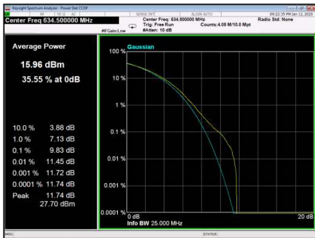
Figure 336: QPSK 10MHz B.W; 634.5MHz, 30kHz
