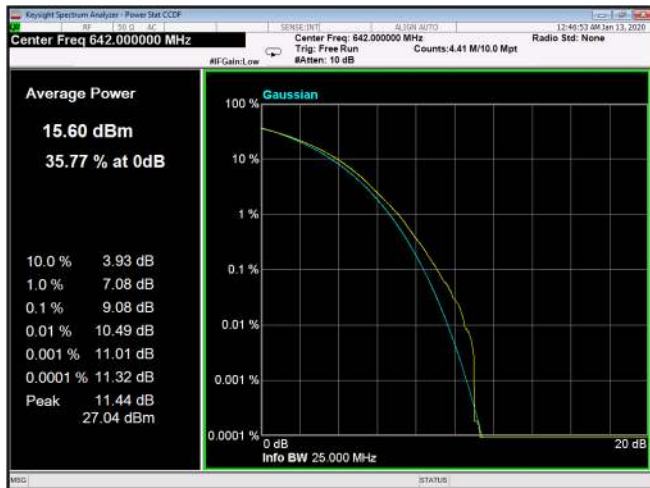
Figure 292: 64QAM 20MHz B.W; 642.0MHz, 60kHz
