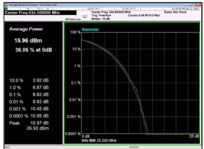
Figure 303: 256QAM 10MHz B.W; 634.5MHz, 30kHz
