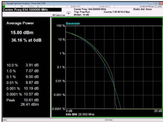
Figure 312: 256QAM 15MHz B.W; 634.5MHz, 30kHz
