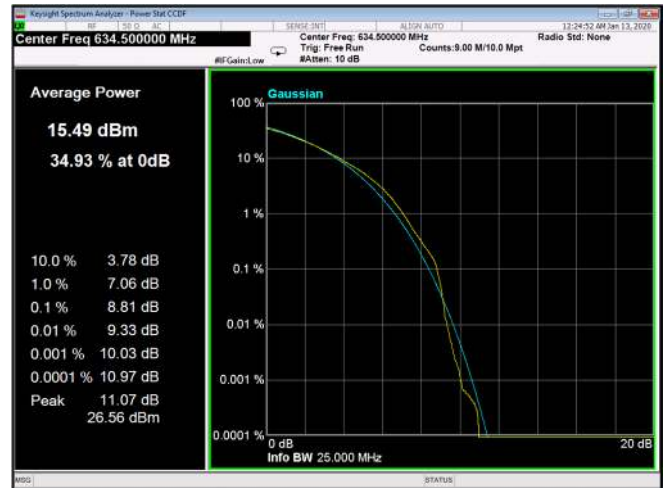
Figure 271: 64QAM 10MHz B.W; 634.5MHz, 60kHz
