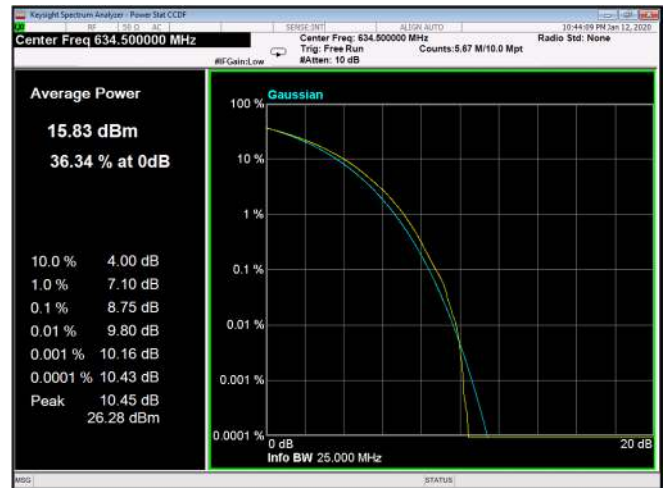
Figure 311: 256QAM 15MHz B.W; 634.5MHz, 15kHz
