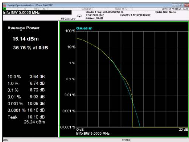
Figure 229: 16QAM 5MHz B.W; 649.5MHz, 15kHz
