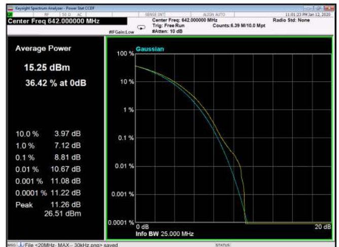
Figure 321: 256QAM 20MHz B.W; 642.0MHz, 30kHz
