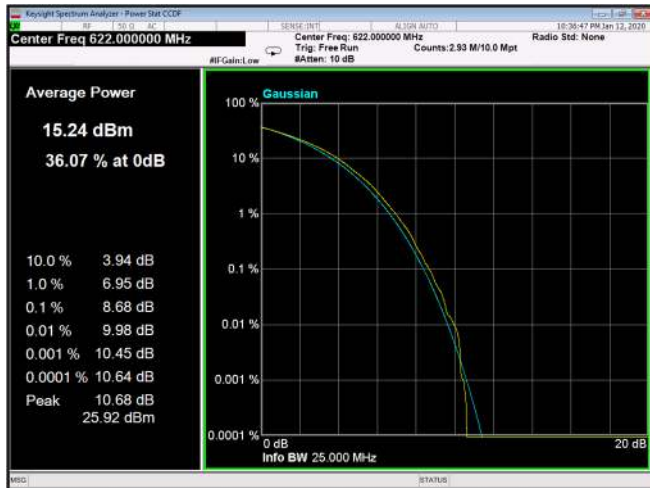
Figure 300: 256QAM 10MHz B.W; 622.0MHz, 30kHz
