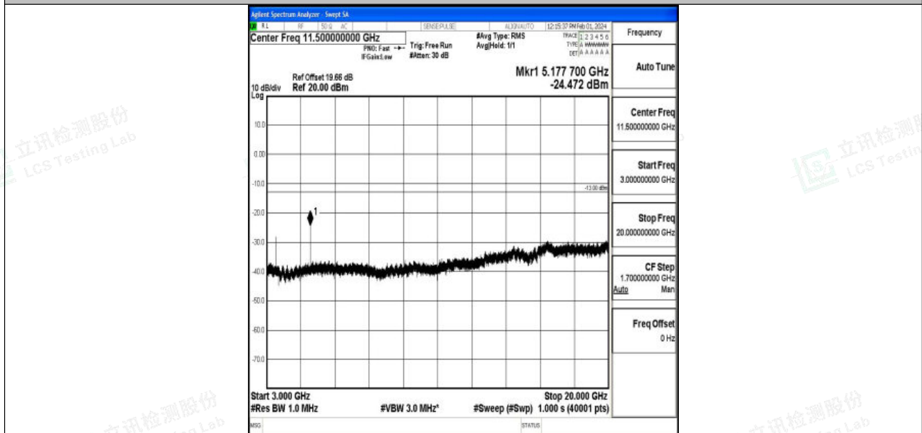
Band4_15MHz_16QAM_20175_1RB#0_3000~20000_3000~20000
