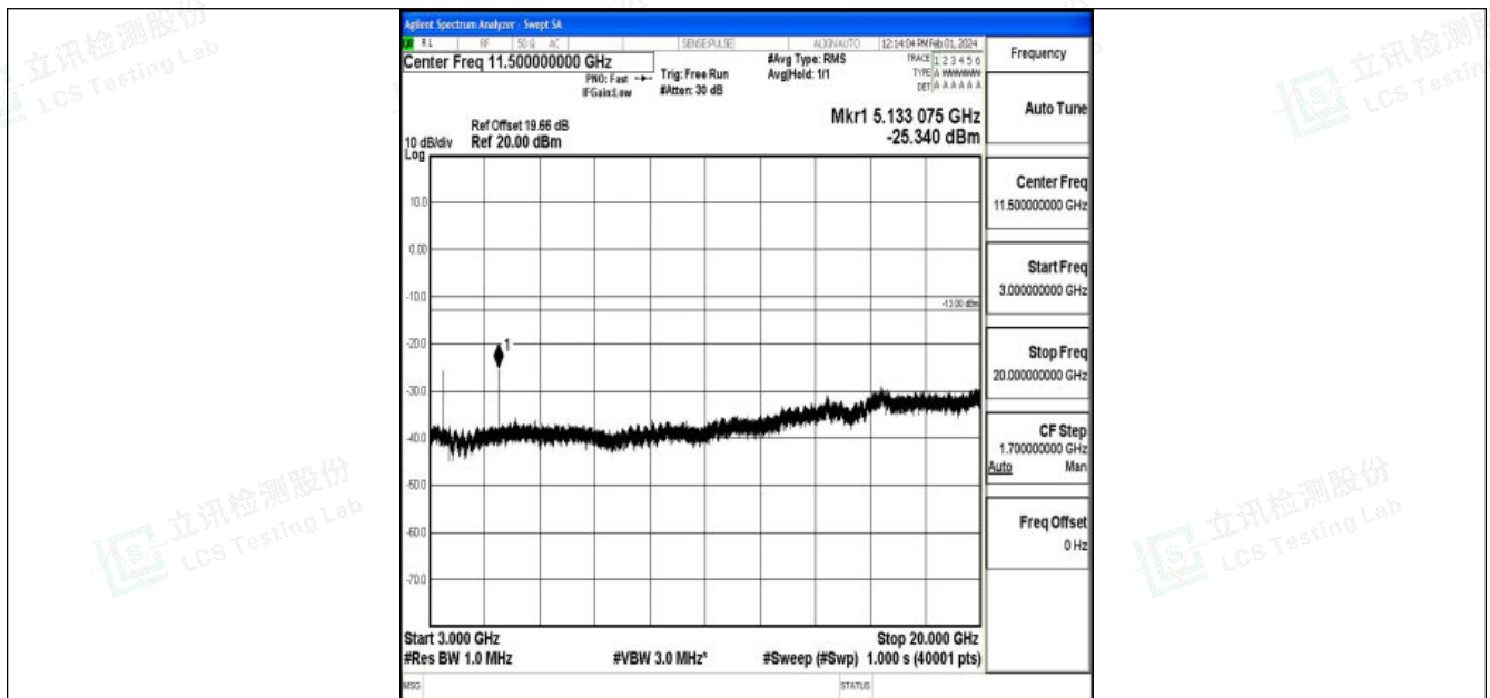
Band4_15MHz_QPSK_20025_1RB#0_3000~20000_3000~20000
