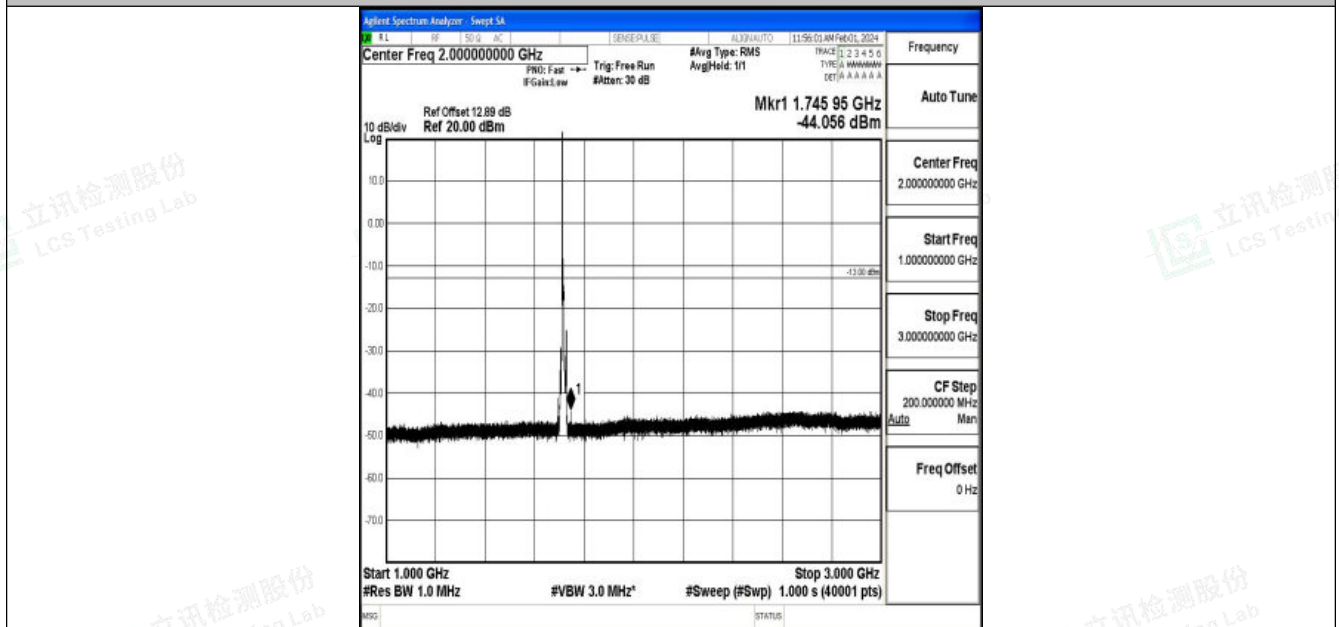
Band4_10MHz_QPSK_20000_1RB#0_1000~3000_1000~3000
