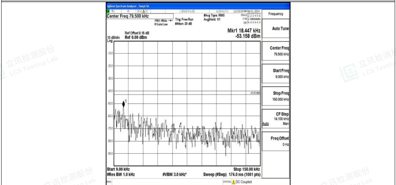
Band4_20MHz_16QAM_20175_1RB#0_0.009~0.15_0.009~0.15
