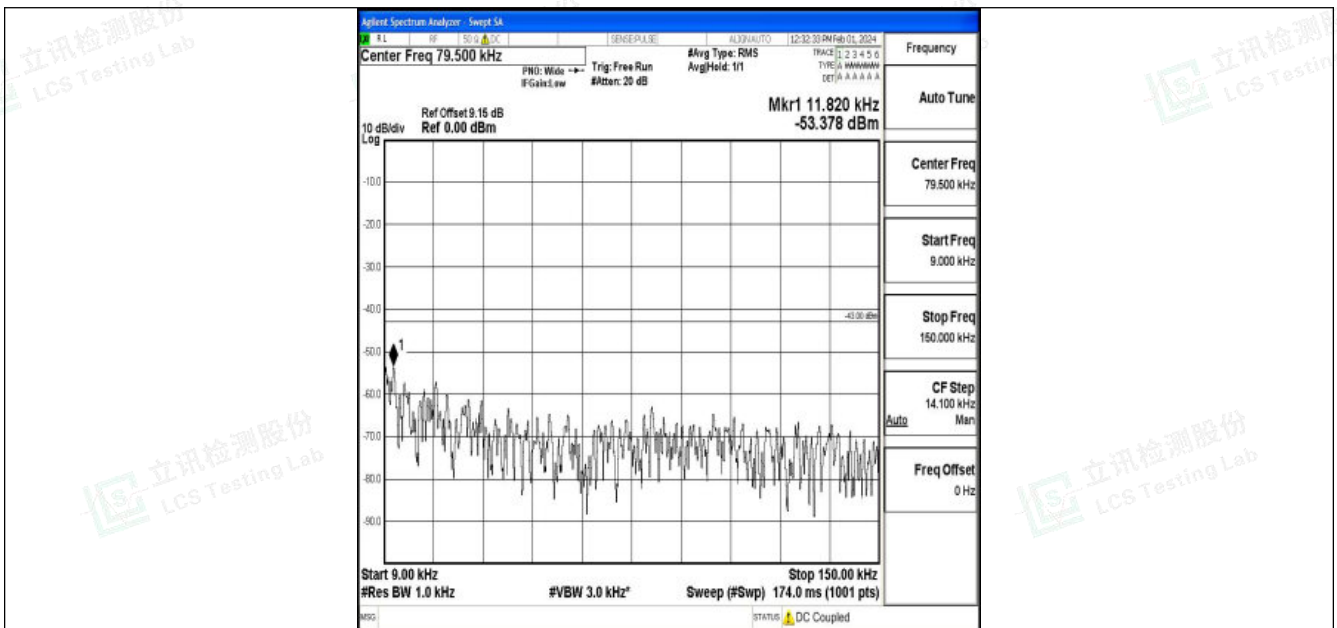
Band4_20MHz_QPSK_20175_1RB#0_0.009~0.15_0.009~0.15
