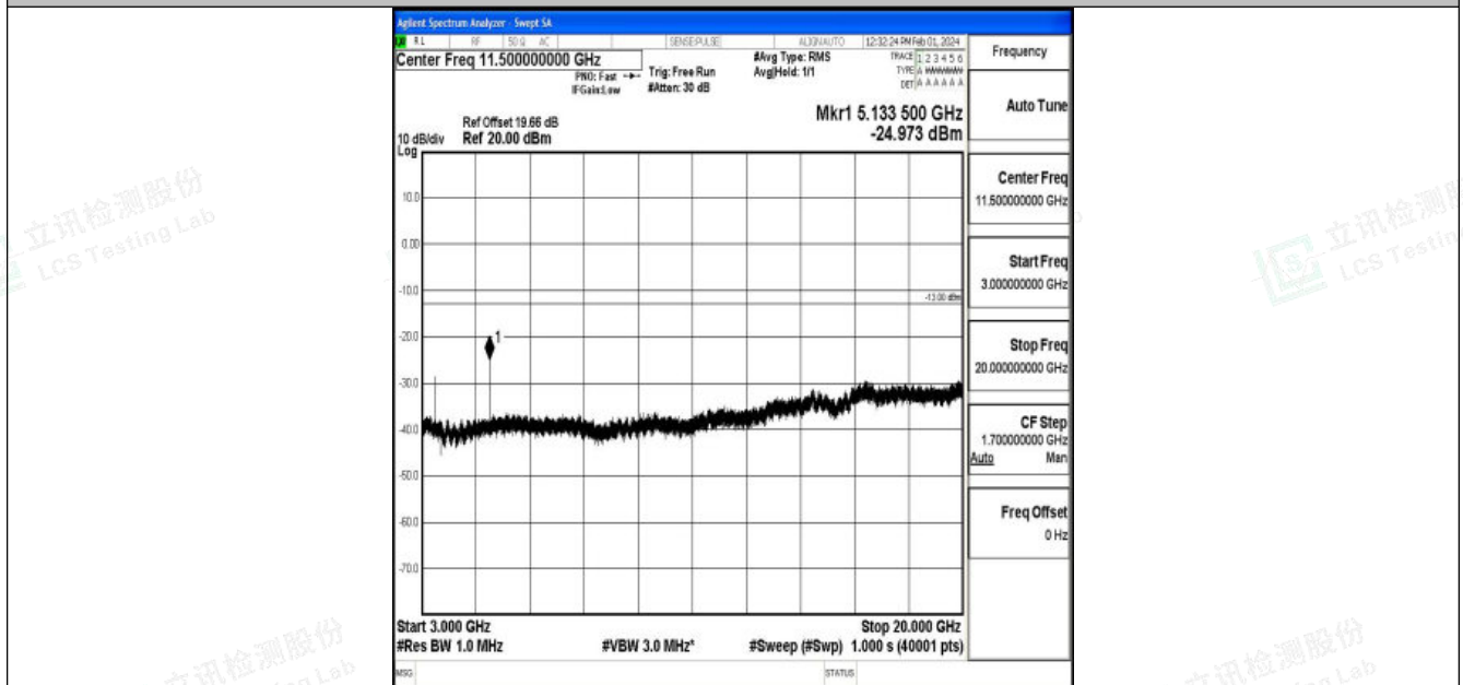
Band4_20MHz_16QAM_20050_1RB#0_3000~20000_3000~20000
