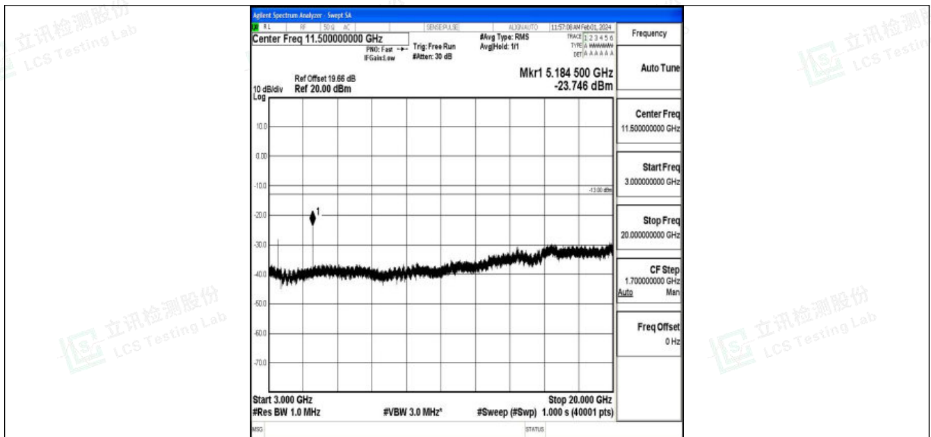
Band4_10MHz_QPSK_20175_1RB#0_3000~20000_3000~20000
