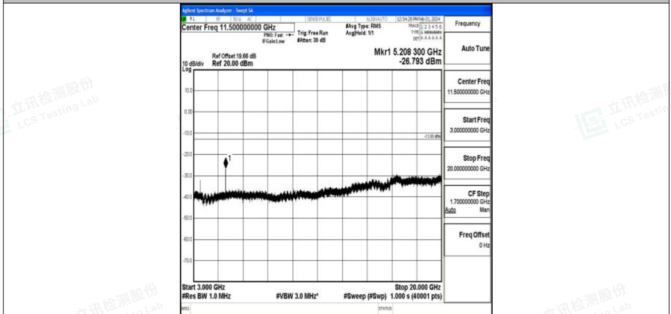
Band4_20MHz_16QAM_20300_1RB#0_3000~20000_3000~20000
