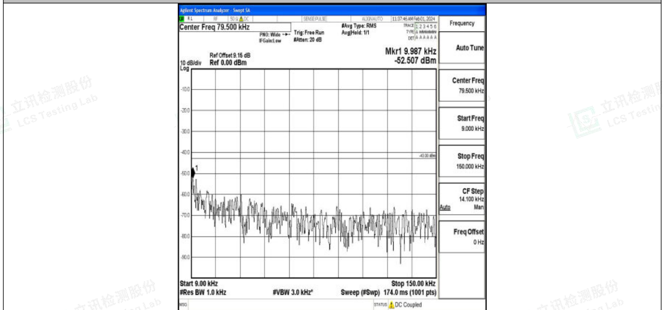
Band4_5MHz_16QAM_20175_1RB#0_0.009~0.15_0.009~0.15
