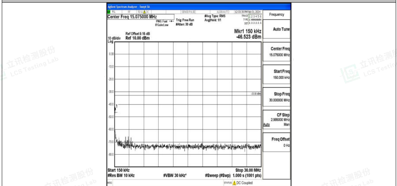
Band4_20MHz_QPSK_20300_1RB#0_0.15~30_0.15~30
