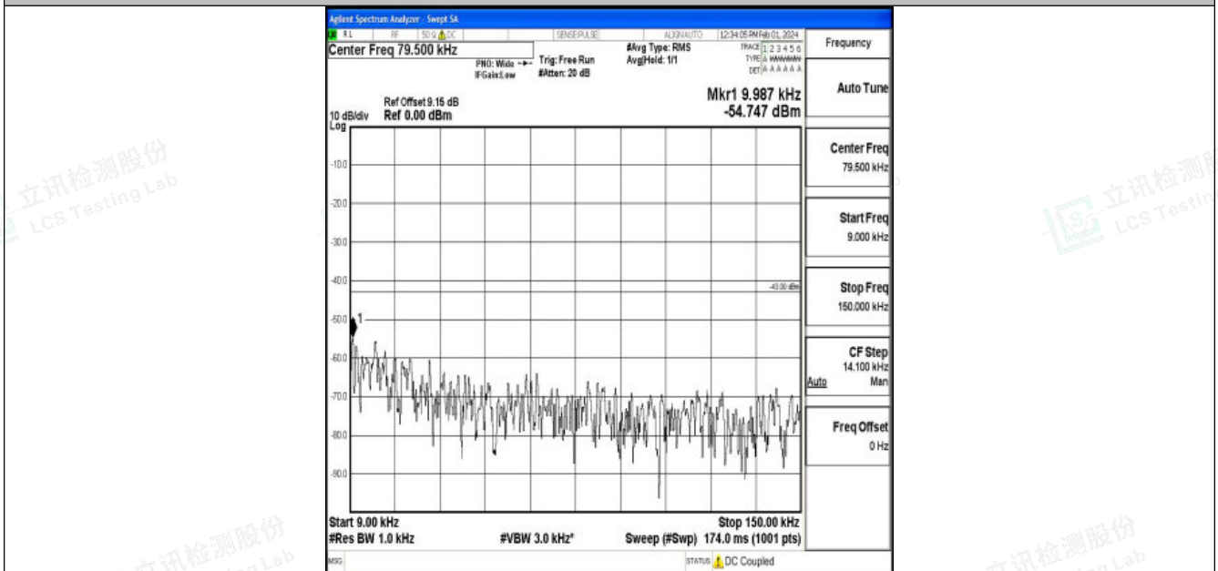
Band4_20MHz_16QAM_20300_1RB#0_0.009~0.15_0.009~0.15
