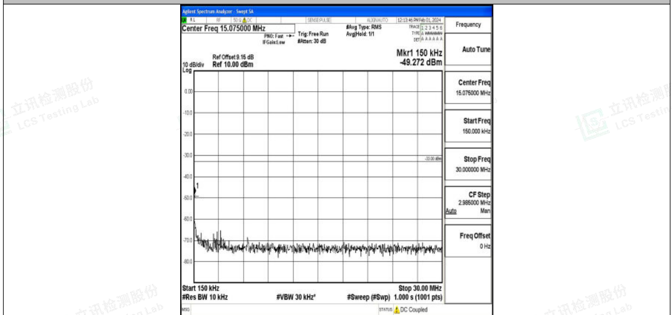
Band4_15MHz_QPSK_20025_1RB#0_0.15~30_0.15~30
