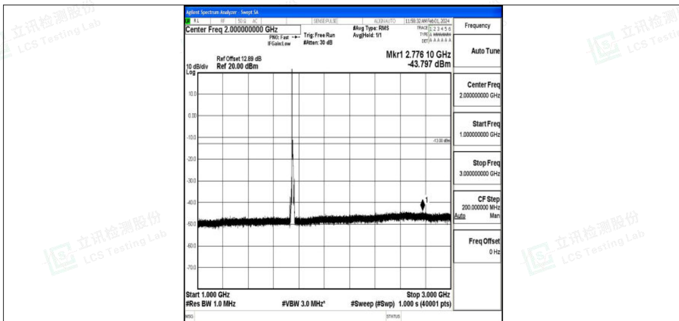
Band4_10MHz_16QAM_20350_1RB#0_1000~3000_1000~3000
