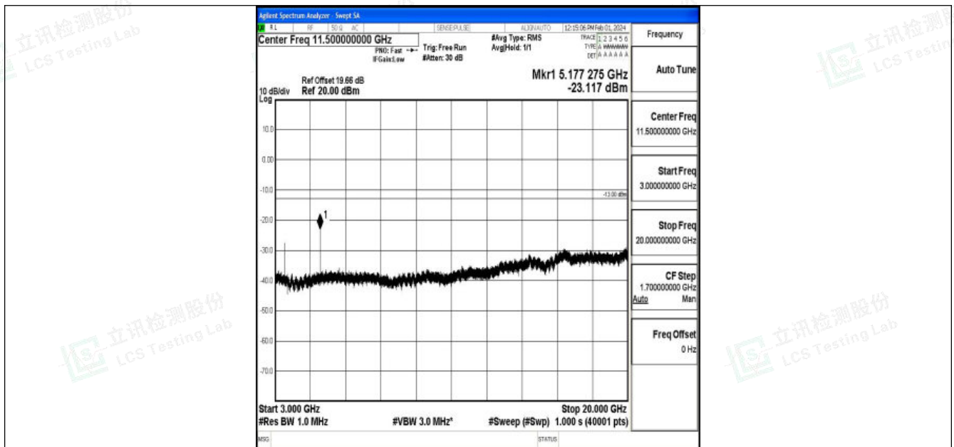
Band4_15MHz_QPSK_20175_1RB#0_3000~20000_3000~20000
