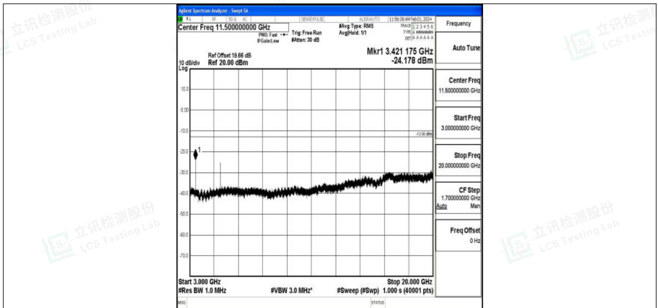
Band4_10MHz_QPSK_20000_1RB#0_3000~20000_3000~20000
