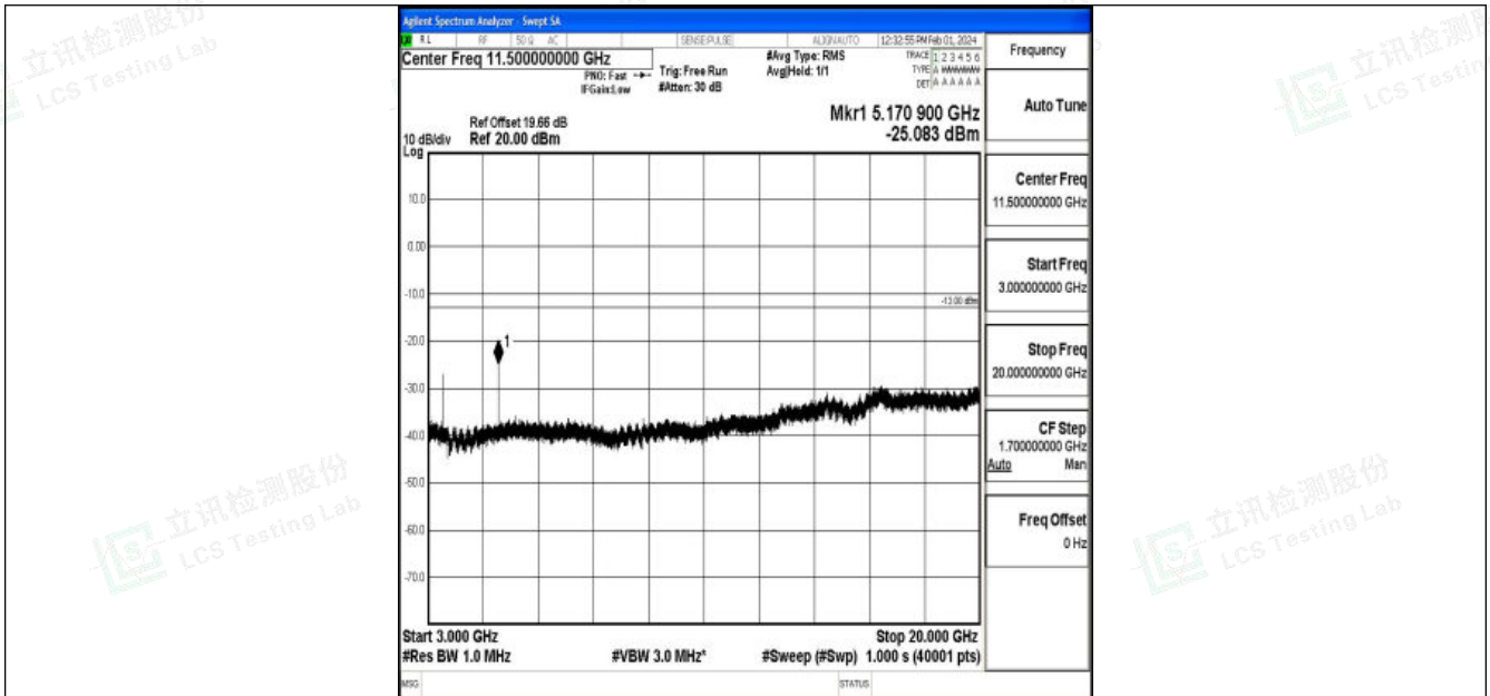
Band4_20MHz_QPSK_20175_1RB#0_3000~20000_3000~20000
