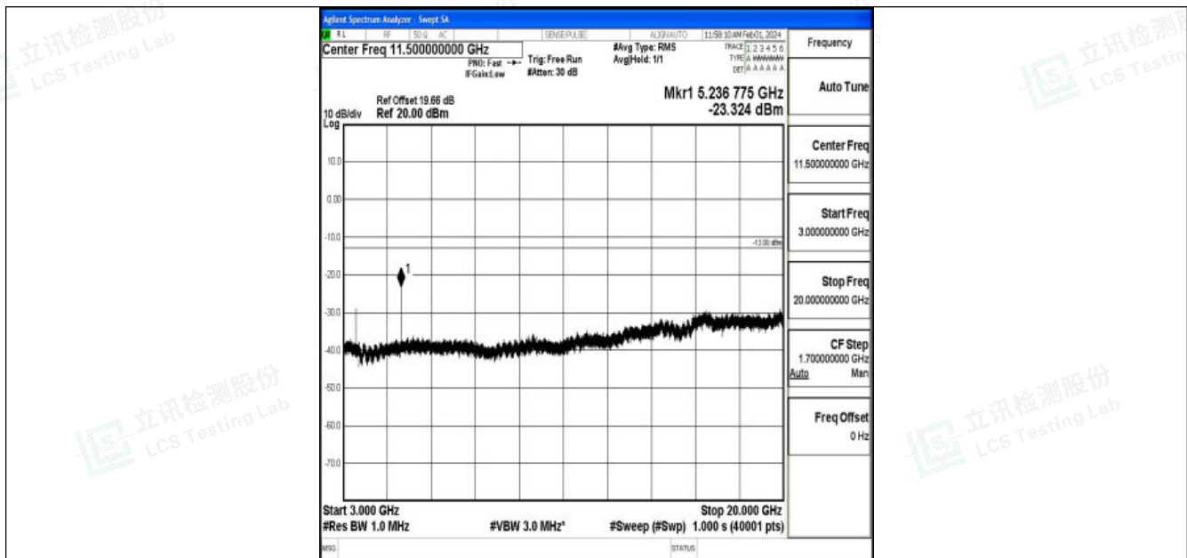
Band4_10MHz_QPSK_20350_1RB#0_3000~20000_3000~20000
