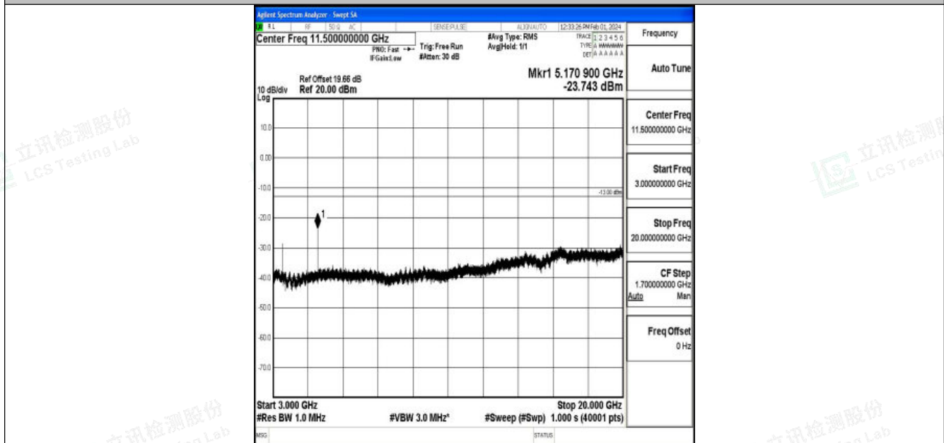
Band4_20MHz_16QAM_20175_1RB#0_3000~20000_3000~20000
