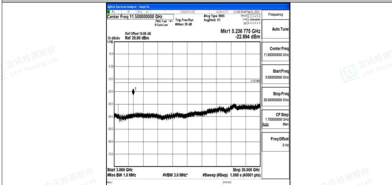
Band4_10MHz_16QAM_20350_1RB#0_3000~20000_3000~20000
