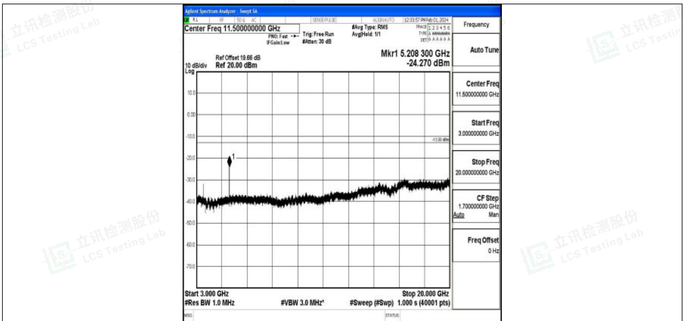
Band4_20MHz_QPSK_20300_1RB#0_3000~20000_3000~20000
