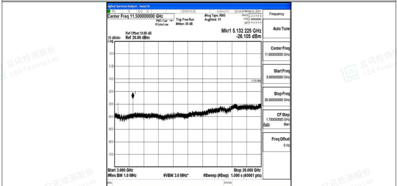
Band4_15MHz_16QAM_20025_1RB#0_3000~20000_3000~20000
