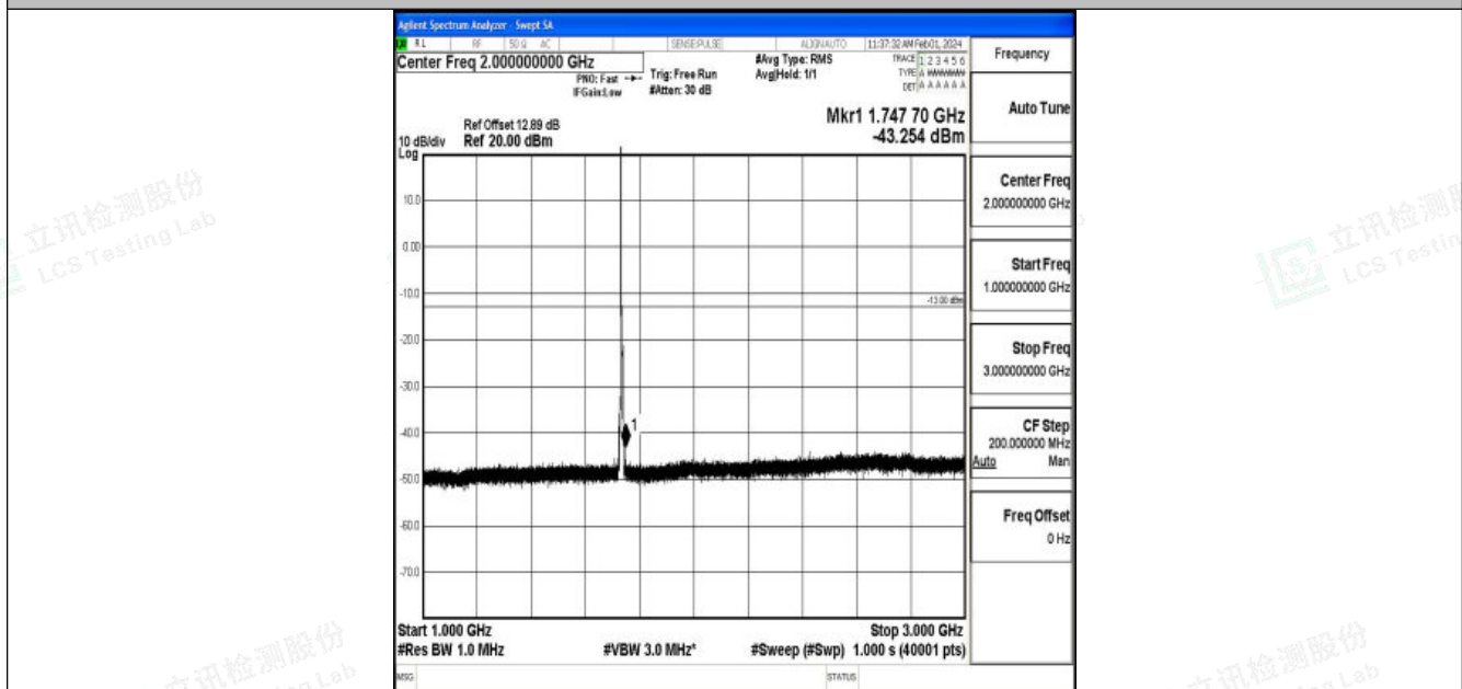
Band4_5MHz_QPSK_20175_1RB#0_1000~3000_1000~3000
