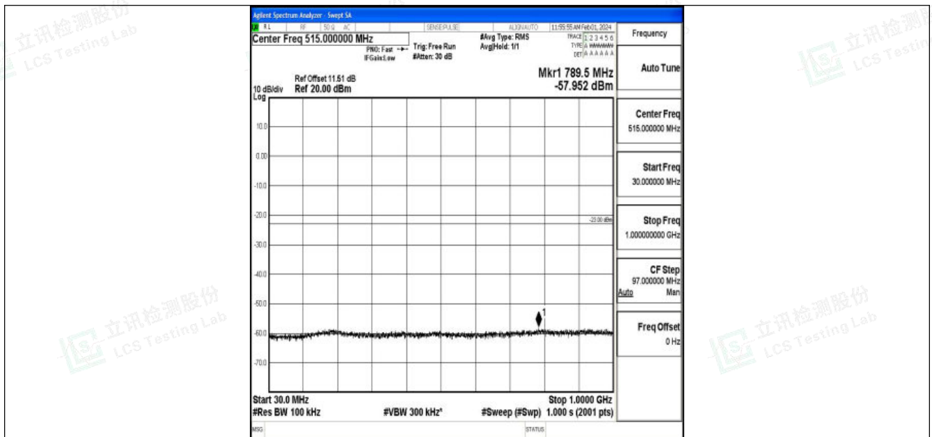
Band4_10MHz_QPSK_20000_1RB#0_30~1000_30~1000
