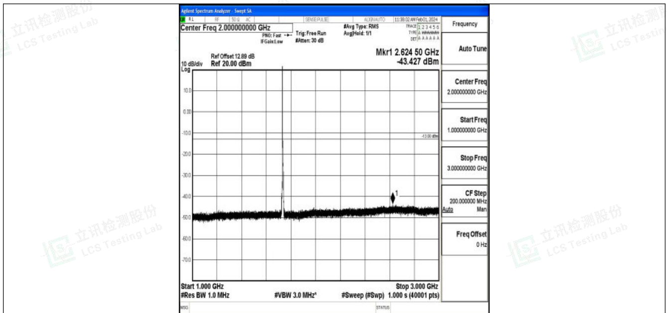
Band4_5MHz_16QAM_20175_1RB#0_1000~3000_1000~3000
