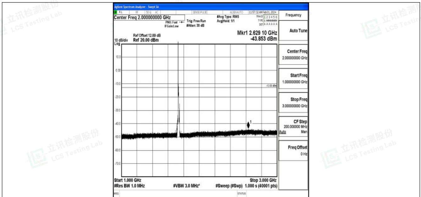
Band4_10MHz_16QAM_20175_1RB#0_1000~3000_1000~3000
