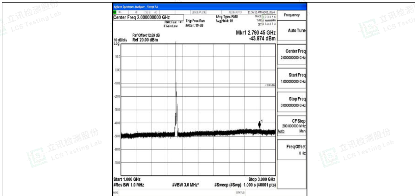
Band4_10MHz_16QAM_20000_1RB#0_1000~3000_1000~3000
