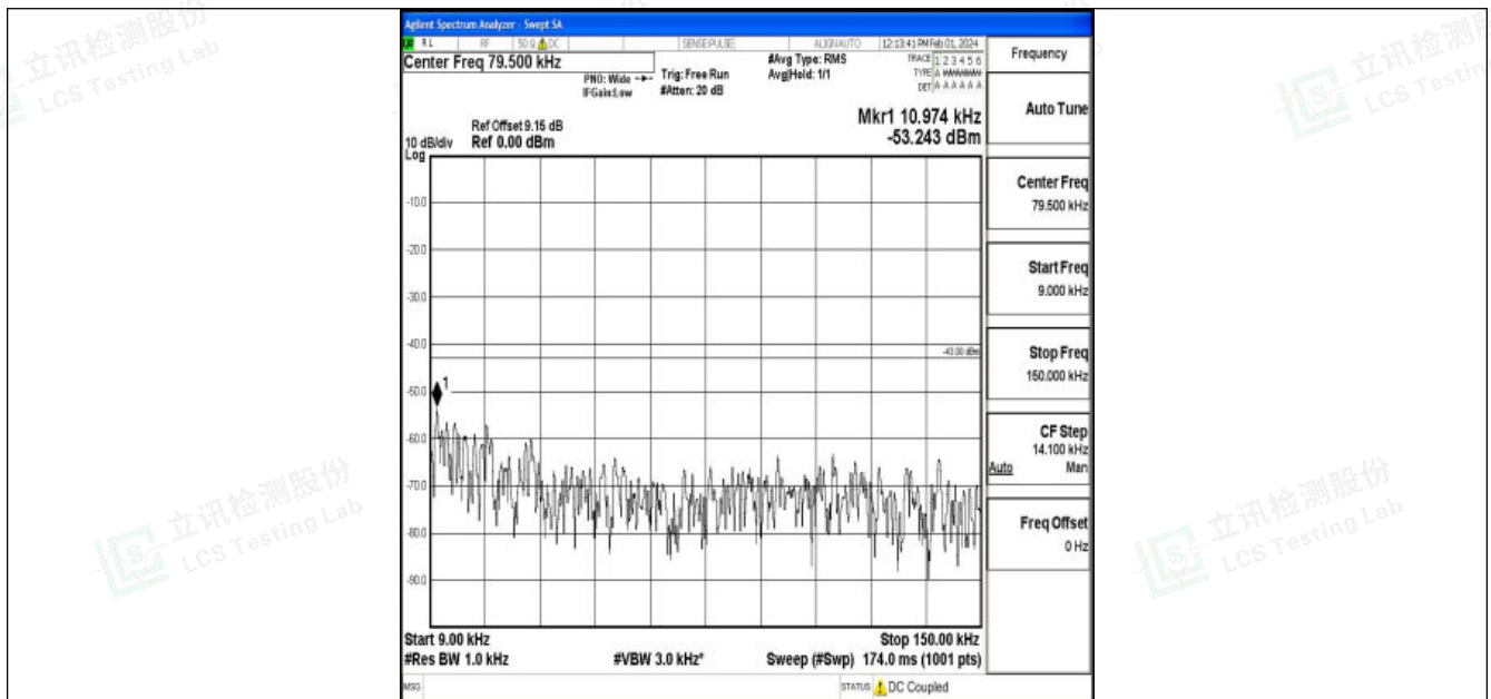
Band4_15MHz_QPSK_20025_1RB#0_0.009~0.15_0.009~0.15
