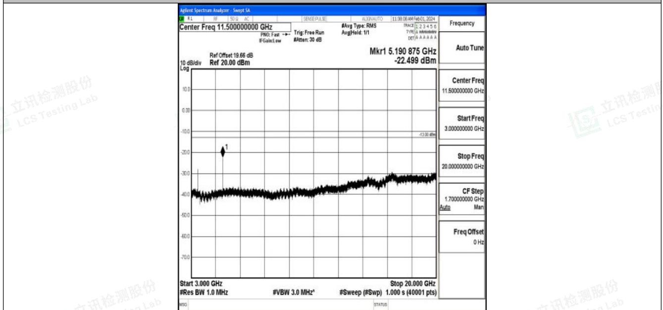
Band4_5MHz_16QAM_20175_1RB#0_3000~20000_3000~20000
