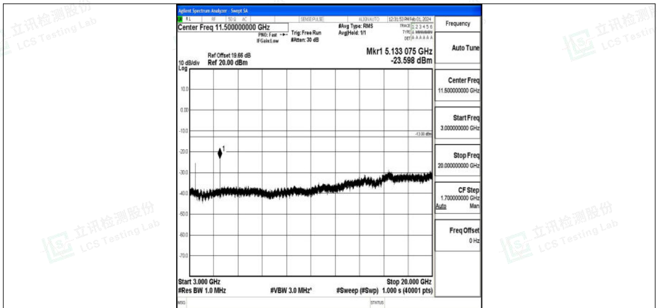
Band4_20MHz_QPSK_20050_1RB#0_3000~20000_3000~20000
