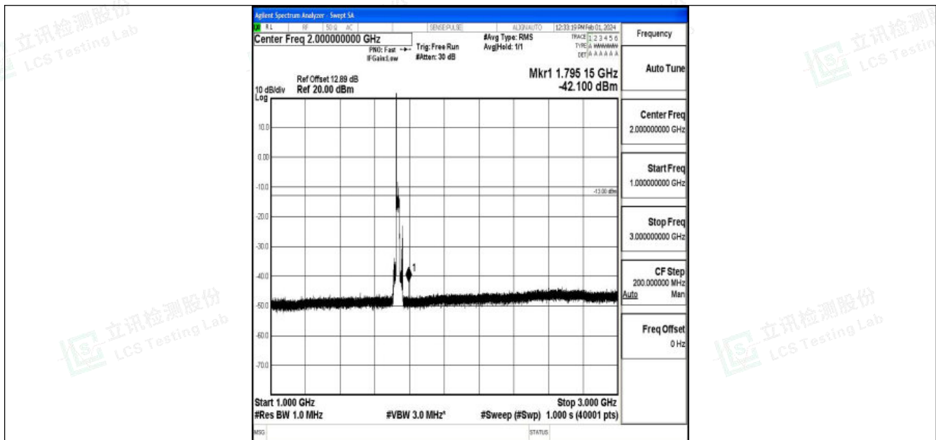
Band4_20MHz_16QAM_20175_1RB#0_1000~3000_1000~3000
