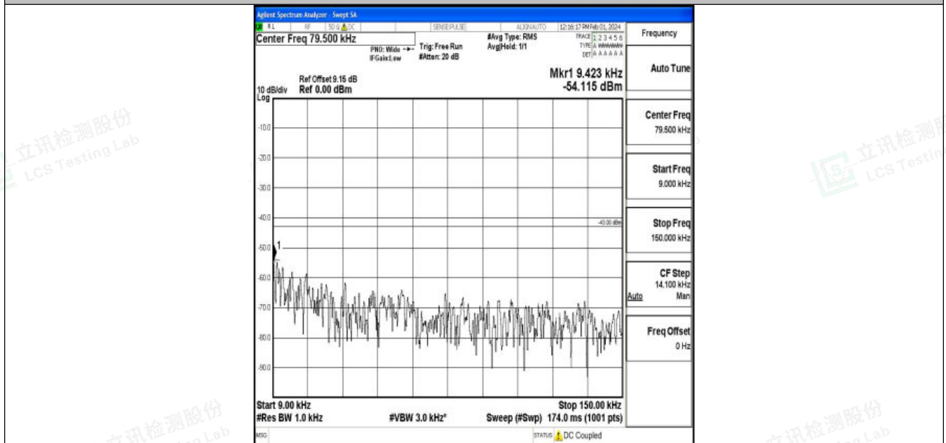
Band4_15MHz_16QAM_20325_1RB#0_0.009~0.15_0.009~0.15
