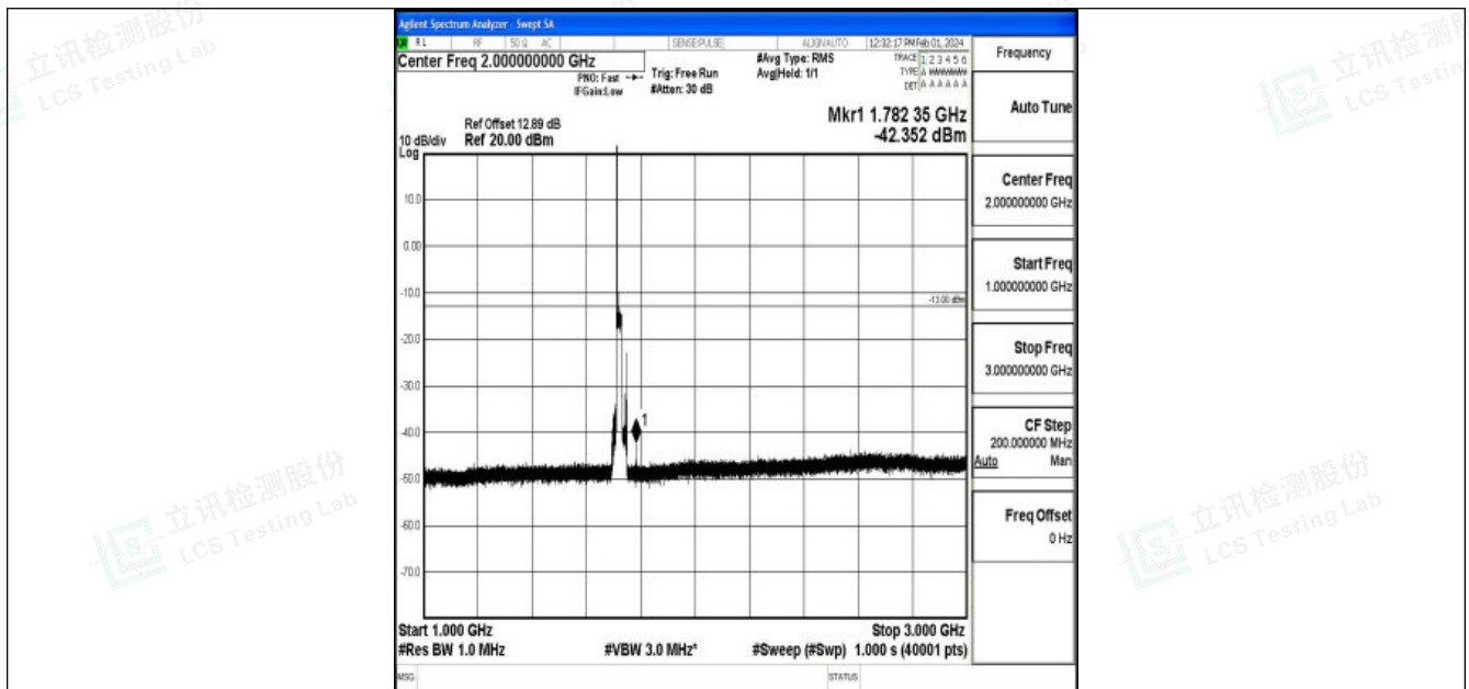
Band4_20MHz_16QAM_20050_1RB#0_1000~3000_1000~3000
