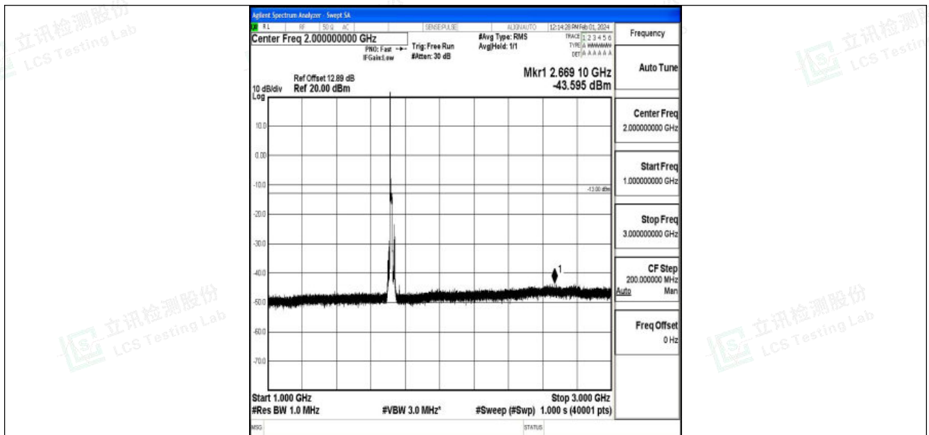
Band4_15MHz_16QAM_20025_1RB#0_1000~3000_1000~3000
