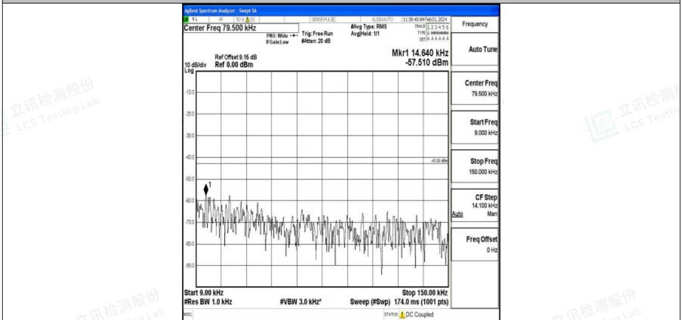
Band4_5MHz_16QAM_20375_1RB#0_0.009~0.15_0.009~0.15
