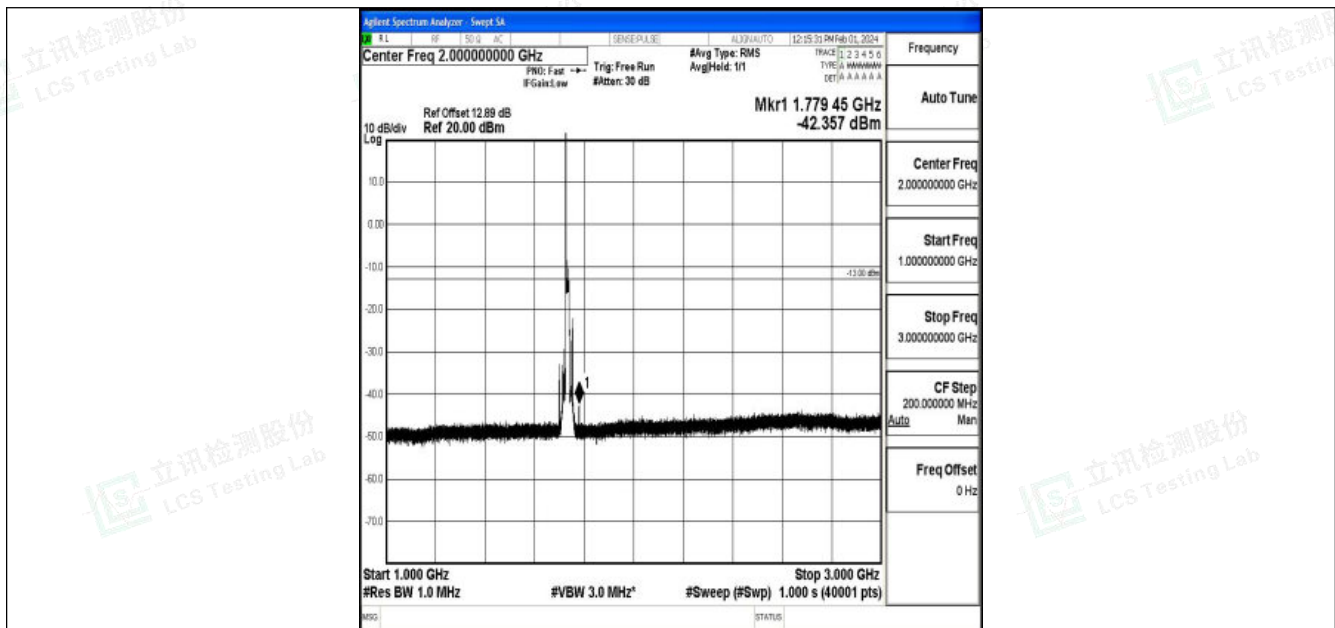
Band4_15MHz_16QAM_20175_1RB#0_1000~3000_1000~3000
