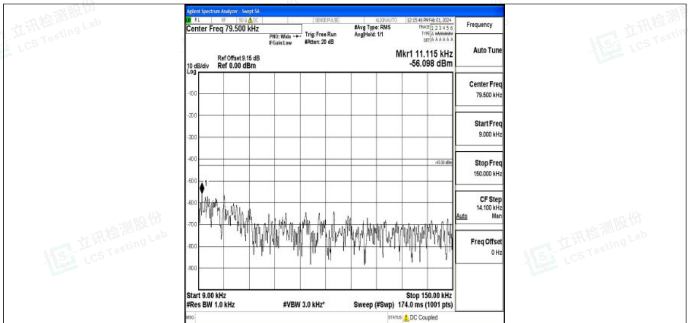
Band4_15MHz_QPSK_20325_1RB#0_0.009~0.15_0.009~0.15
