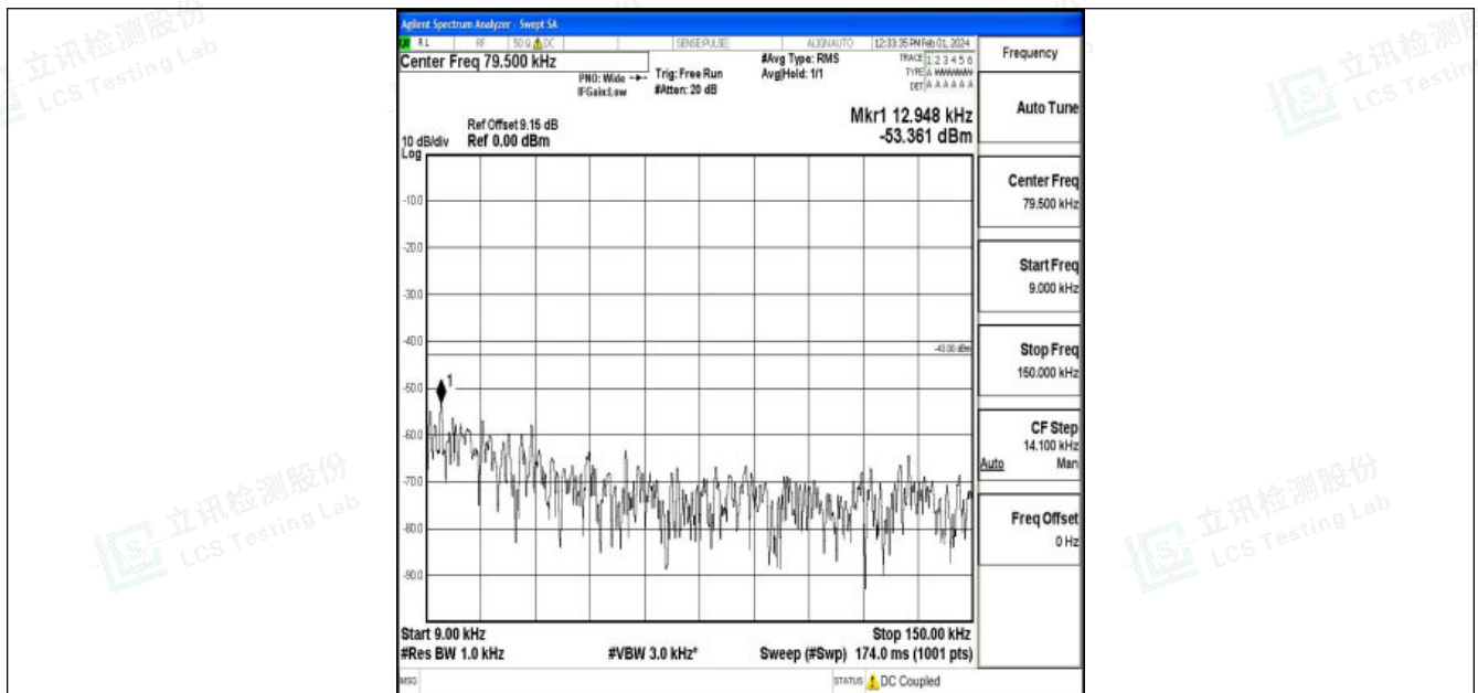
Band4_20MHz_QPSK_20300_1RB#0_0.009~0.15_0.009~0.15
