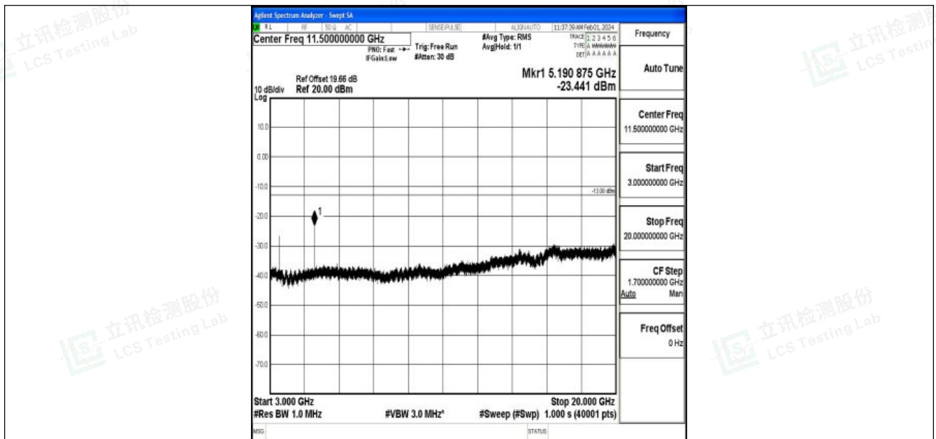
Band4_5MHz_QPSK_20175_1RB#0_3000~20000_3000~20000
