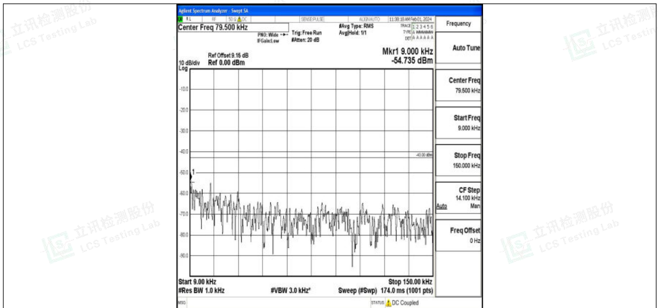
Band4_5MHz_QPSK_20375_1RB#0_0.009~0.15_0.009~0.15
