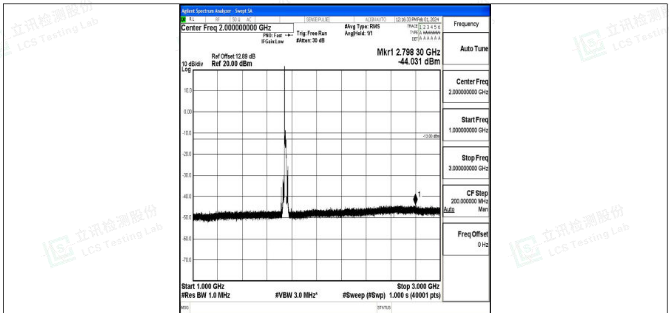
Band4_15MHz_16QAM_20325_1RB#0_1000~3000_1000~3000
