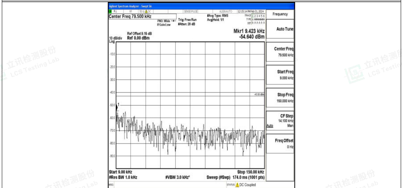
Band4_15MHz_16QAM_20175_1RB#0_0.009~0.15_0.009~0.15
