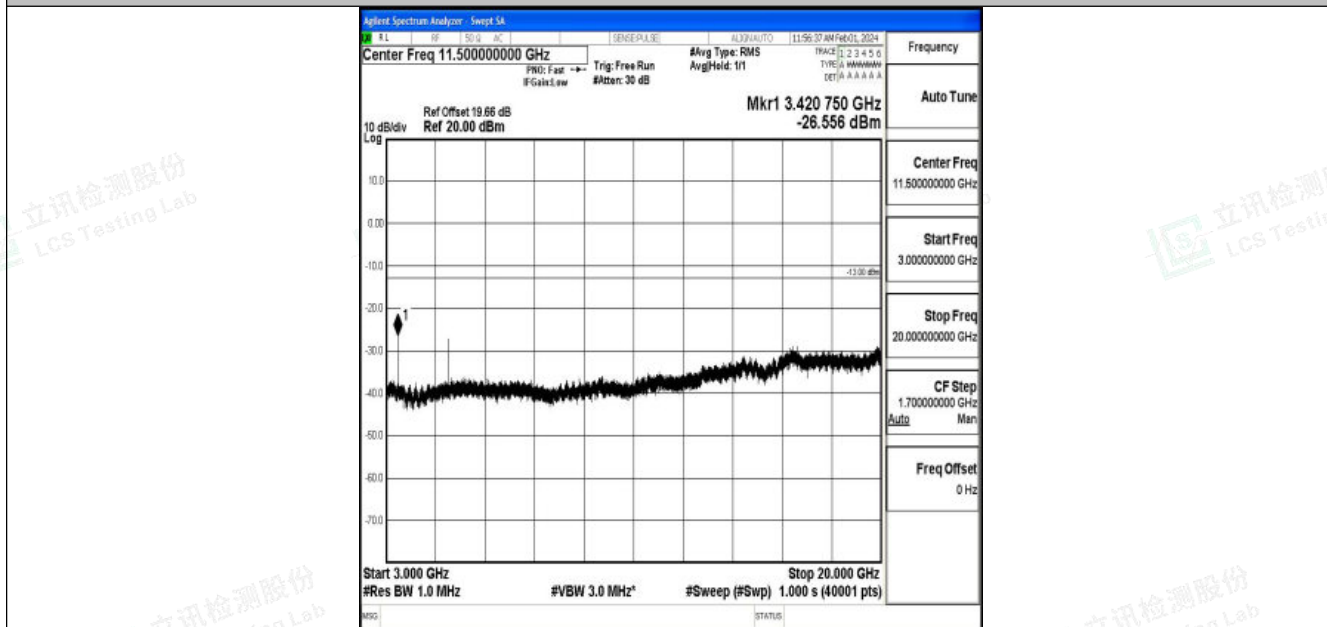
Band4_10MHz_16QAM_20000_1RB#0_3000~20000_3000~20000
