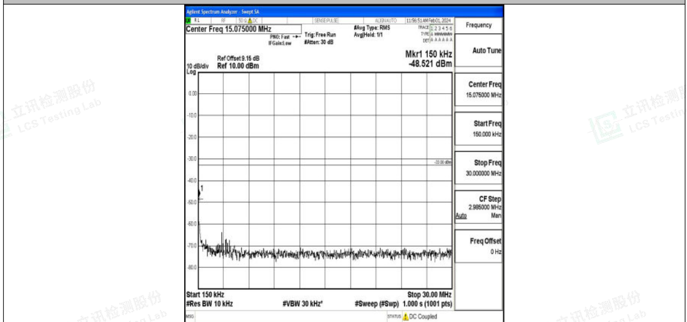
Band4_10MHz_QPSK_20175_1RB#0_0.15~30_0.15~30
