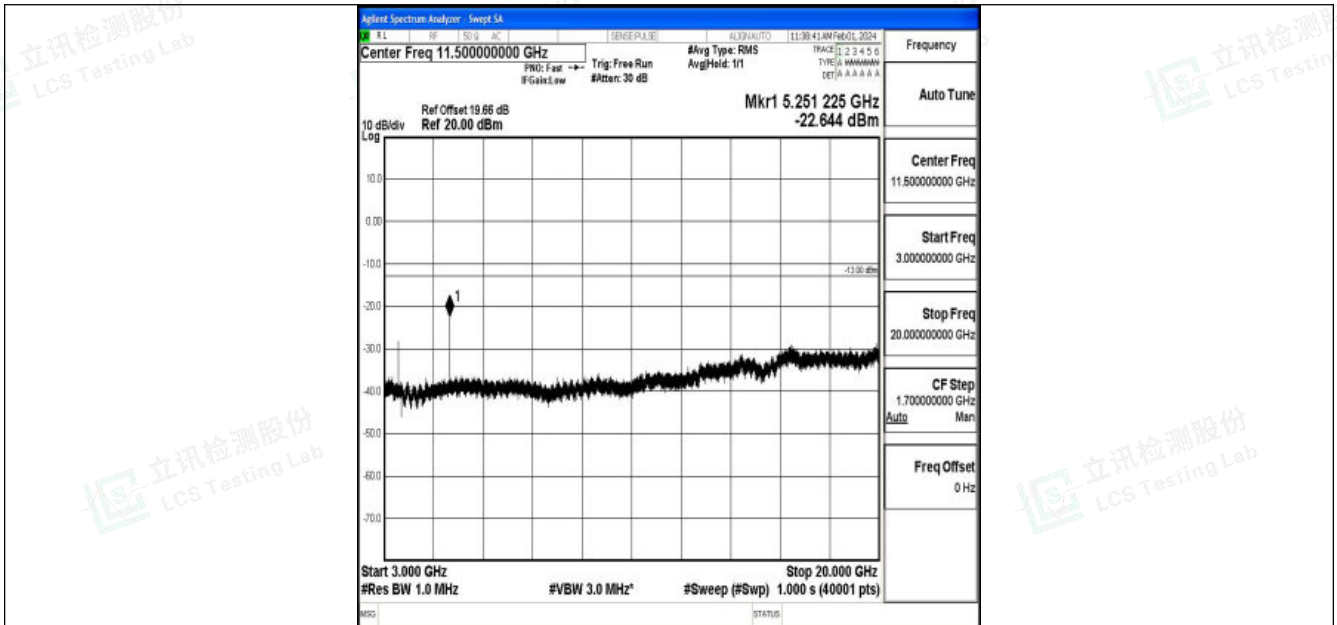
Band4_5MHz_QPSK_20375_1RB#0_3000~20000_3000~20000
