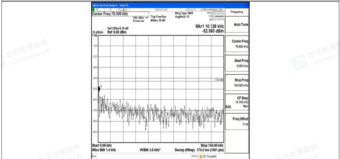
Band4_10MHz_16QAM_20000_1RB#0_0.009~0.15_0.009~0.15
