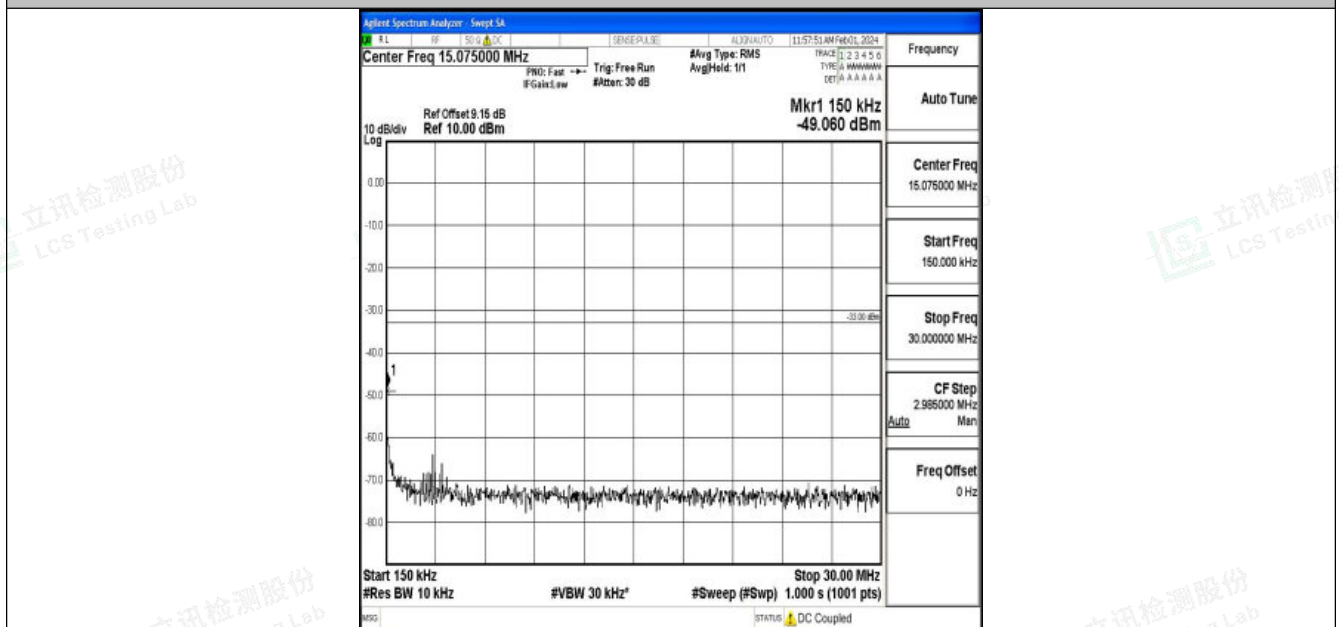
Band4_10MHz_QPSK_20350_1RB#0_0.15~30_0.15~30
