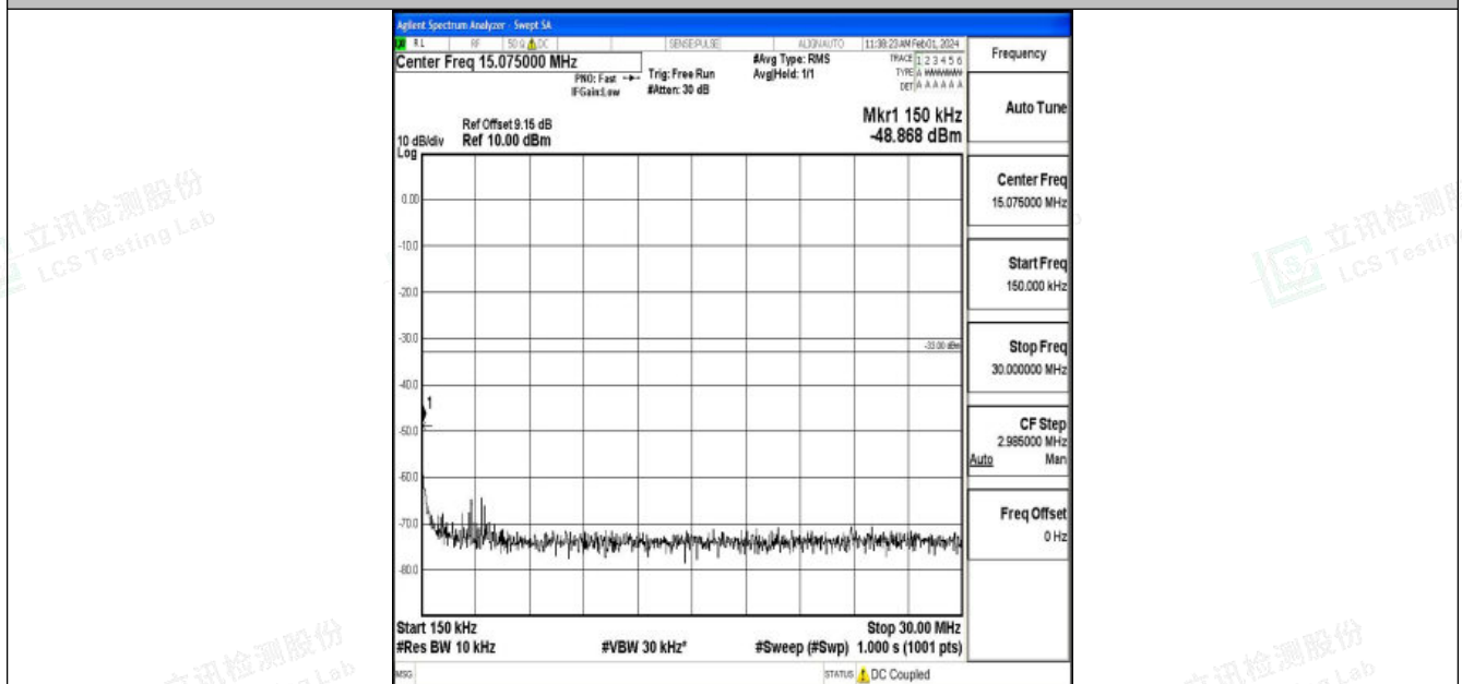
Band4_5MHz_QPSK_20375_1RB#0_0.15~30_0.15~30
