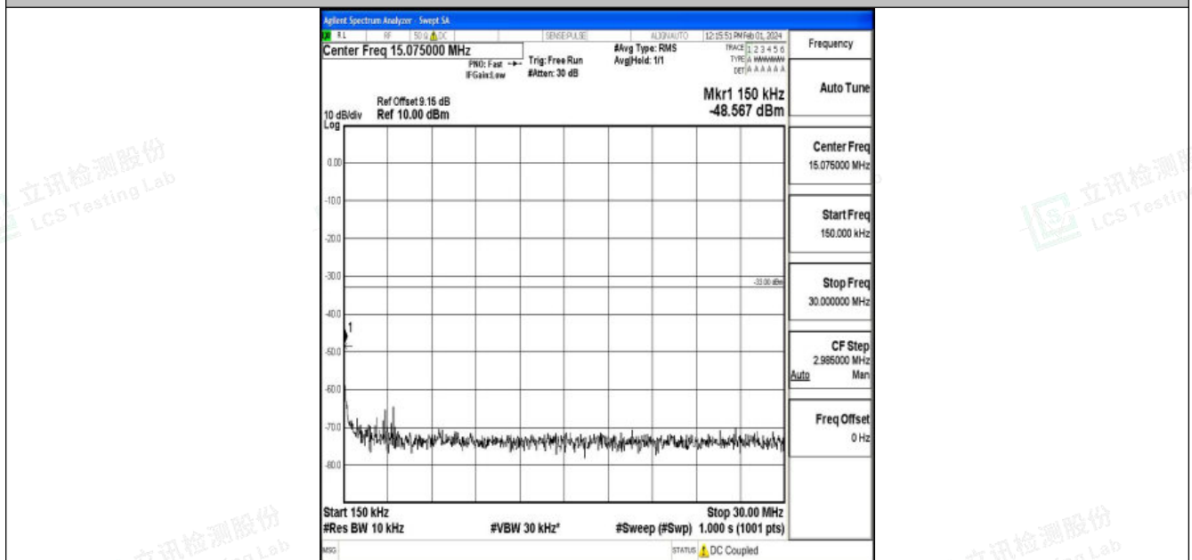
Band4_15MHz_QPSK_20325_1RB#0_0.15~30_0.15~30
