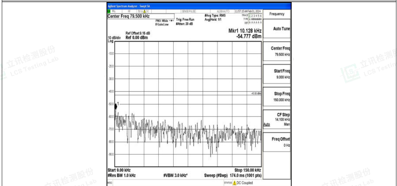
Band4_10MHz_16QAM_20175_1RB#0_0.009~0.15_0.009~0.15
