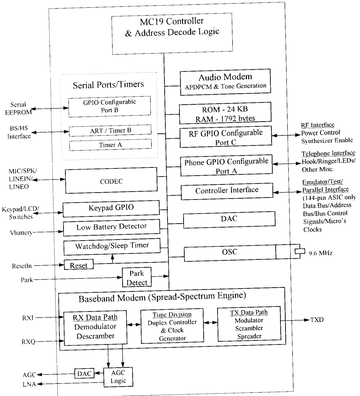
Hummingbird 100pin ASIC Block Diagram
