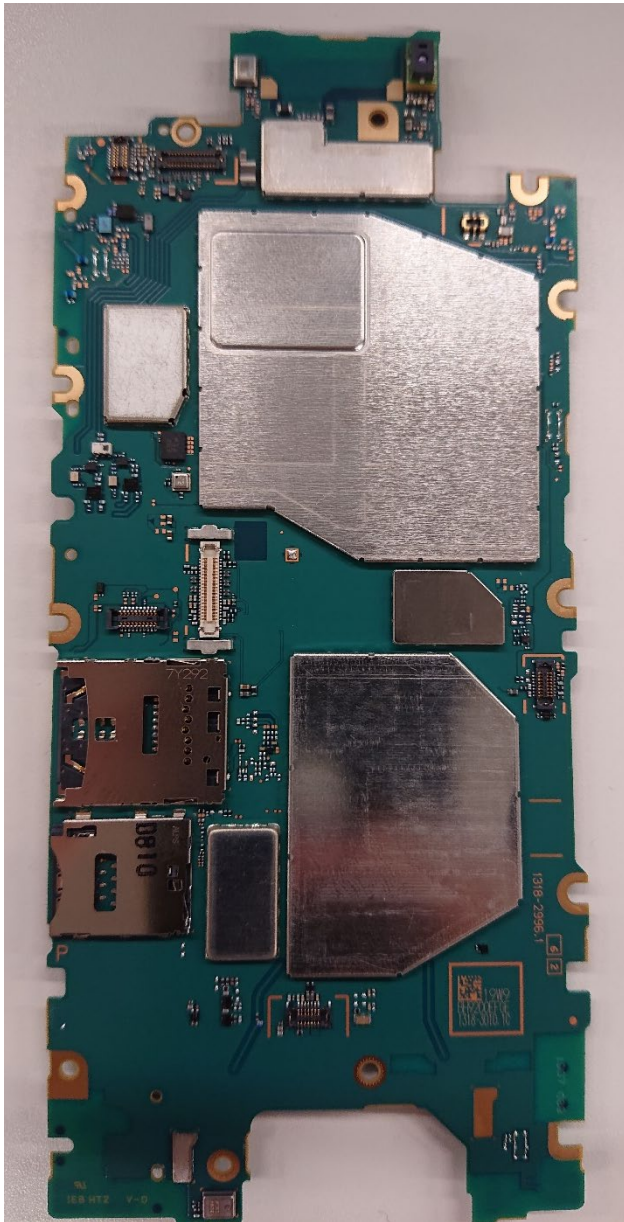
Internal PWB with Shield cases (Front-side)
