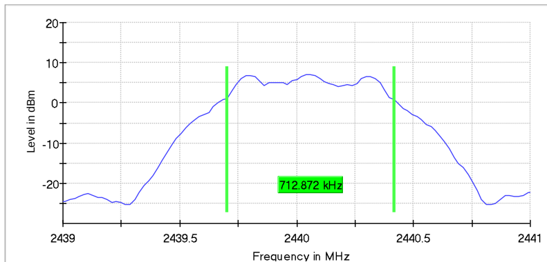
6 dB Bandwidth
