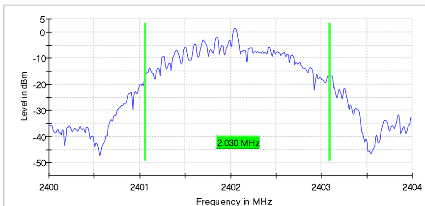
99 % Bandwidth
