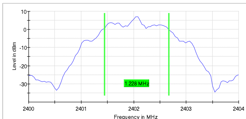
6 dB Bandwidth
