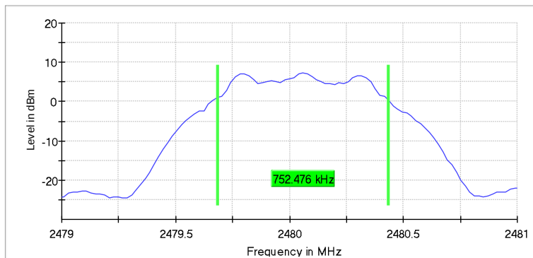
6 dB Bandwidth
