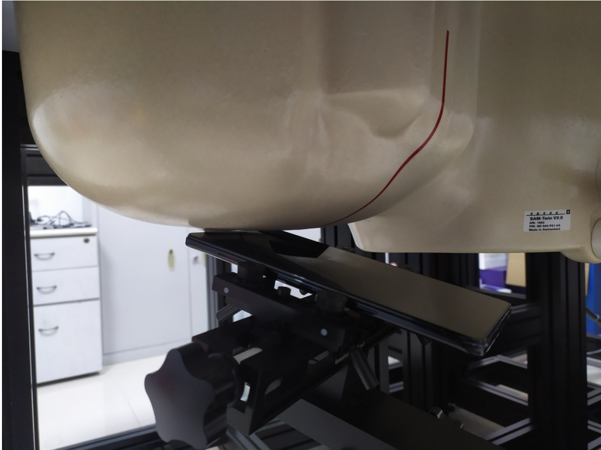
Head Right Tilt Setup Photo
