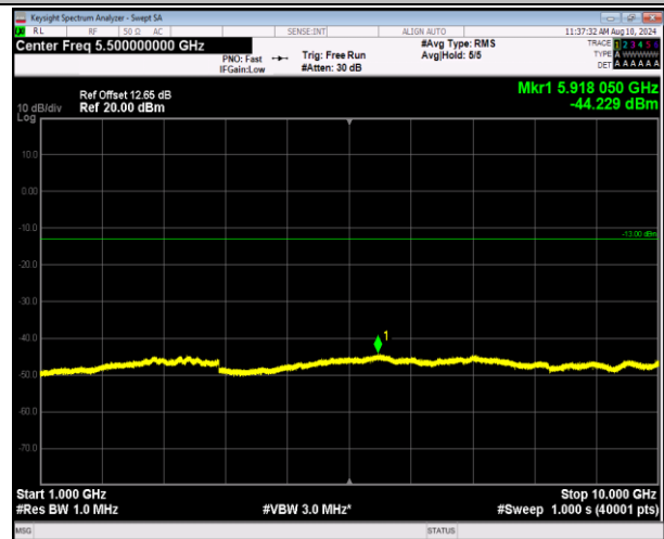
5-5-MHz-3MHz-QPSK-QPSK-20510-20549-1RB#0-0RB#0-1000~10000MHz-PASS
