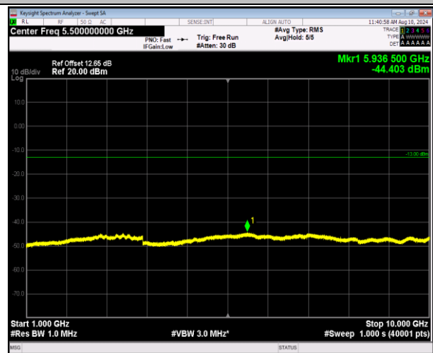
5-5-MHz-3MHz-QPSK-QPSK-20510-20549-25RB#0-15RB #0-1000~10000MHz-PASS
