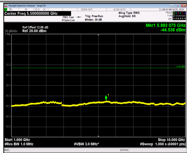
5-5-5MHz-3MHz-64QAM-64QAM-20595-20634-25RB#0-15RB#0-1000~10000MHz-PASS
