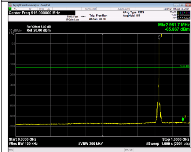
5-5-5MHz-3MHz-16QAM-16QAM-20425-20464-1RB#24-0 ORB#0-30~1000MHz-PASS
