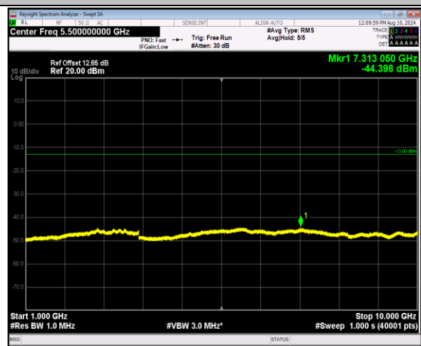
5-5-10MHz-10MHz-QPSK-QPSK-20476-20575-1RB#49-0RB#0-1000~10000MHz-PASS
