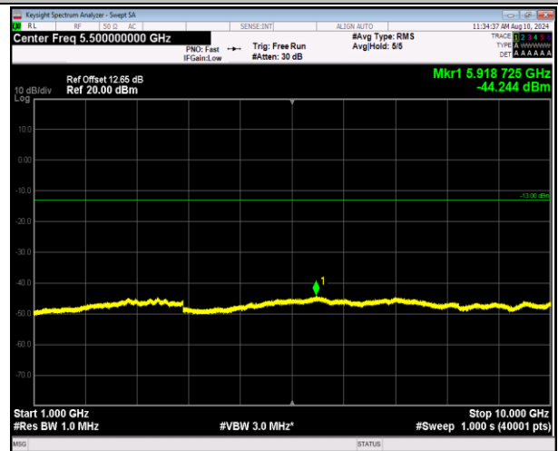
5-5-5MHz-3MHz-16QAM-16QAM-20425-20464-1RB#24-0R B#0-1000~10000MHz-PASS
