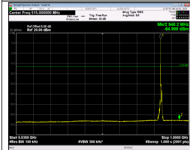
5-5-5MHz-3MHz-64QAM-64QAM-20595-20634-1RB#0-1RB#15-30~1000MHz-PASS
