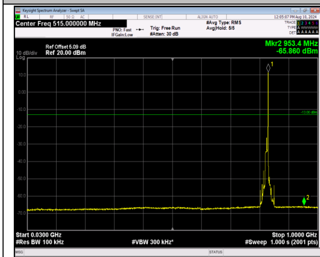
5-5-10MHz-10MHz-QPSK-QPSK-20450-20549-1RB#49-0RB#0-30~1000MHz-PASS
