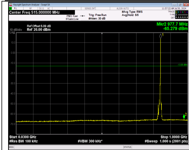
5-5-5MHz-3MHz-64QAM-64QAM-20595-20634-1RB#24-ORB#0-30~1000MHz-PASS
