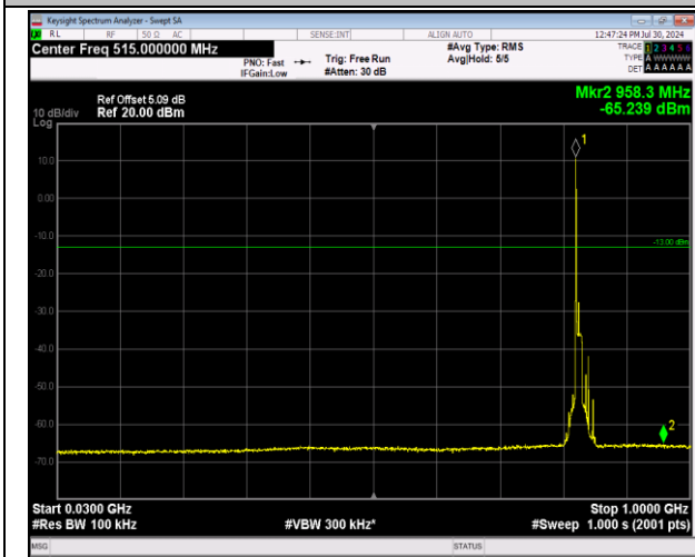
5-5-10MHz-10MHz-64QAM-64QAM-20450-20549-1RB#0 -0RB#0-30~1000MHz-PASS
