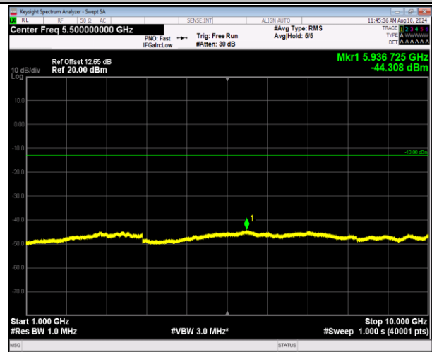
5-5-5MHz-3MHz-QPSK-QPSK-20595-20634-25RB#0-15RB #0-1000~10000MHz-PASS
