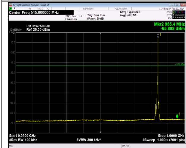
5-5-5MHz-3MHz-16QAM-16QAM-20595-20634-1RB#24- ORB#0-30~1000MHz-PASS
