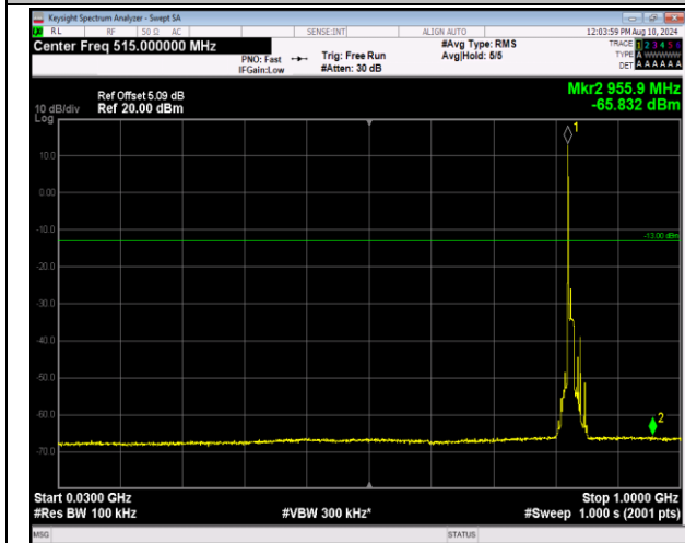
5-5-10MHz-10MHz-QPSK-QPSK-20450-20549-1RB#0-0RB#0-30~1000MHz-PASS
