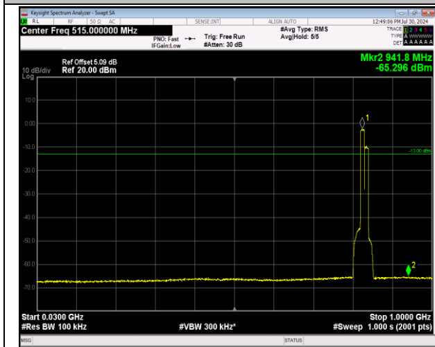
5-5-10MHz-10MHz-64QAM-64QAM-20450-20549-50RB#- 0-50RB#0-30~1000MHz-PASS
