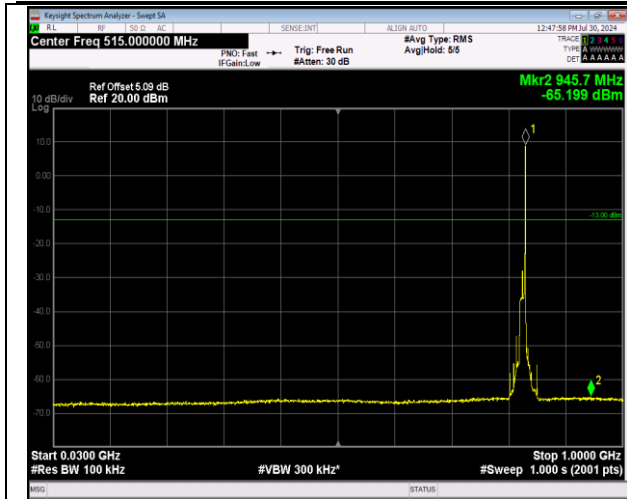
5-5-10MHz-10MHz-64QAM-64QAM-20450-20549-1RB#4 9-0RB#0-30~1000MHz-PASS
