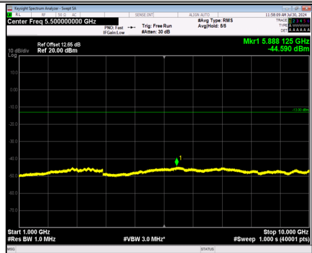
5-5-5MHz-3MHz-64QAM-64QAM-20595-20634-1RB#0-1RB#15-1000~10000MHz-PASS
