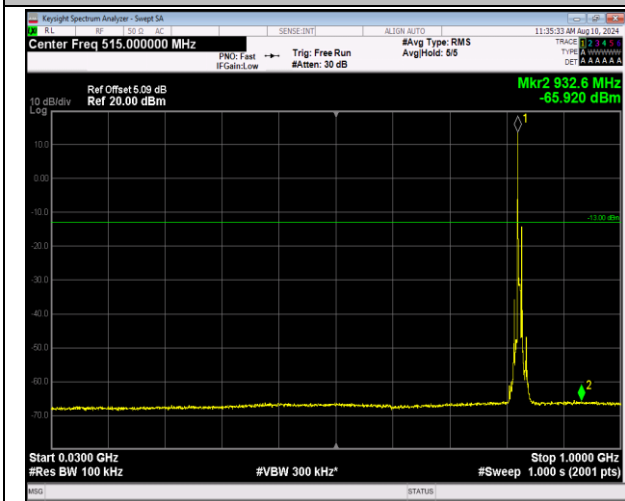
5-5-5MHz-3MHz-16QAM-16QAM-20425-20464-1RB#0-1 RB#15-30~1000MHz-PASS
