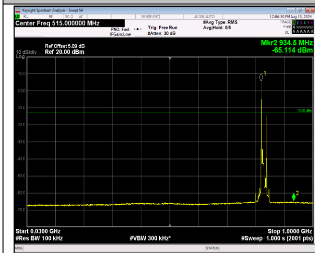
5-5-10MHz-10MHz-16QAM-16QAM-20450-20549-1RB#0 -1RB#49-30~1000MHz-PASS
