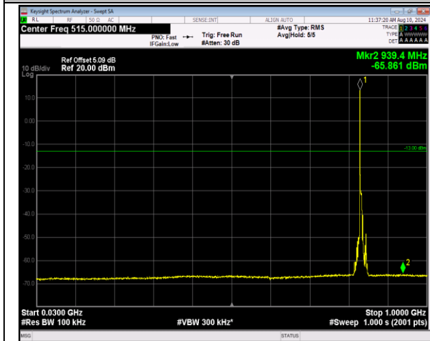
5-5-MHz-3MHz-QPSK-QPSK-20510-20549-1RB#0-0RB#0-30~1000MHz-PASS
