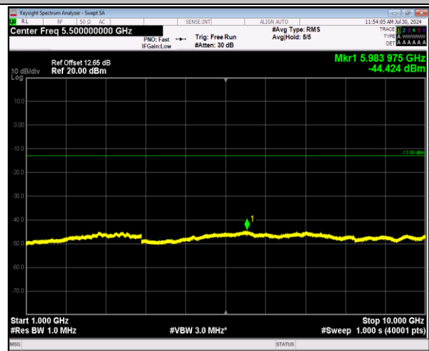
5-5-MHz-3MHz-64QAM-64QAM-20425-20464-25RB#0-15RB#0-1000~10000MHz-PASS
