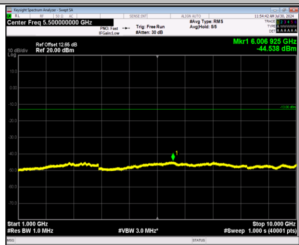
5-5-5MHz-3MHz-64QAM-64QAM-20510-20549-1RB#0-0RB#0-1000~10000MHz-PASS
