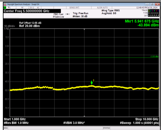
5-5-10MHz-10MHz-64QAM-64QAM-20450-20549-1RB#0-1 RB#49-1000~10000MHz-PASS
