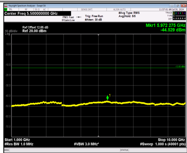
5-5-5MHz-3MHz-64QAM-64QAM-20595-20634-1RB#0-0RB#0-1000~10000MHz-PASS
