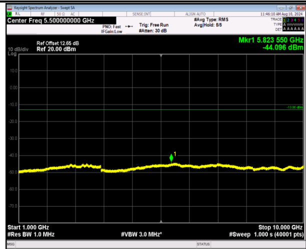
5-5-5MHz-3MHz-16QAM-16QAM-20595-20634-25RB#0-15RB#0-1000~10000MHz-PASS
