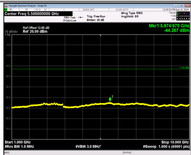
5-5-10MHz-10MHz-16QAM-16QAM-20450-20549-1RB#49- 0RB#0-1000~10000MHz-PASS
