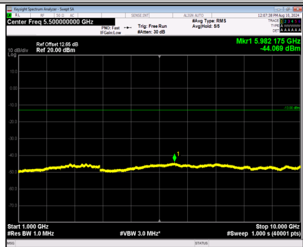
5-5-10MHz-10MHz-QPSK-QPSK-20450-20549-50RB#0-50RB#0-1000~10000MHz-PASS
