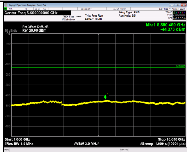
5-5-10MHz-10MHz-QPSK-QPSK-20450-20549-1RB#0-0RB#0-1000~10000MHz-PASS
