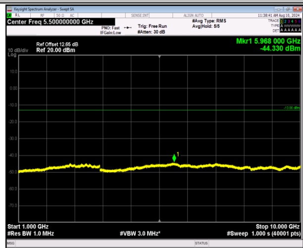
5-5-MHz-3MHz-QPSK-QPSK-20510-20549-1RB#24-0RB# 0-1000~10000MHz-PASS
