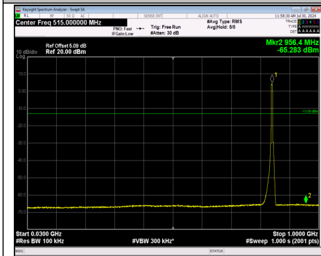
5-5-5MHz-3MHz-64QAM-64QAM-20595-20634-25RB#0-15RB#0-30~1000MHz-PASS
