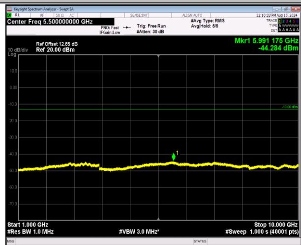
5-5-10MHz-10MHz-16QAM-16QAM-20476-20575-1RB#49- ORB#0-1000~10000MHz-PASS
