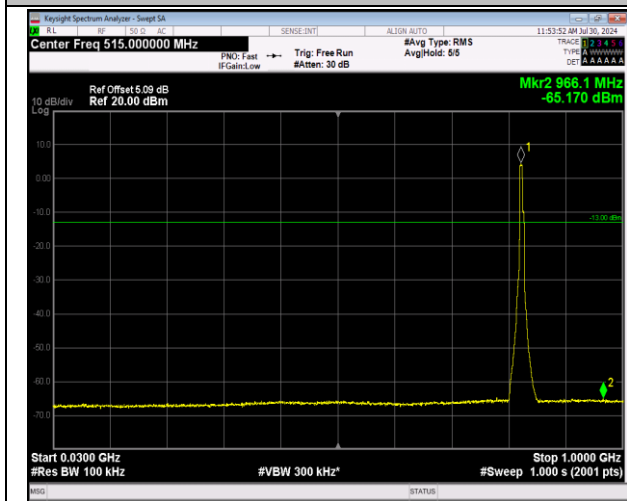
5-5-MHz-3MHz-64QAM-64QAM-20425-20464-25RB#0-15RB#0-30~1000MHz-PASS
