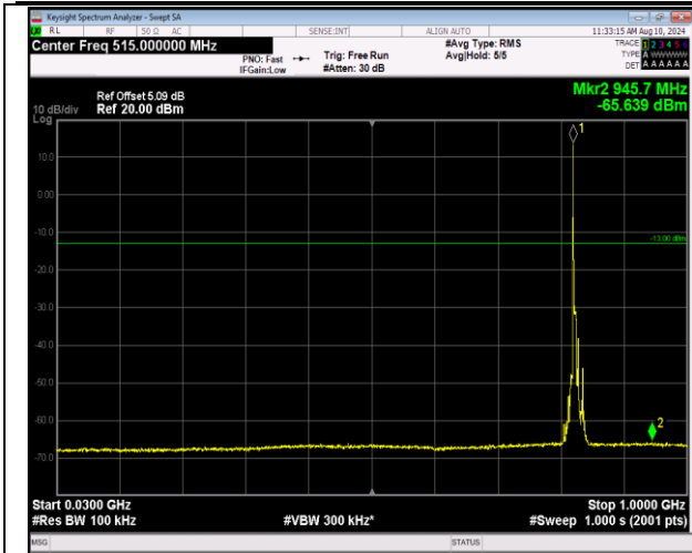
5-5-5MHz-3MHz-16QAM-16QAM-20425-20464-1RB#0-0 RB#0-30~1000MHz-PASS
