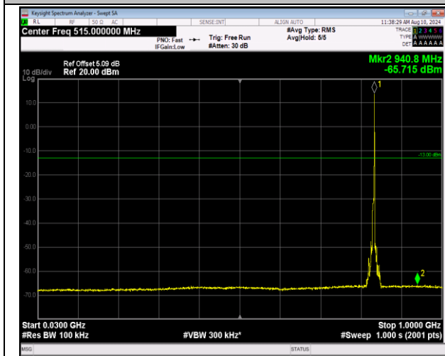
5-5-MHz-3MHz-QPSK-QPSK-20510-20549-1RB#24-0R B#0-30~1000MHz-PASS
