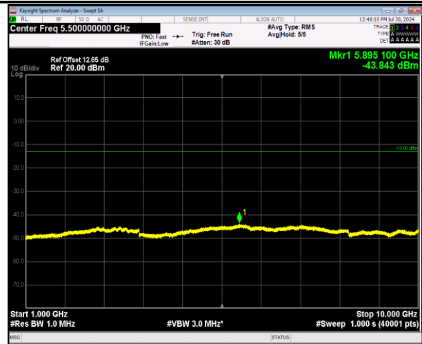
5-5-10MHz-10MHz-64QAM-64QAM-20450-20549-1RB#49- 0RB#0-1000~10000MHz-PASS
