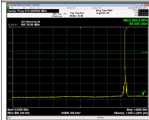
5-5-5MHz-3MHz-64QAM-64QAM-20510-20549-1RB#0-0RB#0-30~1000MHz-PASS
