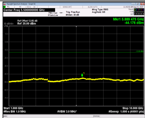
5-5-5MHz-3MHz-16QAM-16QAM-20595-20634-1RB#24-0R B#0-1000~10000MHz-PASS
