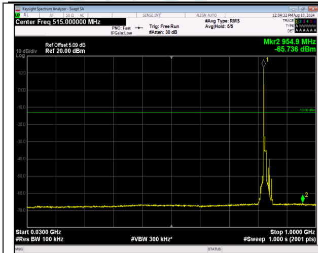
5-5-10MHz-10MHz-16QAM-16QAM-20450-20549-1RB#0 -0RB#0-30~1000MHz-PASS
