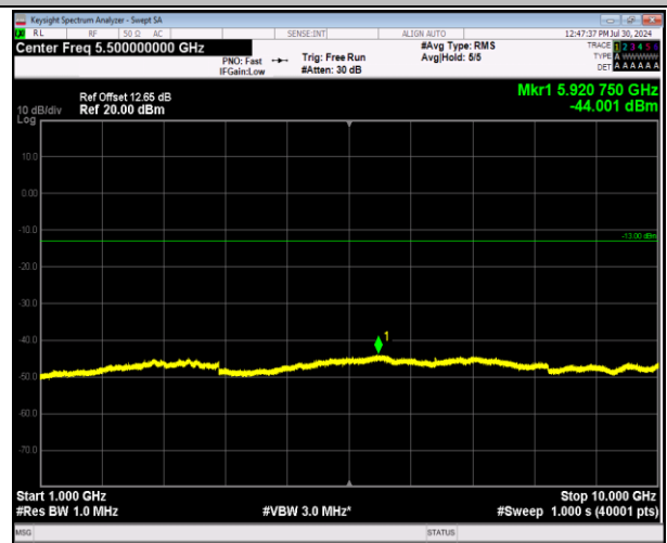
5-5-10MHz-10MHz-64QAM-64QAM-20450-20549-1RB#0-0 RB#0-1000~10000MHz-PASS
