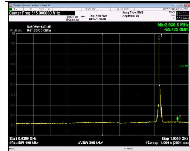
5-5-MHz-3MHz-QPSK-QPSK-20510-20549-1RB#0-1RB #15-30~1000MHz-PASS
