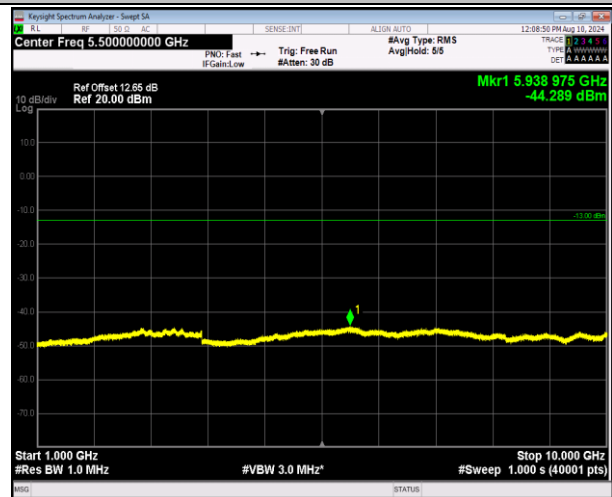
5-5-10MHz-10MHz-QPSK-QPSK-20476-20575-1RB#0-0RB #0-1000~10000MHz-PASS
