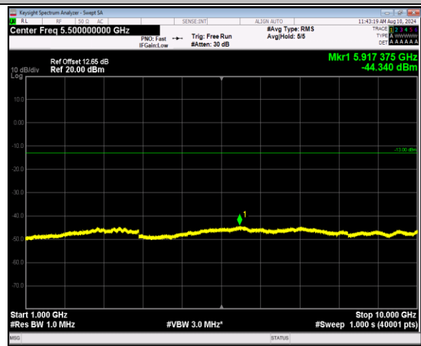
5-5-5MHz-3MHz-QPSK-QPSK-20595-20634-1RB#24-0RB# 0-1000~10000MHz-PASS
