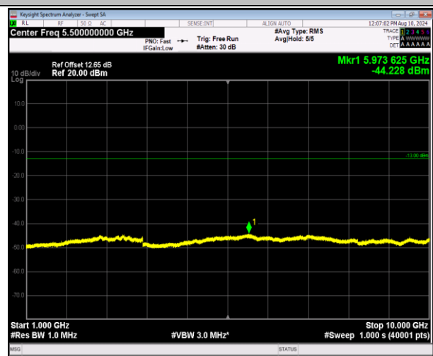
5-5-10MHz-10MHz-16QAM-16QAM-20450-20549-1RB#0-1 RB#49-1000~10000MHz-PASS
