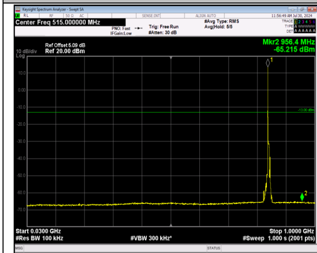
5-5-5MHz-3MHz-64QAM-64QAM-20595-20634-1RB#0-0RB#0-30~1000MHz-PASS
