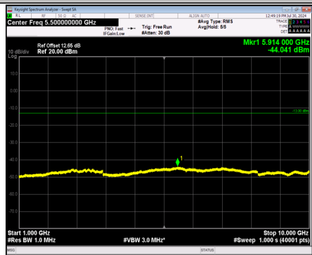
5-5-10MHz-10MHz-64QAM-64QAM-20450-20549-50RB#0- 50RB#0-1000~10000MHz-PASS
