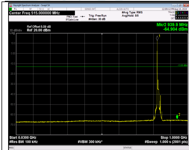
5-5-10MHz-10MHz-16QAM-16QAM-20476-20575-1RB#0 -ORB#0-30~1000MHz-PASS
