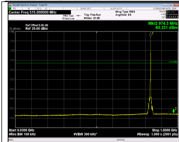
5-5-5MHz-3MHz-64QAM-64QAM-20510-20549-1RB#24- ORB#0-30~1000MHz-PASS
