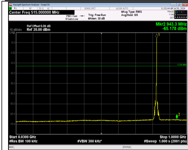
5-5-MHz-3MHz-64QAM-64QAM-20425-20464-1RB#24-ORB#0-30~1000MHz-PASS
