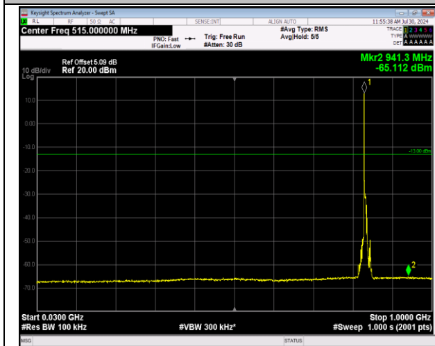
5-5-5MHz-3MHz-64QAM-64QAM-20510-20549-1RB#0-1RB#15-30~1000MHz-PASS
