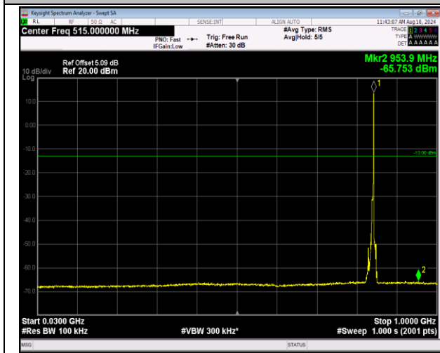
5-5-5MHz-3MHz-QPSK-QPSK-20595-20634-1RB#24-0RB B#0-30~1000MHz-PASS
