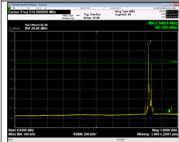
5-5-10MHz-10MHz-64QAM-64QAM-20450-20549-1RB#0 -1RB#49-30~1000MHz-PASS
