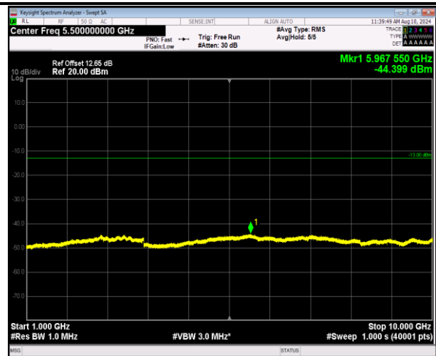
5-5-MHz-3MHz-QPSK-QPSK-20510-20549-1RB#0-1RB#1 5-1000~10000MHz-PASS
