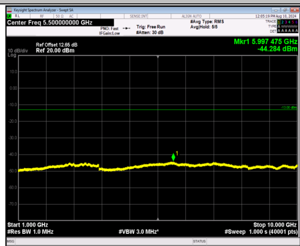
5-5-10MHz-10MHz-QPSK-QPSK-20450-20549-1RB#49-0RB#0-1000~10000MHz-PASS
