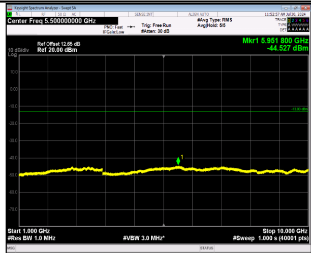
5-5-MHz-3MHz-64QAM-64QAM-20425-20464-1RB#24-ORB#0-1000~10000MHz-PASS
