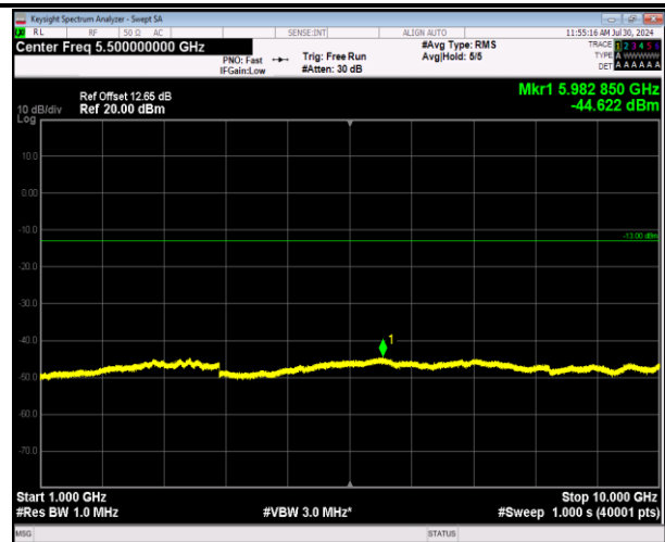
5-5-5MHz-3MHz-64QAM-64QAM-20510-20549-1RB#24-0R B#0-1000~10000MHz-PASS
