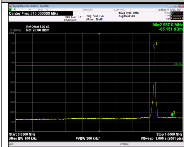
5-5-5MHz-3MHz-64QAM-64QAM-20510-20549-25RB#0- 15RB#0-30~1000MHz-PASS
