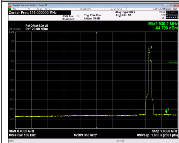
5-5-10MHz-10MHz-QPSK-QPSK-20450-20549-50RB#0-050RB#0-30~1000MHz-PASS
