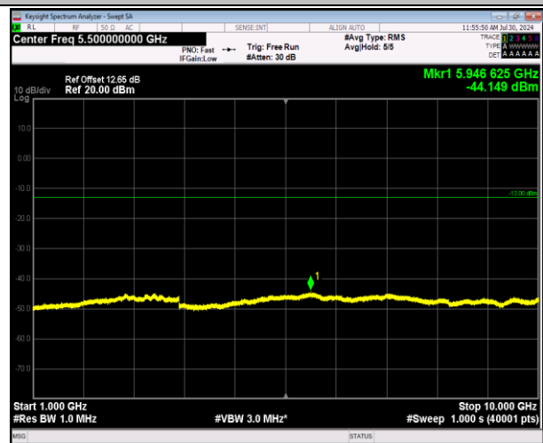
5-5-5MHz-3MHz-64QAM-64QAM-20510-20549-1RB#0-1RB#15-1000~10000MHz-PASS
