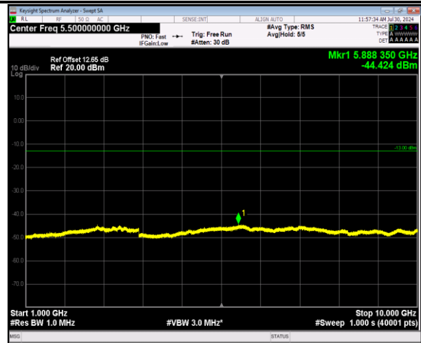
5-5-5MHz-3MHz-64QAM-64QAM-20595-20634-1RB#24-ORB#0-1000~10000MHz-PASS
