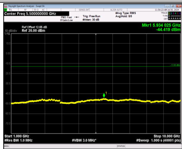
5-5-5MHz-3MHz-64QAM-64QAM-20510-20549-25RB#0-15 RB#0-1000~10000MHz-PASS
