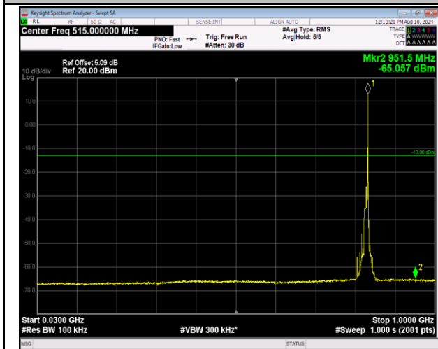
5-5-10MHz-10MHz-16QAM-16QAM-20476-20575-1RB#4 9-ORB#0-30~1000MHz-PASS
