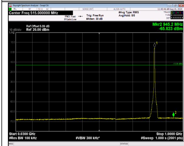
5-5-MHz-3MHz-QPSK-QPSK-20510-20549-25RB#0-15 RB#0-30~1000MHz-PASS
