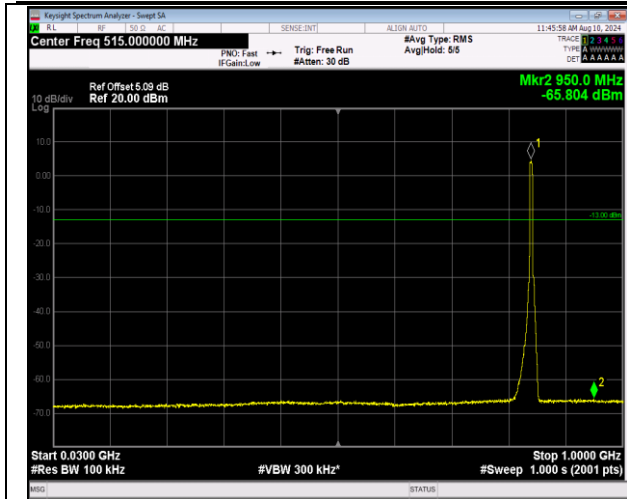
5-5-5MHz-3MHz-16QAM-16QAM-20595-20634-25RB#0-0-15RB#0-30~1000MHz-PASS
