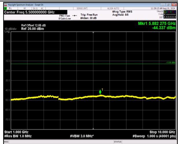
5-5-5MHz-3MHz-16QAM-16QAM-20510-20549-1RB#24-OR B#0-1000~10000MHz-PASS
