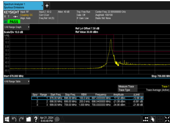
N71(20M)_DFT-s- OFDM_BPSK_Edge_1RB_Right_High_CH
