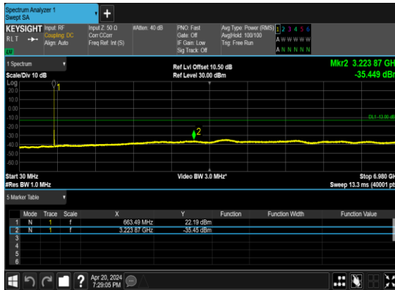
N71(5M)_CP- OFDM_QPSK_Edge_1RB_Left_Low_CH
