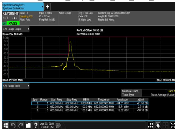
N71(10M)_CP- OFDM_QPSK_Edge_1RB_Left_Low_CH
