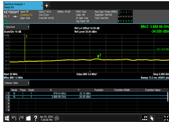
N71(5M)_CP- OFDM_QPSK_Edge_1RB_Left_Mid_CH
