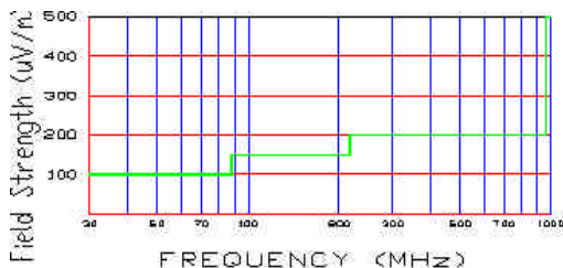
Figure A-7. Radiated limits at 3 meters.
