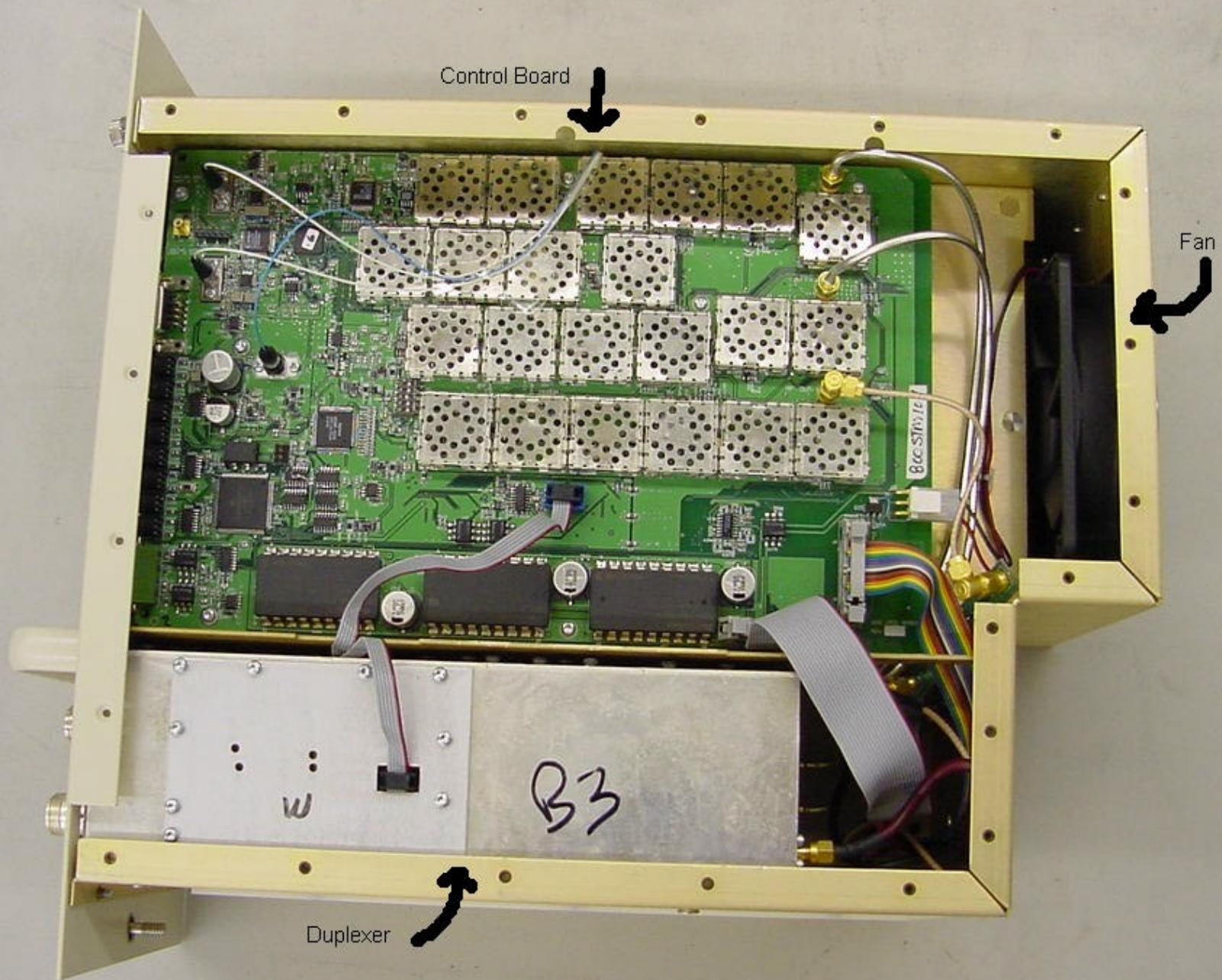
Digivance 800 MHz LRCS Signal Transport Module Right View - Open
