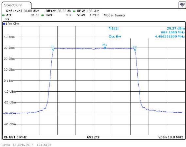
Figure 27 Occupied Bandwidth – 64QAM (881.5 MHz) (5 MHz Channel BW)
