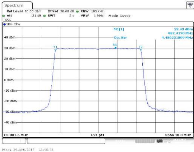
Figure 24 Occupied Bandwidth – 256QAM (881.5 MHz) (5 MHz Channel BW)
