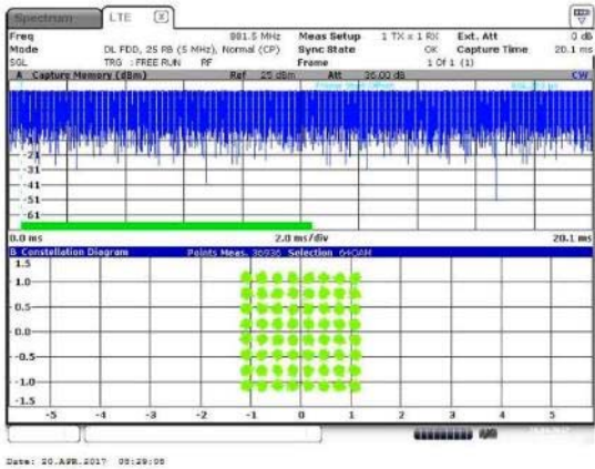
Figure 9 I/Q constellation diagram with capture buffer – 64QAM (881.5 MHz) (5 MHz Channel BW)
