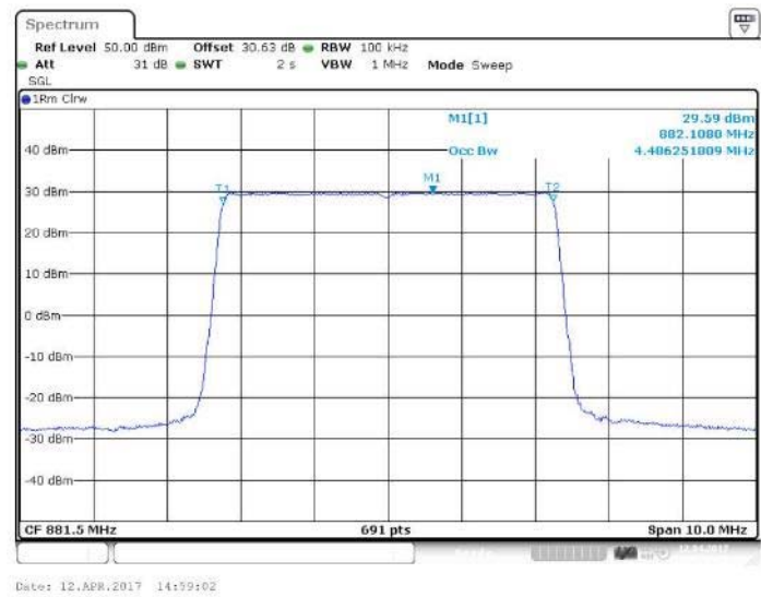
Figure 15 Occupied Bandwidth – 64QAM (881.5 MHz) (5 MHz Channel BW)
