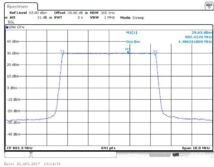
Figure 16 Occupied Bandwidth – 256QAM (881.5 MHz) (5 MHz Channel BW)
