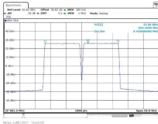
Figure 32 Occupied Bandwidth – 256QAM (879 MHz, 884 MHz) (2 X 5 MHz Channel BW)
