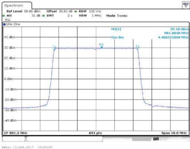
Figure 23 Occupied Bandwidth – 64QAM (881.5 MHz) (5 MHz Channel BW)
