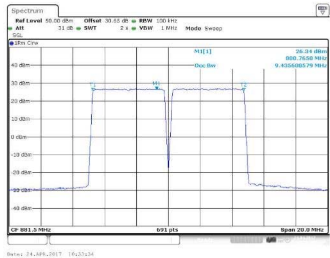
Figure 31 Occupied Bandwidth – 64QAM (879 MHz, 884 MHz) (2 X 5 MHz Channel BW)
