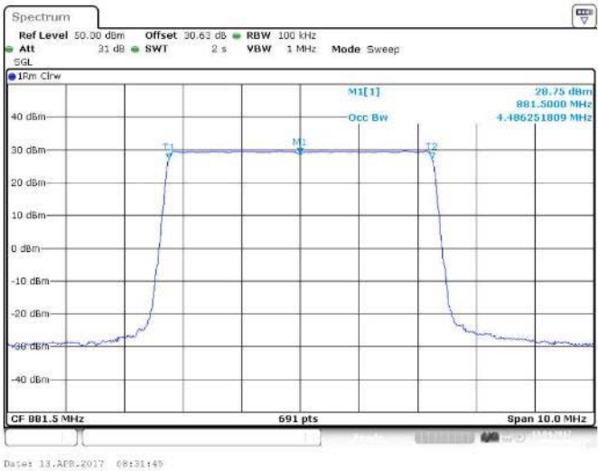
Figure 17 Occupied Bandwidth – QPSK (881.5 MHz) (5 MHz Channel BW)
