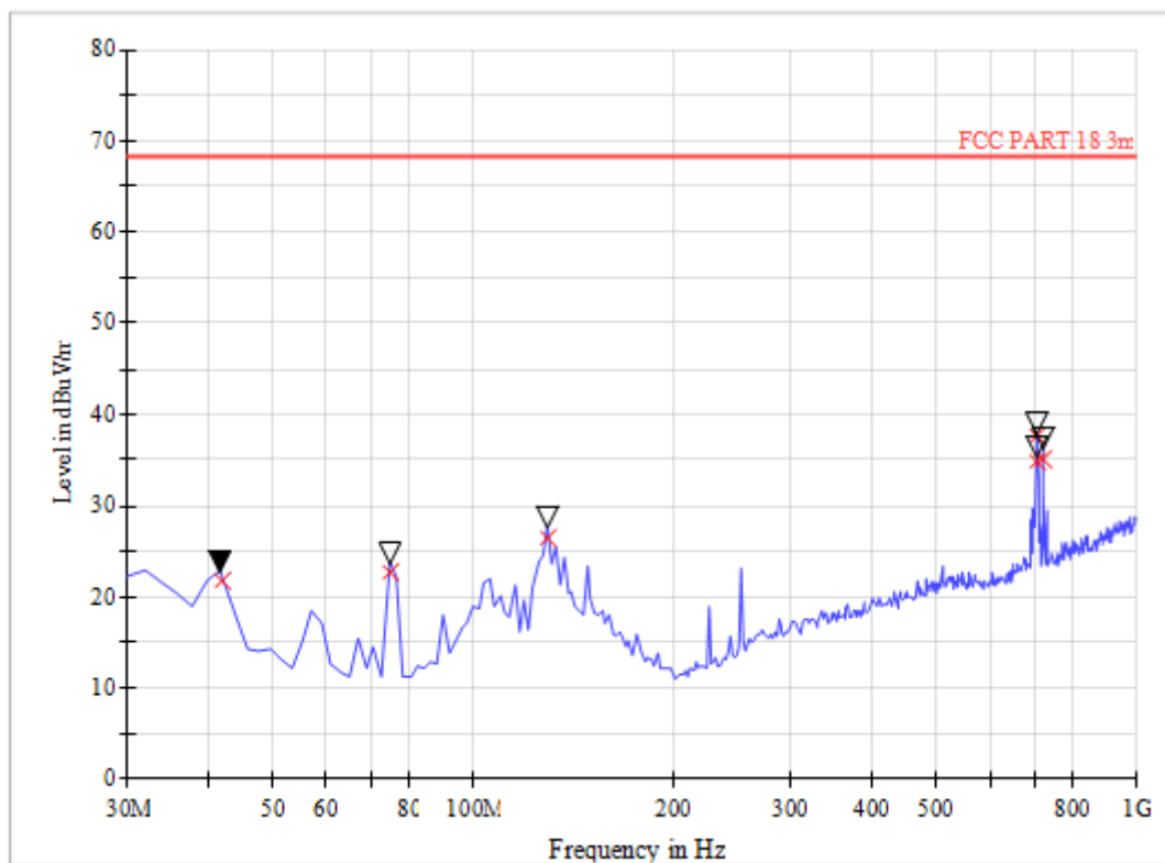
(Plot B: Test Antenna Vertical 30M - 1G)
