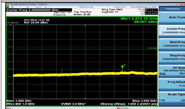
Band5_3MHz_16QAM_20525_1RB#14_1000~3000_1000~3000
