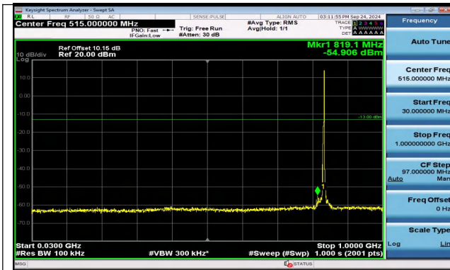
Band5_3MHz_QPSK_20525_1RB#14_30~1000_30~1000
