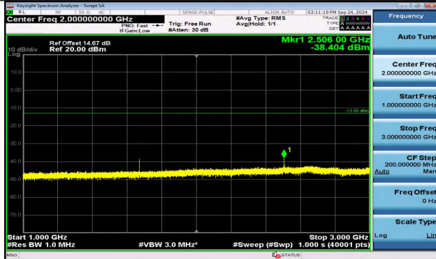
Band5_3MHz_16QAM_20525_1RB#0_1000~3000_1000~3000
