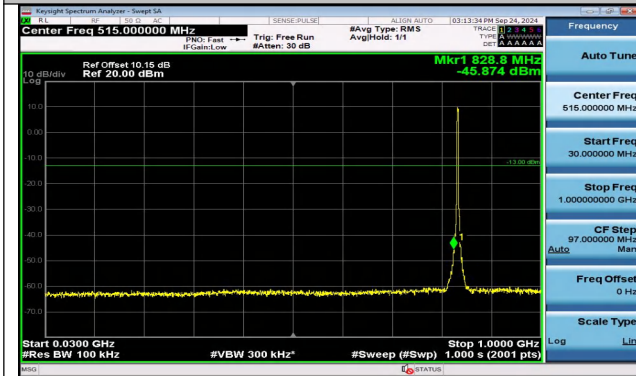
Band5_3MHz_QPSK_20525_15RB#0_30~1000_30~1000
