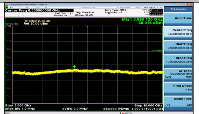
Band5_3MHz_16QAM_20525_1RB#14_3000~10000_3000~10000
