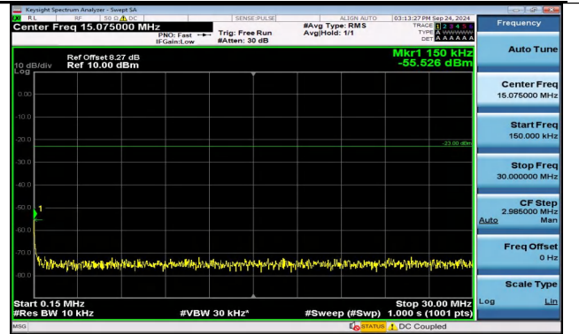
Band5_3MHz_QPSK_20525_15RB#0_0.15~30_0.15~30
