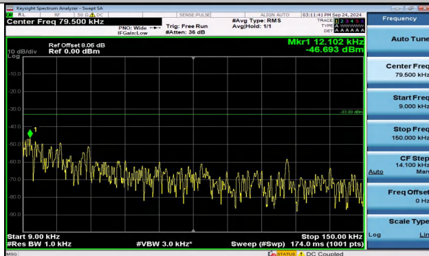
Band5_3MHz_QPSK_20525_1RB#14_0.009~0.15_0.009~0.15
