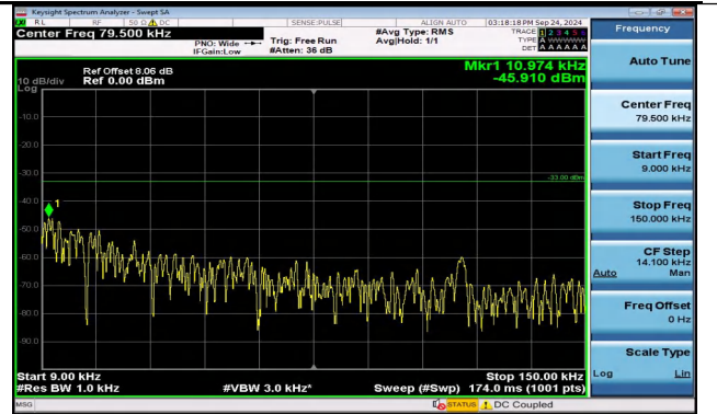
Band5_3MHz_16QAM_20635_1RB#14_0.009~0.15_0.009 ~0.15
