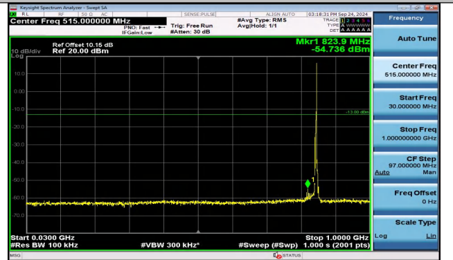
Band5_3MHz_16QAM_20635_1RB#14_30~1000_30~100 0
