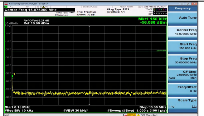
Band5_3MHz_QPSK_20525_1RB#14_0.15~30_0.15~30
