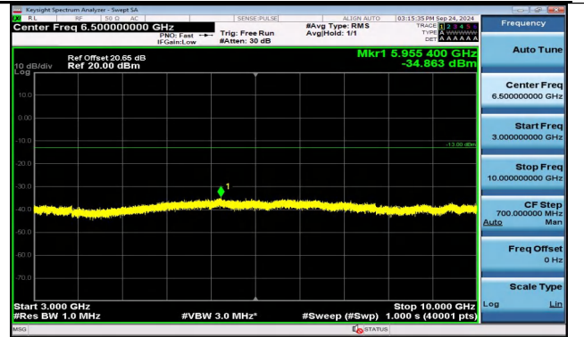
Band5_3MHz_16QAM_20525_15RB#0_3000~10000_3000 ~10000
