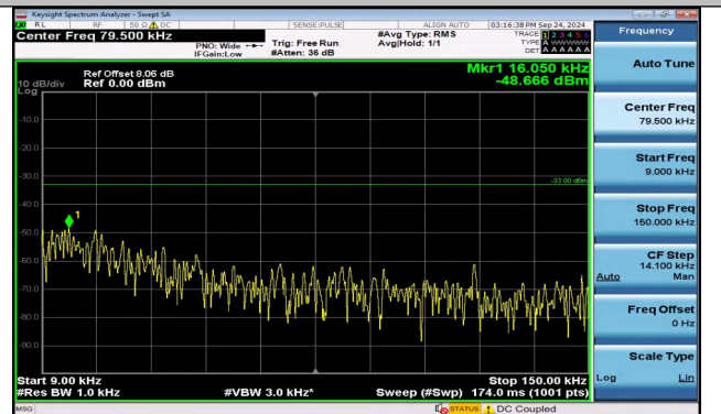
Band5_3MHz_16QAM_20635_1RB#0_0.009~0.15_0.009~0.15
