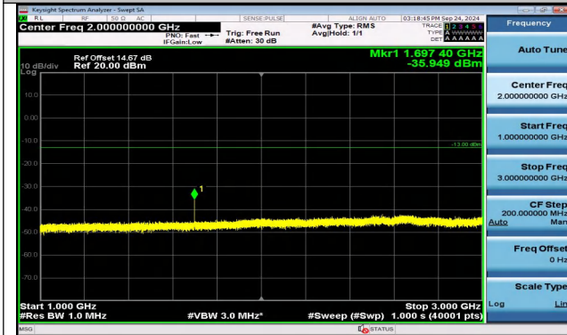
Band5_3MHz_16QAM_20635_1RB#14_1000~3000_1000 ~3000
