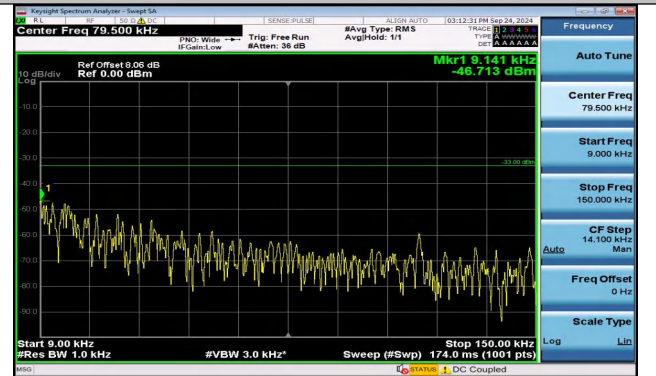
Band5_3MHz_16QAM_20525_1RB#14_0.009~0.15_0.009~0.15
