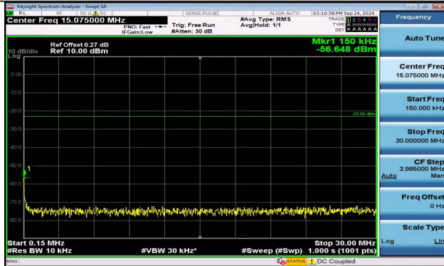
Band5_3MHz_16QAM_20525_1RB#0_0.15~30_0.15~30
