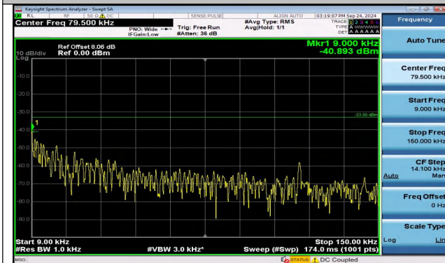
Band5_3MHz_QPSK_20635_15RB#0_0.009~0.15_0.009 ~0.15
