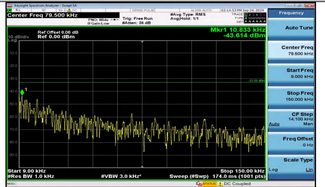
Band5_3MHz_16QAM_20525_15RB#0_0.009~0.15_0.009~0.15
