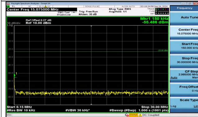
Band5_3MHz_16QAM_20635_1RB#14_0.15~30_0.15~3 0
