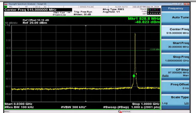
Band5_3MHz_16QAM_20525_15RB#0_30~1000_30~1000
