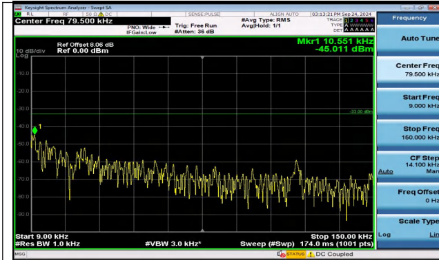
Band5_3MHz_QPSK_20525_15RB#0_0.009~0.15_0.009~0.15
