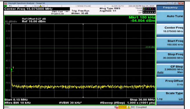
Band5_3MHz_QPSK_20635_1RB#0_0.15~30_0.15~30
