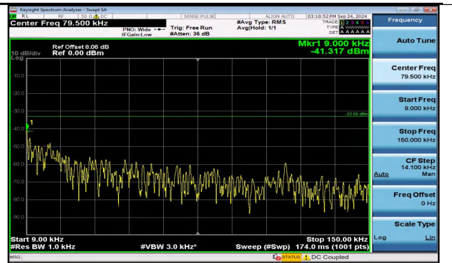
Band5_3MHz_16QAM_20525_1RB#0_0.009~0.15_0.009~0.15
