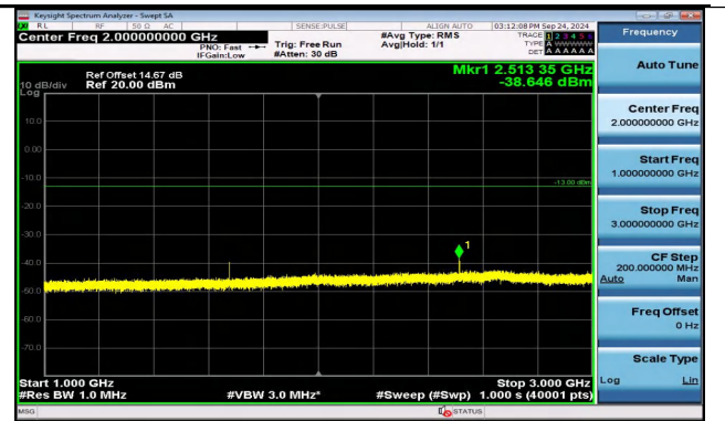
Band5_3MHz_QPSK_20525_1RB#14_1000~3000_1000~3000
