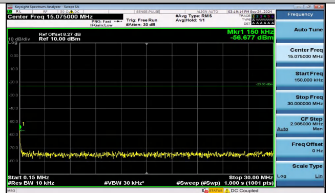
Band5_3MHz_QPSK_20635_15RB#0_0.15~30_0.15~30
