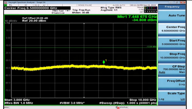
Band5_3MHz_16QAM_20525_1RB#0_3000~10000_3000~10000
