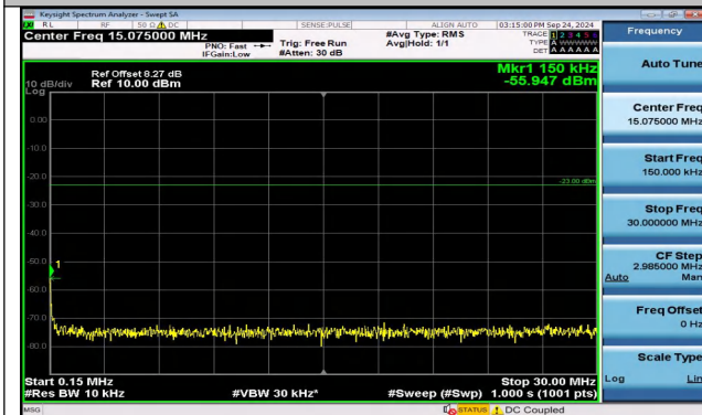
Band5_3MHz_16QAM_20525_15RB#0_0.15~30_0.15~30
