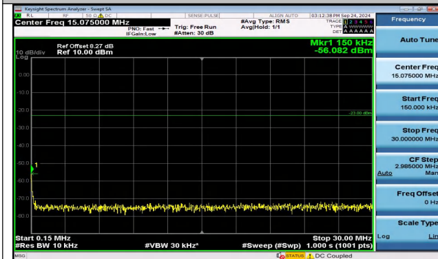
Band5_3MHz_16QAM_20525_1RB#14_0.15~30_0.15~30
