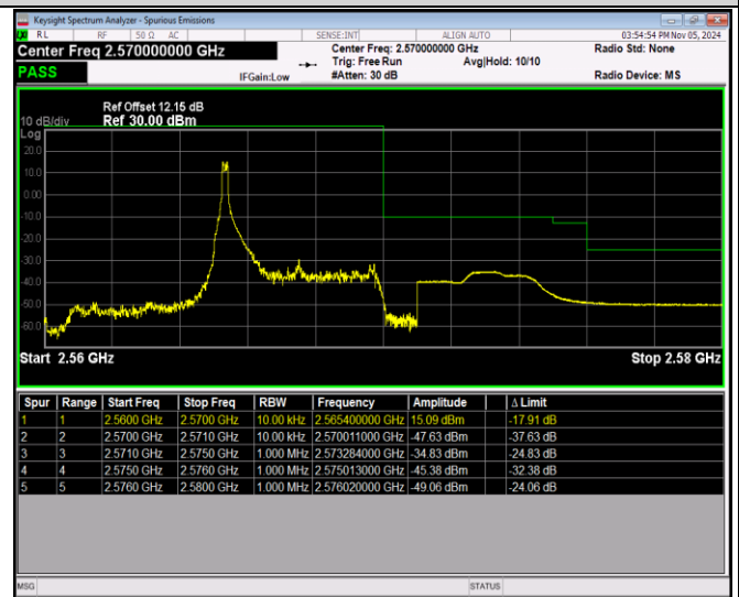
Band7-5MHz-QPSK-21425-25RB#0
