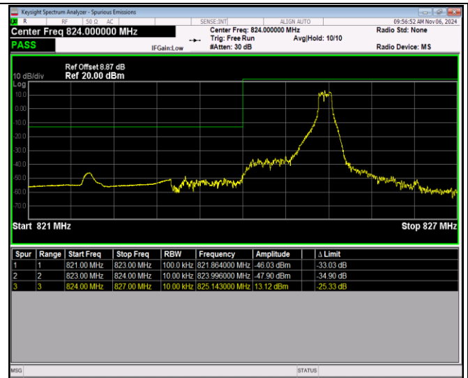
Band5-1.4MHz-64QAM-20643-1RB#0
