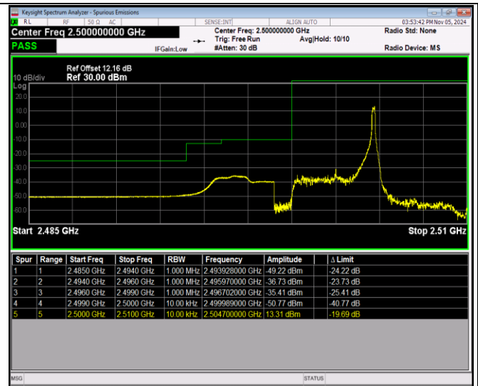
Band7-5MHz-16QAM-21425-1RB#0
