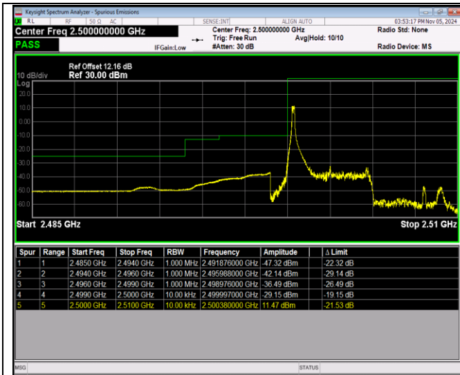
Band7-5MHz-64QAM-20775-25RB#0
