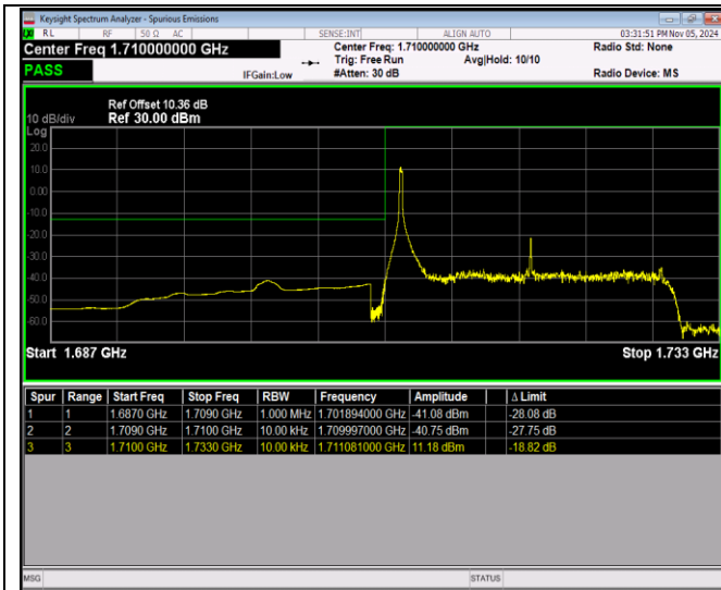
Band4-20MHz-16QAM-20050-100RB#0
