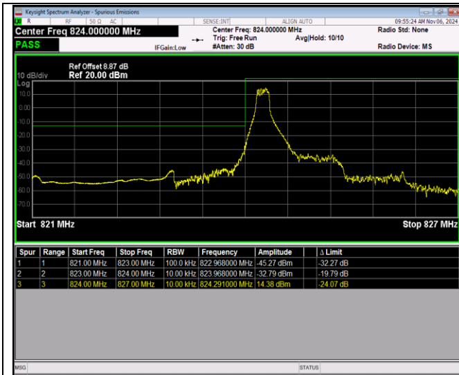
Band5-1.4MHz-QPSK-20407-6RB#0
