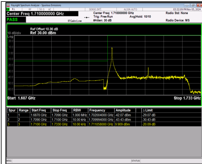
Band4-20MHz-64QAM-20050-100RB#0
