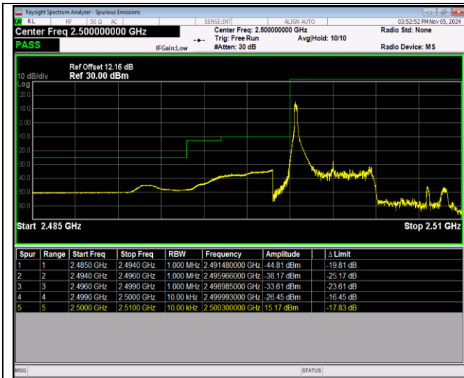
Band7-5MHz-QPSK-20775-25RB#0
