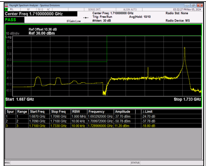
Band4-20MHz-QPSK-20300-1RB#0
