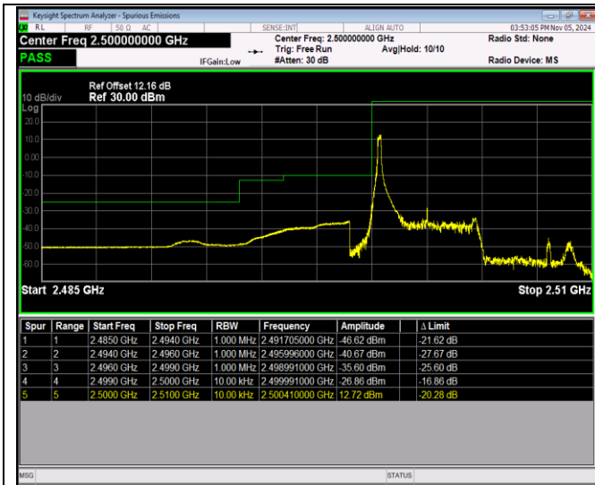
Band7-5MHz-16QAM-20775-25RB#0
