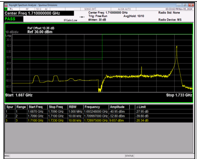
Band4-20MHz-64QAM-20300-1RB#0
