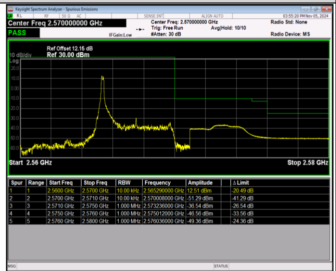
Band7-5MHz-64QAM-21425-25RB#0
