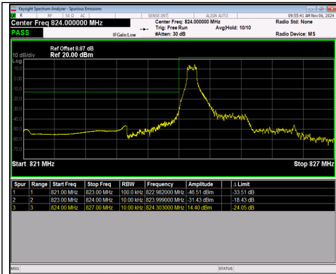
Band5-1.4MHz-16QAM-20407-6RB#0
