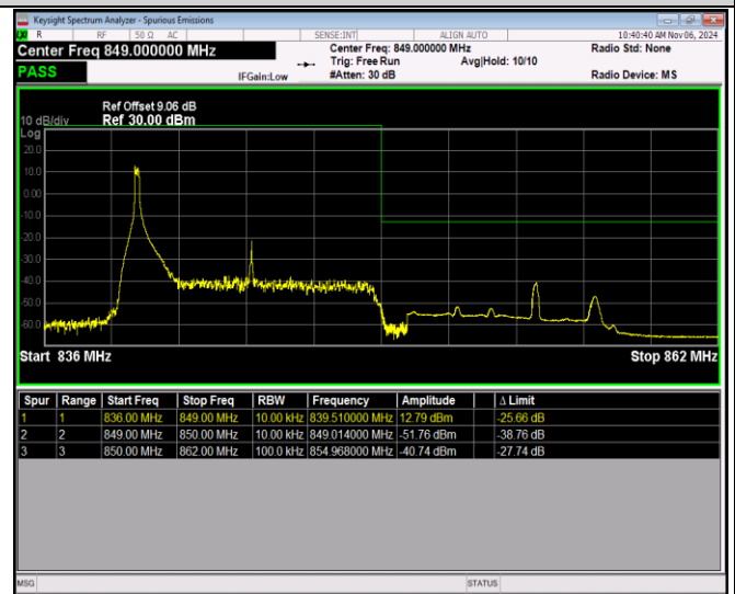
Band5-10MHz-16QAM-20600-50RB#0
