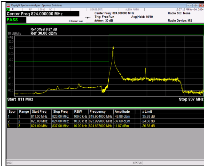
Band5-10MHz-64QAM-20450-50RB#0
