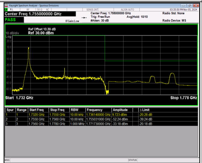
Band4-20MHz-64QAM-20300-100RB#0
