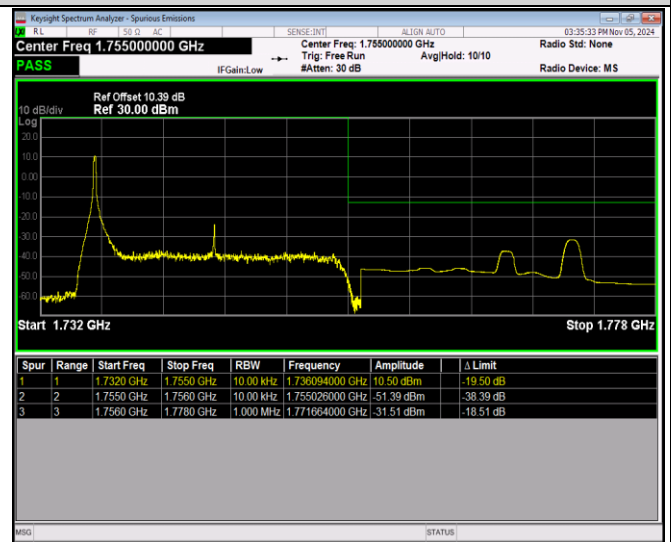
Band4-20MHz-16QAM-20300-100RB#0
