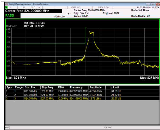
Band5-1.4MHz-64QAM-20407-6RB#0
