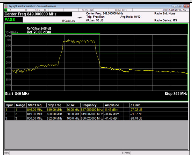
Band5-1.4MHz-16QAM-20407-1RB#5
