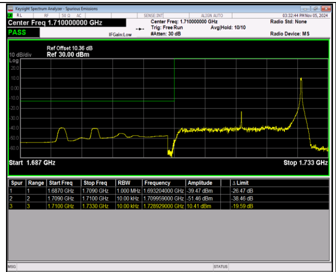
Band4-20MHz-16QAM-20300-1RB#0
