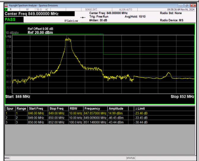
Band5-1.4MHz-QPSK-20643-6RB#0
