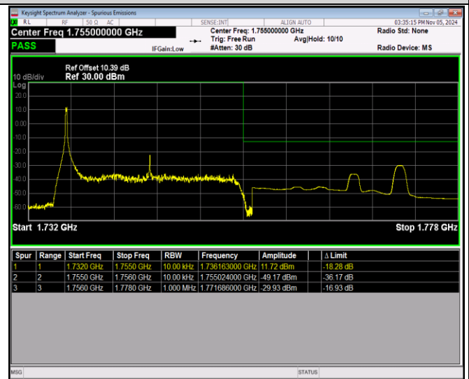
Band4-20MHz-QPSK-20300-100RB#0
