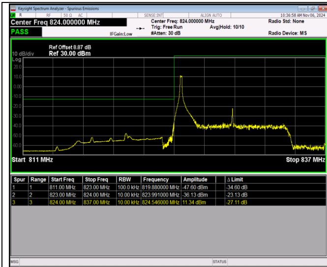
Band5-10MHz-16QAM-20450-50RB#0
