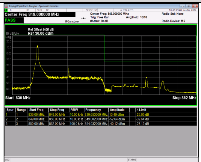
Band5-10MHz-QPSK-20600-50RB#0
