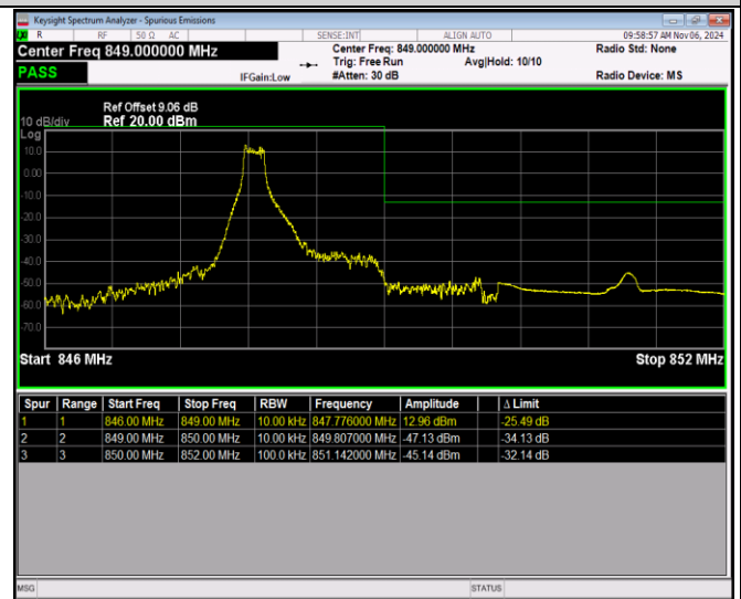
Band5-1.4MHz-16QAM-20643-6RB#0
