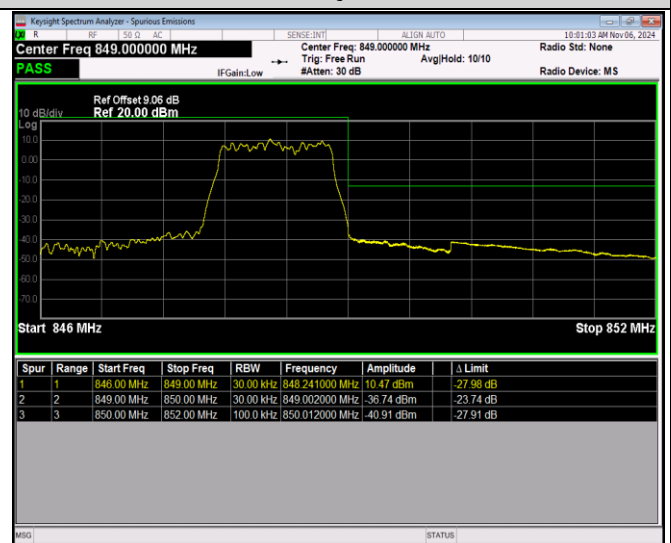
Band5-1.4MHz-64QAM-20407-1RB#5
