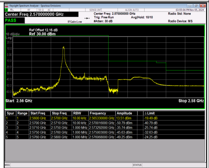
Band7-5MHz-16QAM-21425-25RB#0
