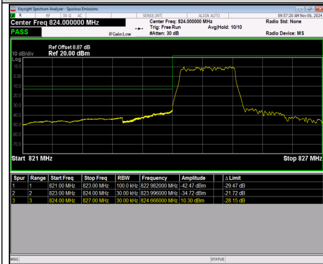
Band5-1.4MHz-QPSK-20643-1RB#5
