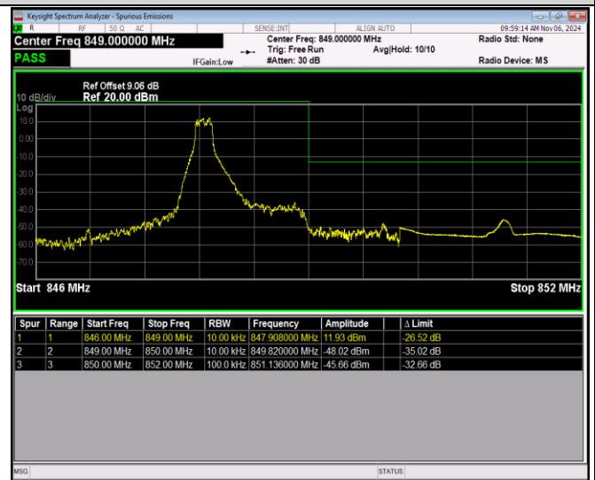
Band5-1.4MHz-64QAM-20643-6RB#0
