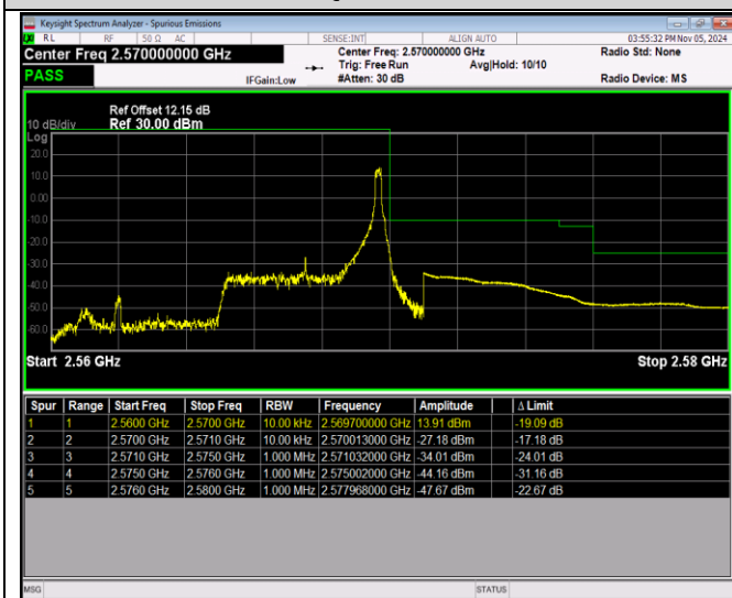
Band7-5MHz-16QAM-20775-1RB#0
