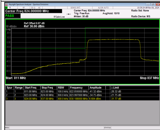
Band5-10MHz-16QAM-20600-1RB#49
