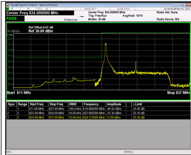
Band5-10MHz-QPSK-20450-50RB#0
